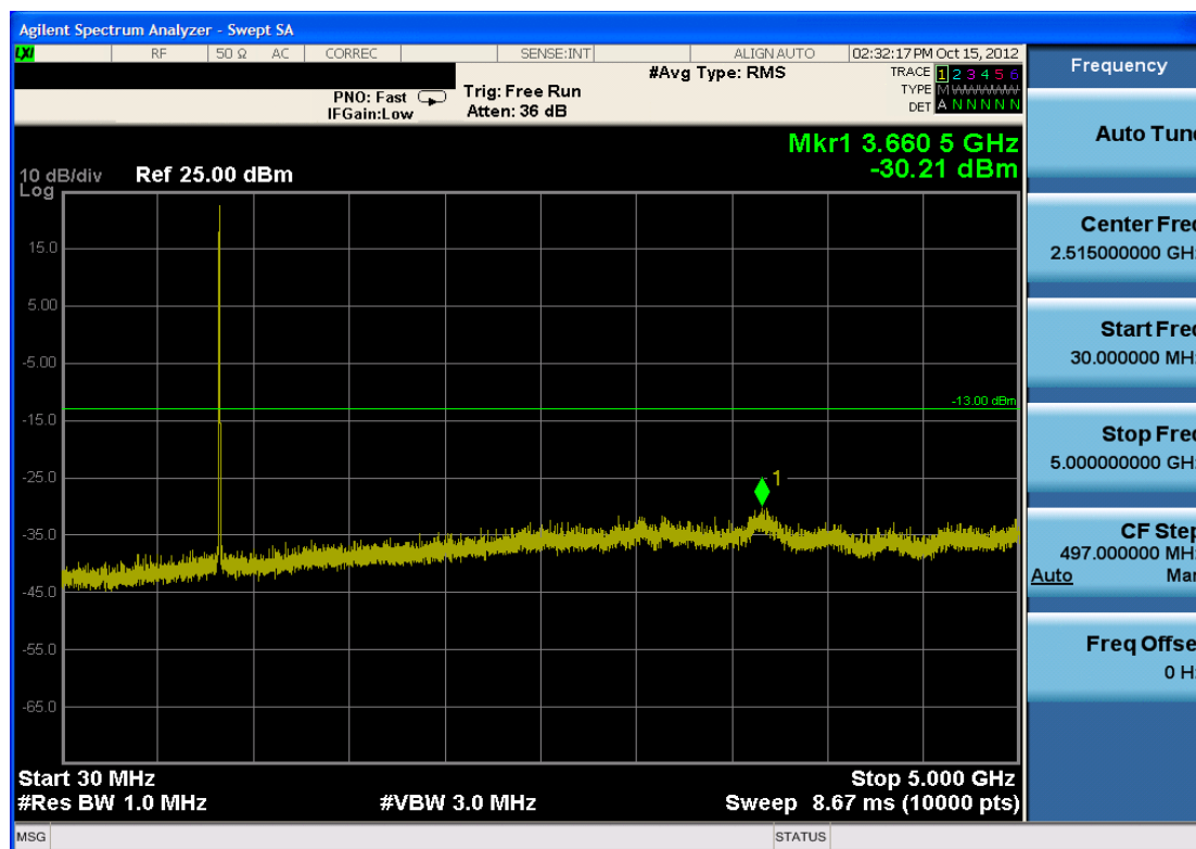
Plot 7-17. Conducted Spurious Plot (Cellular WCDMA Mode – Ch. 4233)
