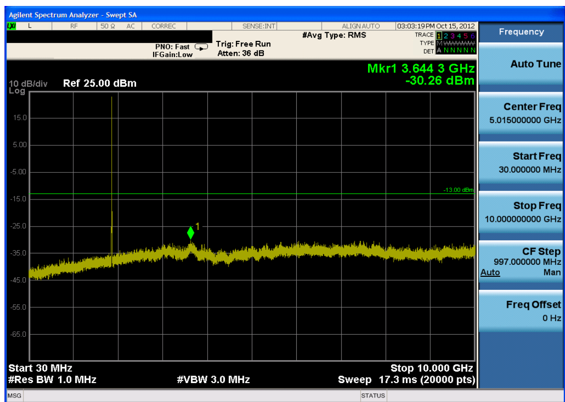
Plot 7-24. Conducted Spurious Plot (PCS WCDMA Mode – Ch. 9400)
