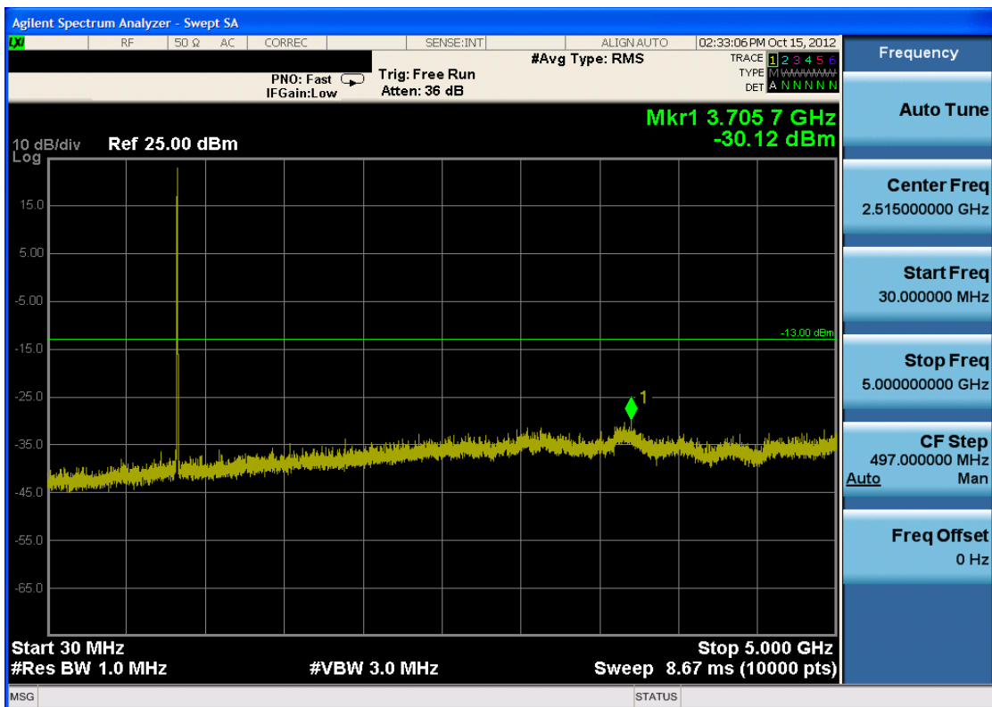
Plot 7-14. Conducted Spurious Plot (Cellular WCDMA Mode – Ch. 4183)
