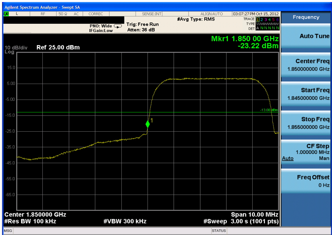
Plot 7-22. Band Edge Plot (PCS WCDMA Mode – Ch. 9262)
