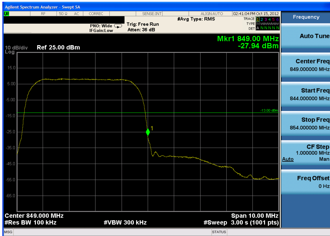
Plot 7-19. Band Edge Plot (Cellular WCDMA Mode – Ch. 4233)
