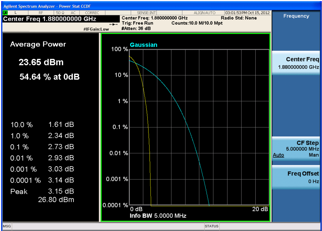
Plot 7-27. Peak-Average Ratio Plot (PCS WCDMA Mode – Ch. 9400)
