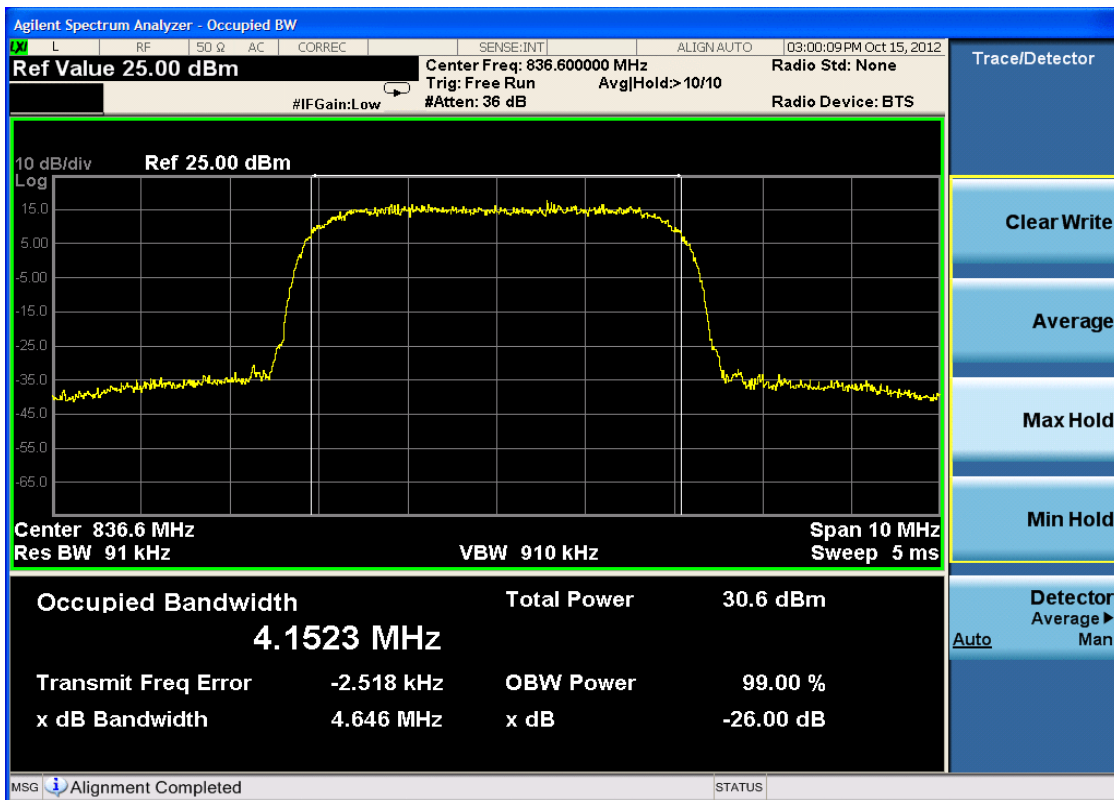
Plot 7-16. Occupied Bandwidth Plot (Cellular WCDMA Mode – Ch. 4183)
