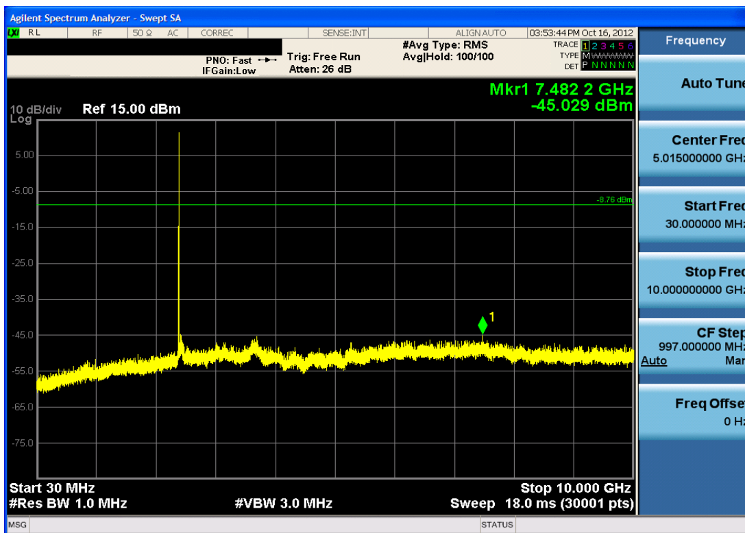
Plot 6-27. Conducted Spurious Plot (Bluetooth, 1Mbps – Ch. 0)
