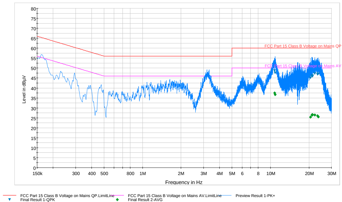
Plot 6-34. Line-Conducted Test Plot (N)
