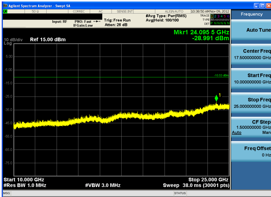
Plot 6-32. Conducted Spurious Plot (Bluetooth, 1Mbps – Ch. 78)
