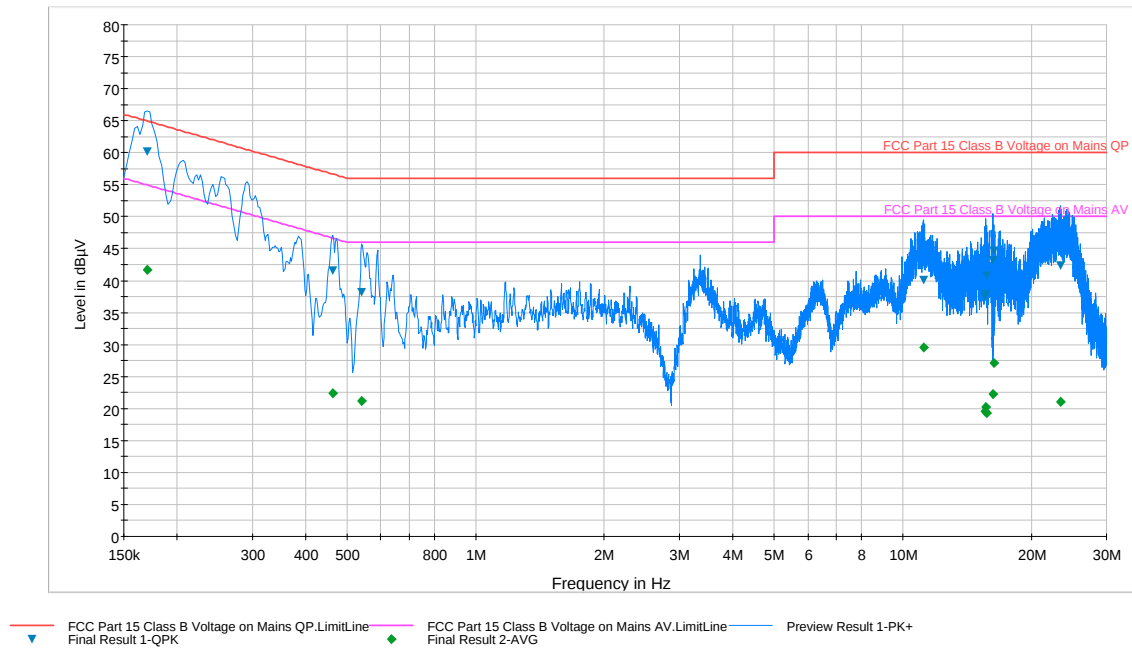
Plot 6-33. Line-Conducted Test Plot (L1)
