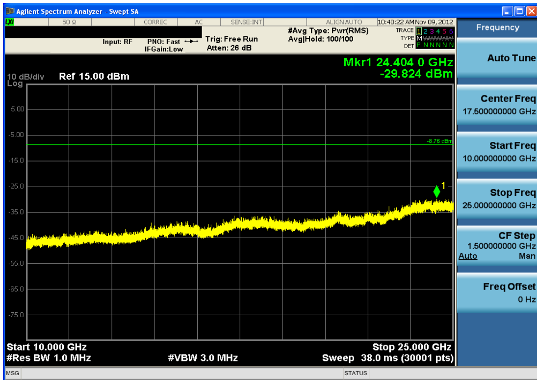
Plot 6-28. Conducted Spurious Plot (Bluetooth, 1Mbps – Ch. 0)
