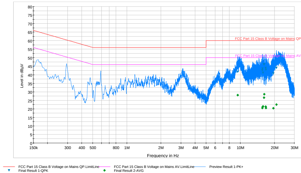
Plot 6-57. Line Conducted Plot with 802.11a UNII Band 1 (L1)
