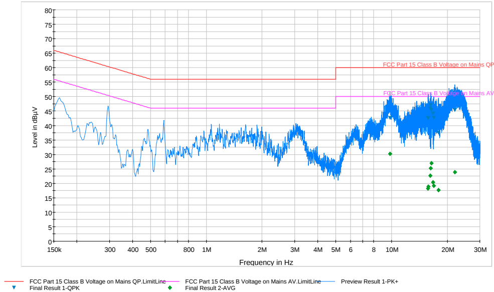
Plot 6-61. Line Conducted Plot with 802.11a UNII Band 3 (L1)
