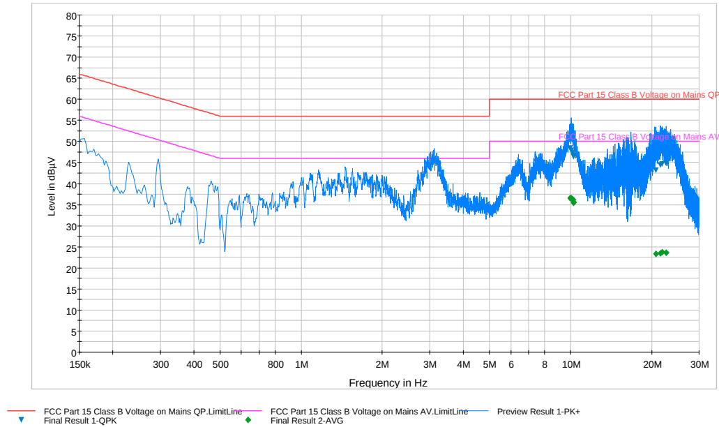
Plot 6-58. Line Conducted Plot with 802.11a UNII Band 1 (N)
