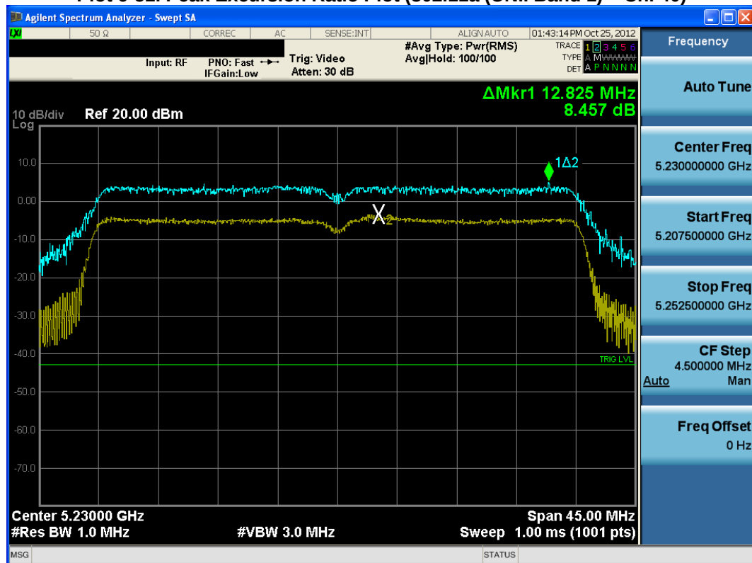
Plot 6-52. Peak Excursion Ratio Plot (40MHz BW 802.11n (UNII Band 1) – Ch. 46)
