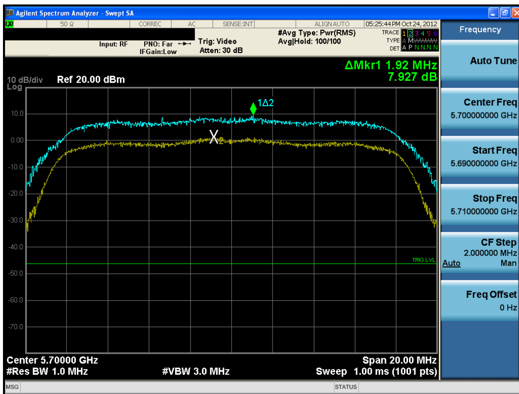
Plot 6-55. Peak Excursion Ratio Plot (802.11a (UNII Band 3) – Ch. 140)
