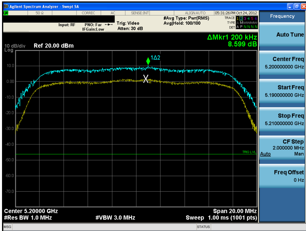
Plot 6-51. Peak Excursion Ratio Plot (802.11a (UNII Band 1) – Ch. 40)
