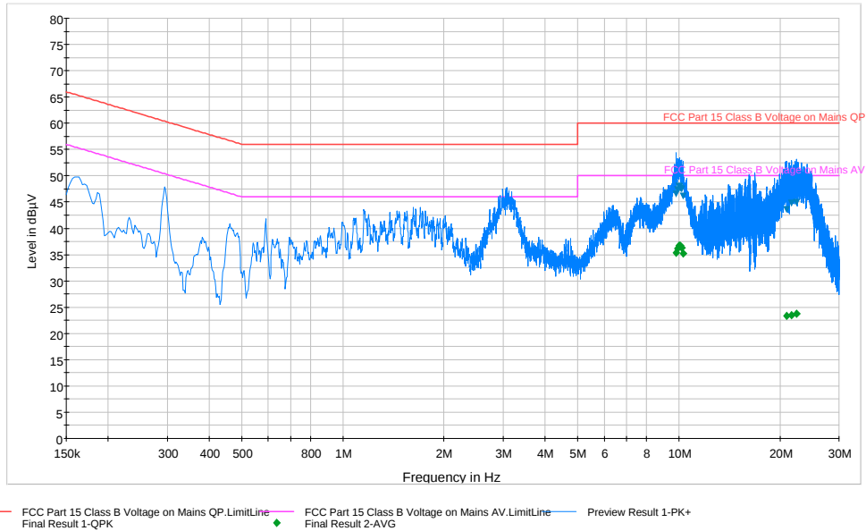
Plot 6-60. Line Conducted Plot with 802.11a UNII Band 2 (N)
