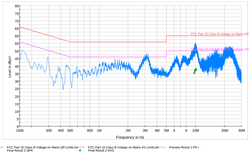
Plot 6-62. Line Conducted Plot with 802.11a UNII Band 3 (N)
