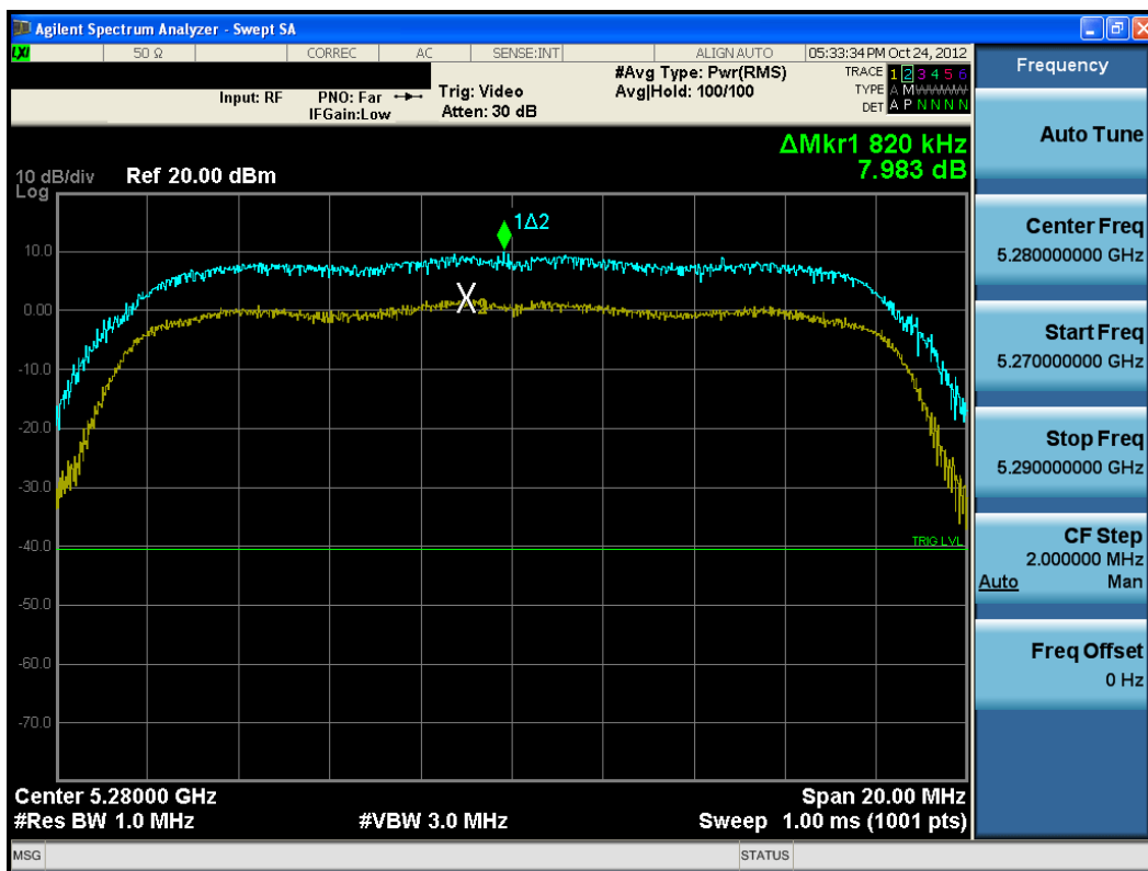
Plot 6-53. Peak Excursion Ratio Plot (802.11a (UNII Band 2) – Ch. 56)
