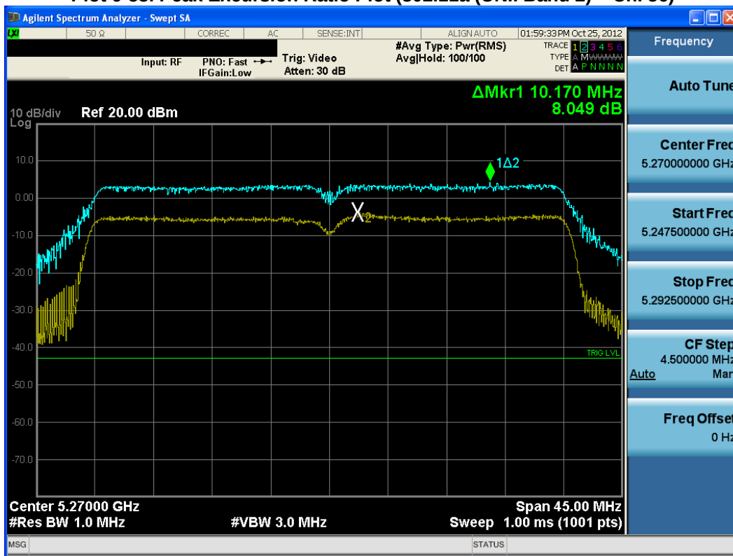
Plot 6-54. Peak Excursion Ratio Plot (40MHz BW 802.11n (UNII Band 2) – Ch. 54)
