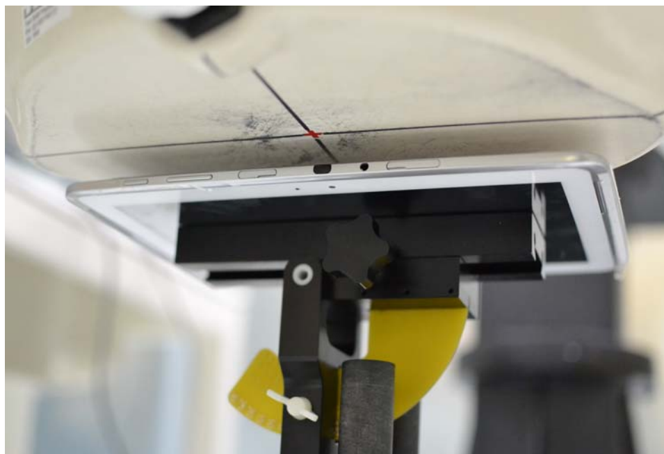
SAR Test Setup Photo 1: Back Side at 1.2 cm
