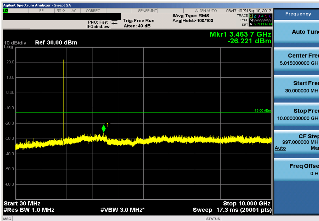
Plot 7-30. Conducted Spurious Plot (PCS WCDMA Mode – Ch. 9538)
