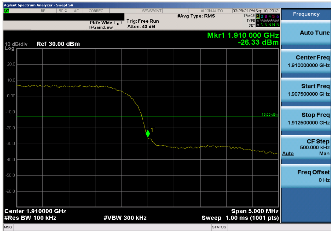
Plot 7-32. Band Edge Plot (PCS WCDMA Mode – Ch. 9538)
