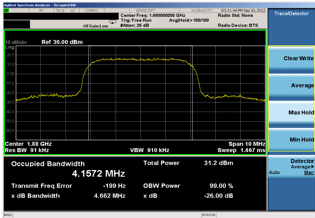
Plot 7-28. Occupied Bandwidth Plot (PCS WCDMA Mode – Ch. 9400)
