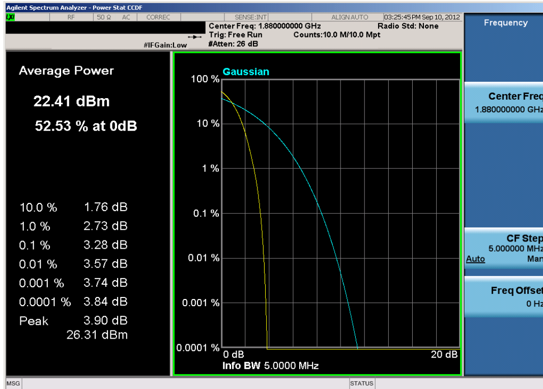
Plot 7-29. Peak-Average Ratio Plot (PCS WCDMA Mode – Ch. 9400)
