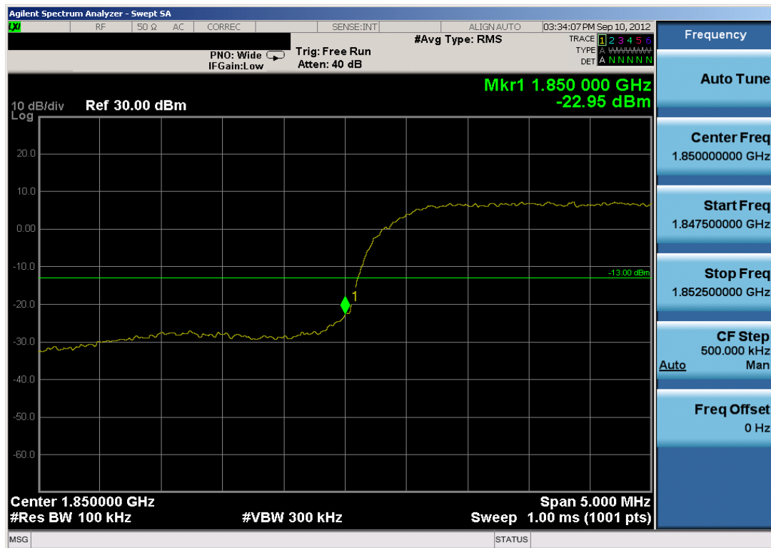
Plot 7-24. Band Edge Plot (PCS WCDMA Mode – Ch. 9262)
