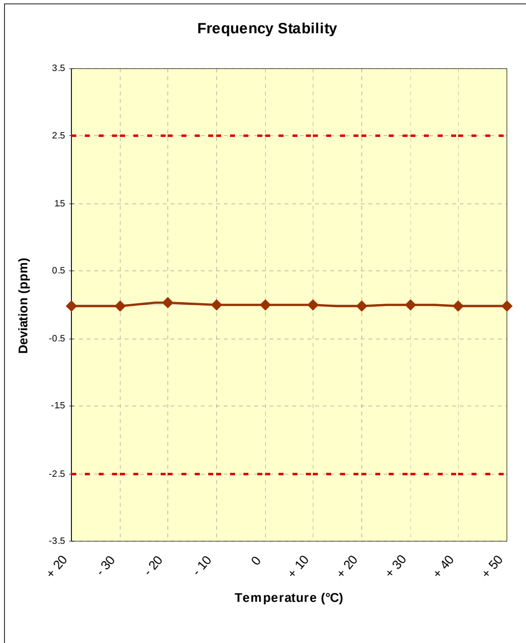
Figure 6-1. Frequency Stability Graph (Cellular WCDMA Mode – Ch. 4183)
