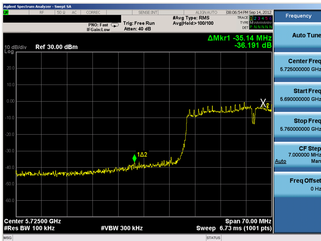
Plot 6-43. Band Edge Plot (40MHz BW 802.11n (5.8GHz) – Ch. 151)
