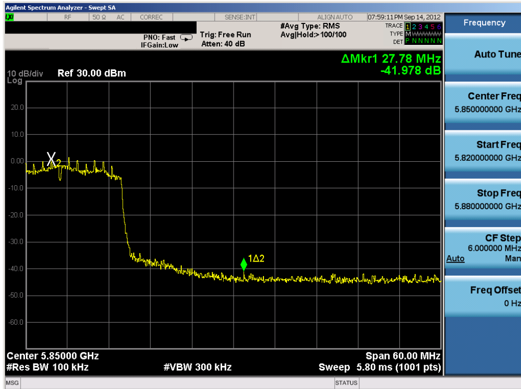
Plot 6-42. Band Edge Plot (20MHz BW 802.11n (5.8GHz) – Ch. 165)
