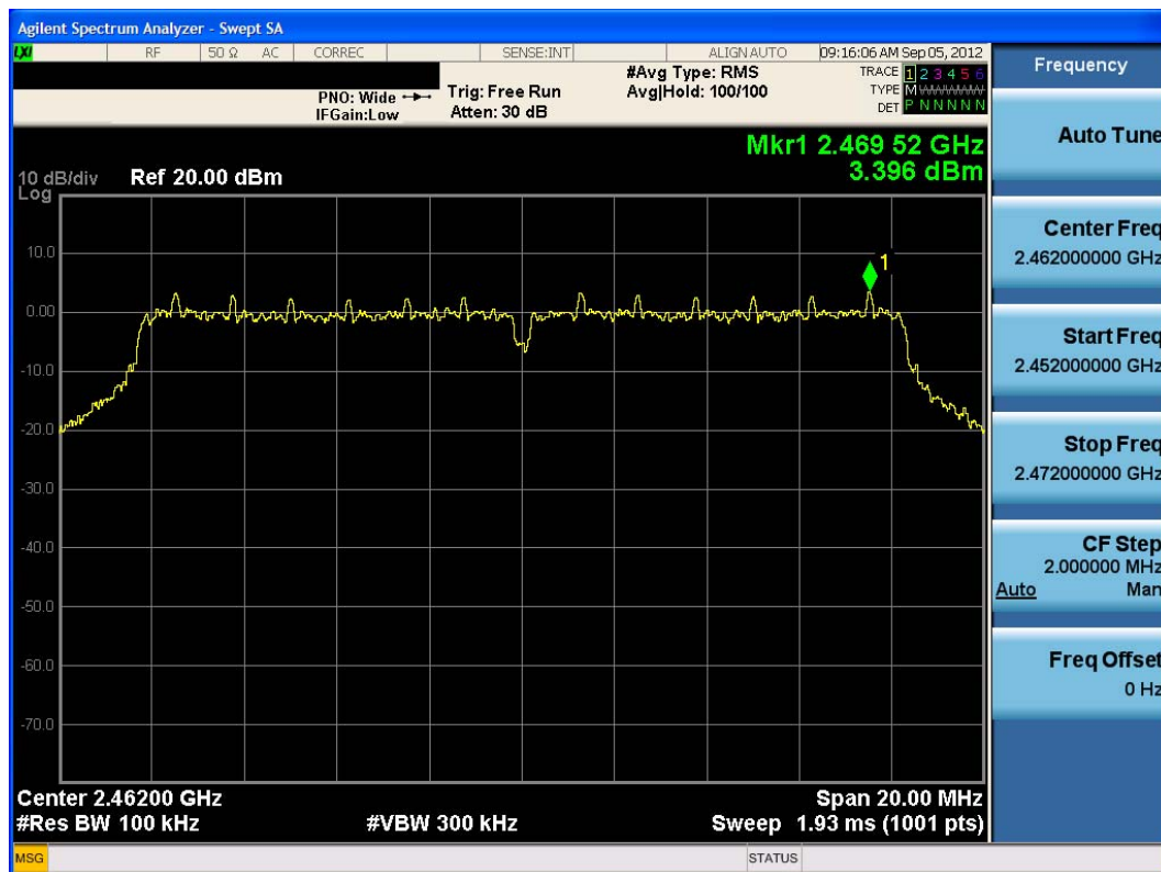
Plot 6-22. Power Spectral Density Plot (802.11g – Ch. 11)
