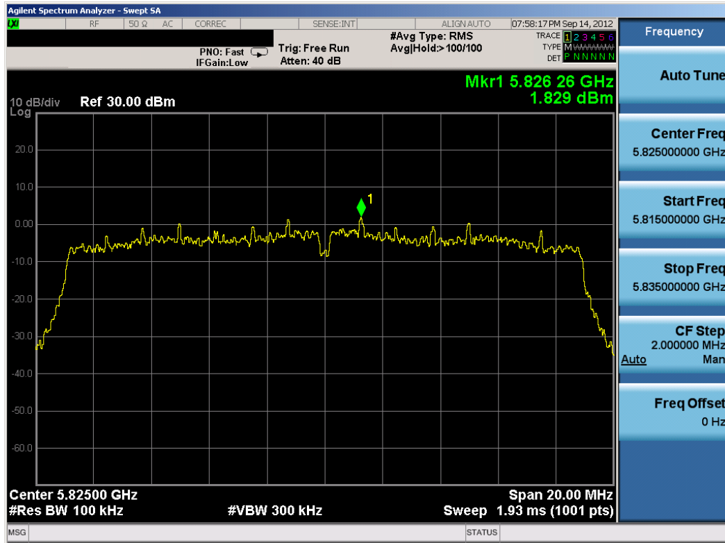
Plot 6-31. Power Spectral Density Plot (20MHz BW 802.11n (5.8GHz) – Ch. 165)
