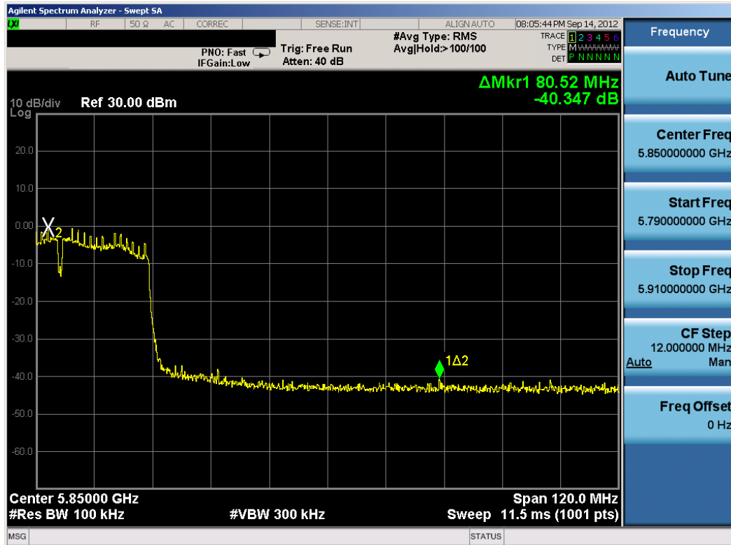
Plot 6-44. Band Edge Plot (40MHz BW 802.11n (5.8GHz) – Ch. 159)
