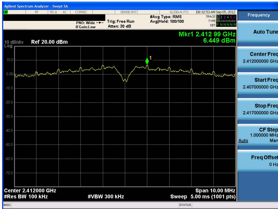
Plot 6-17. Power Spectral Density Plot (802.11b - Ch. 1)
