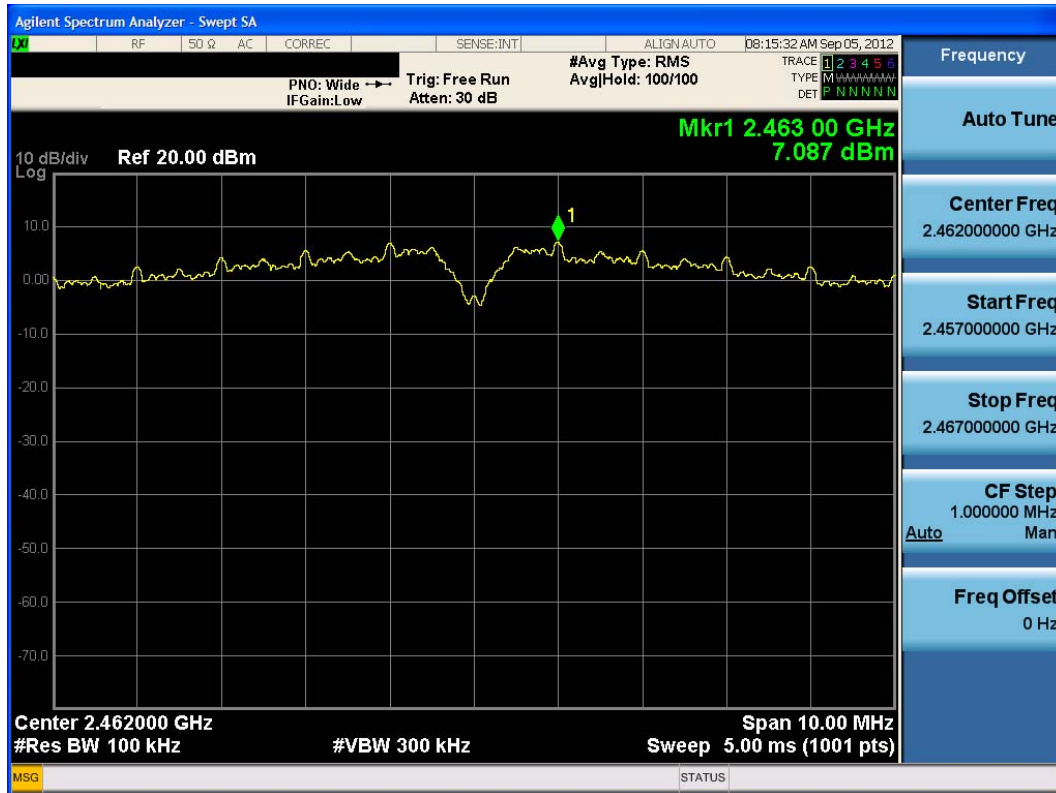
Plot 6-19. Power Spectral Density Plot (802.11b – Ch. 11)
