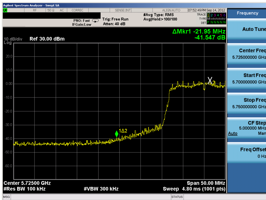
Plot 6-39. Band Edge Plot (802.11a – Ch. 149)
