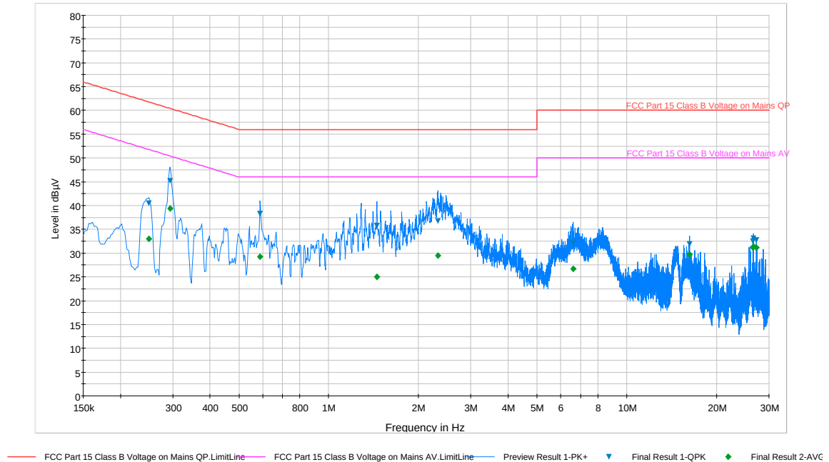
Plot 6-59. Line Conducted Plot with 802.11a (L1)
