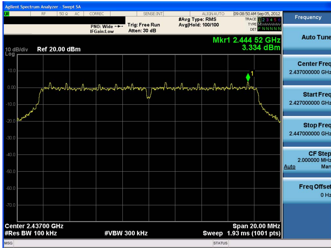
Plot 6-21. Power Spectral Density Plot (802.11g – Ch. 6)
