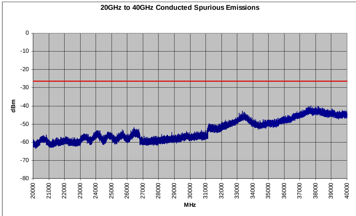
Plot 6-54. Conducted Spurious Plot (802.11a – Ch. 157)
