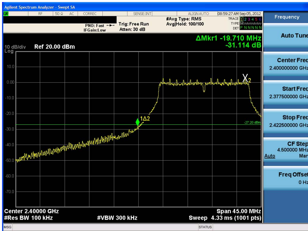
Plot 6-35. Band Edge Plot (802.11g – Ch. 1)
