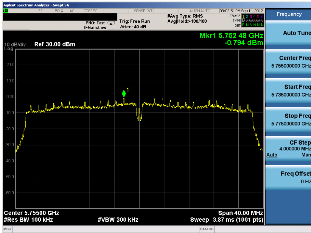
Plot 6-32. Power Spectral Density Plot (40MHz BW 802.11n (5.8GHz) – Ch. 151)
