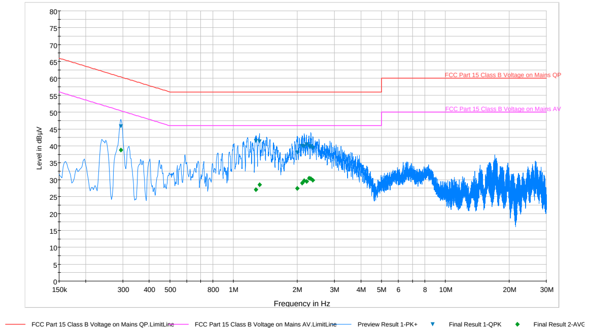
Plot 6-60. Line Conducted Plot with 802.11a (N)
