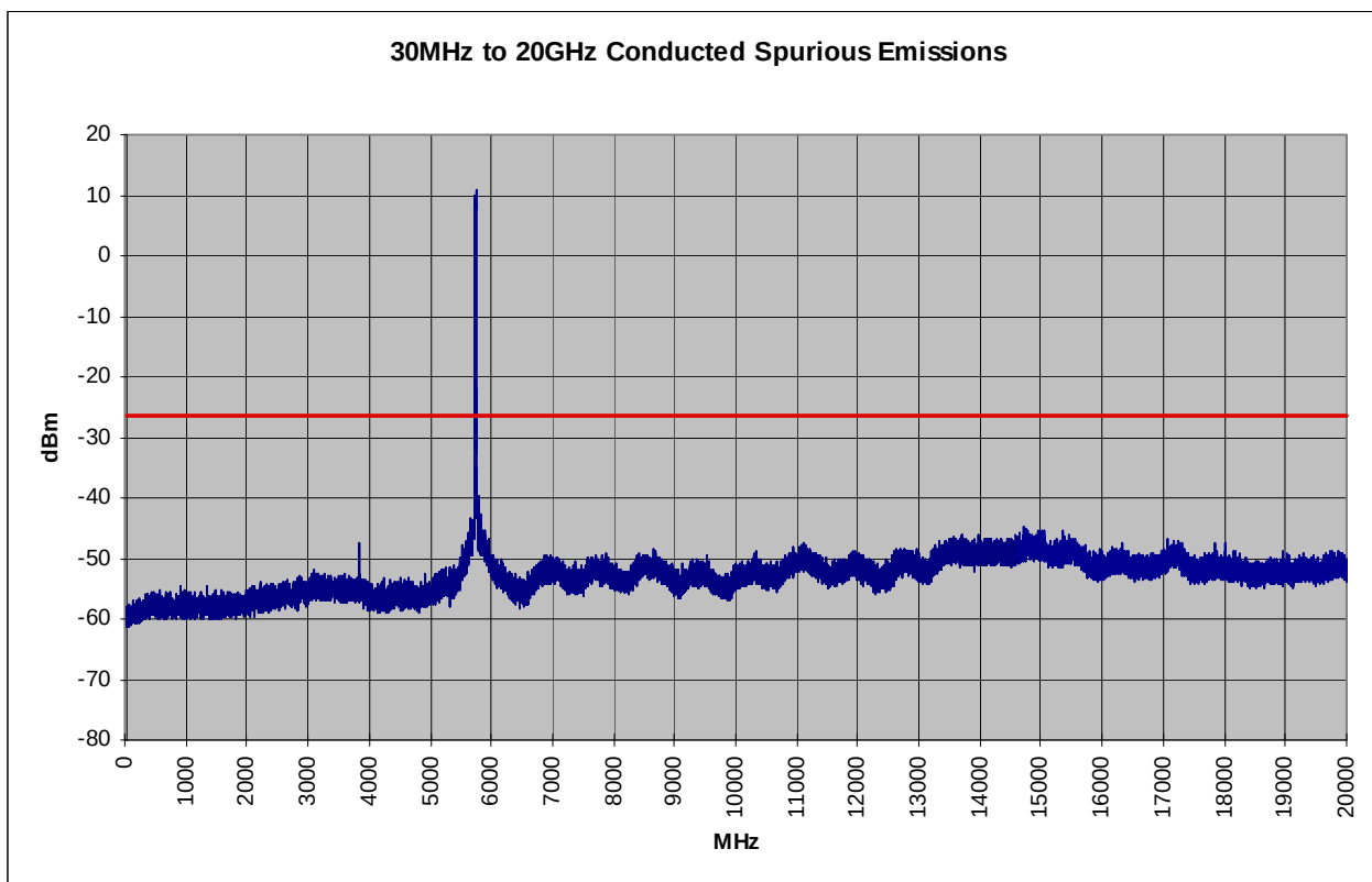
Plot 6-51. Conducted Spurious Plot (802.11a – Ch. 149)
