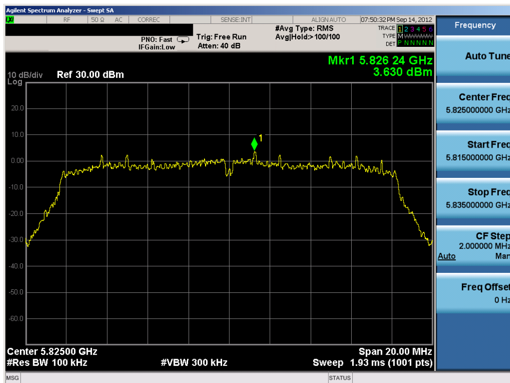
Plot 6-28. Power Spectral Density Plot (802.11a – Ch. 165)
