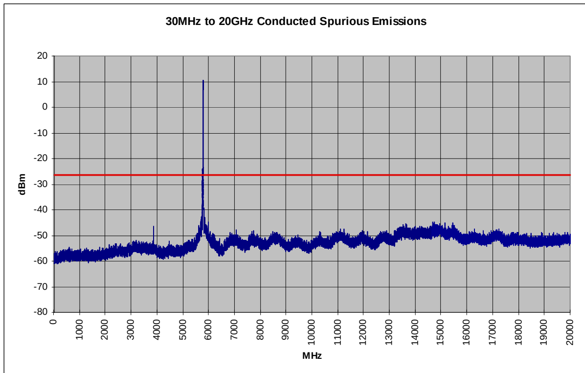
Plot 6-53. Conducted Spurious Plot (802.11a – Ch. 157)
