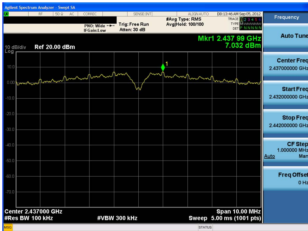
Plot 6-18. Power Spectral Density Plot (802.11b - Ch. 6)
