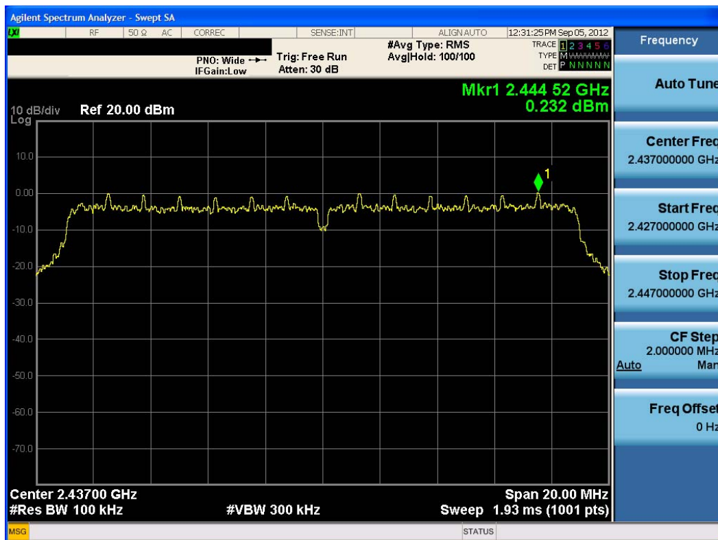
Plot 6-24. Power Spectral Density Plot (802.11n (2.4GHz) – Ch. 6)
