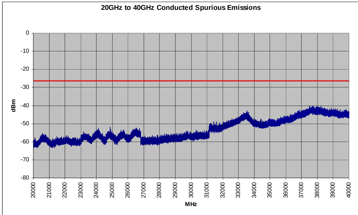
Plot 6-52. Conducted Spurious Plot (802.11a – Ch. 149)
