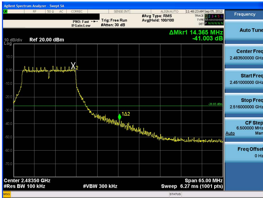
Plot 6-36. Band Edge Plot (802.11g – Ch. 11)
