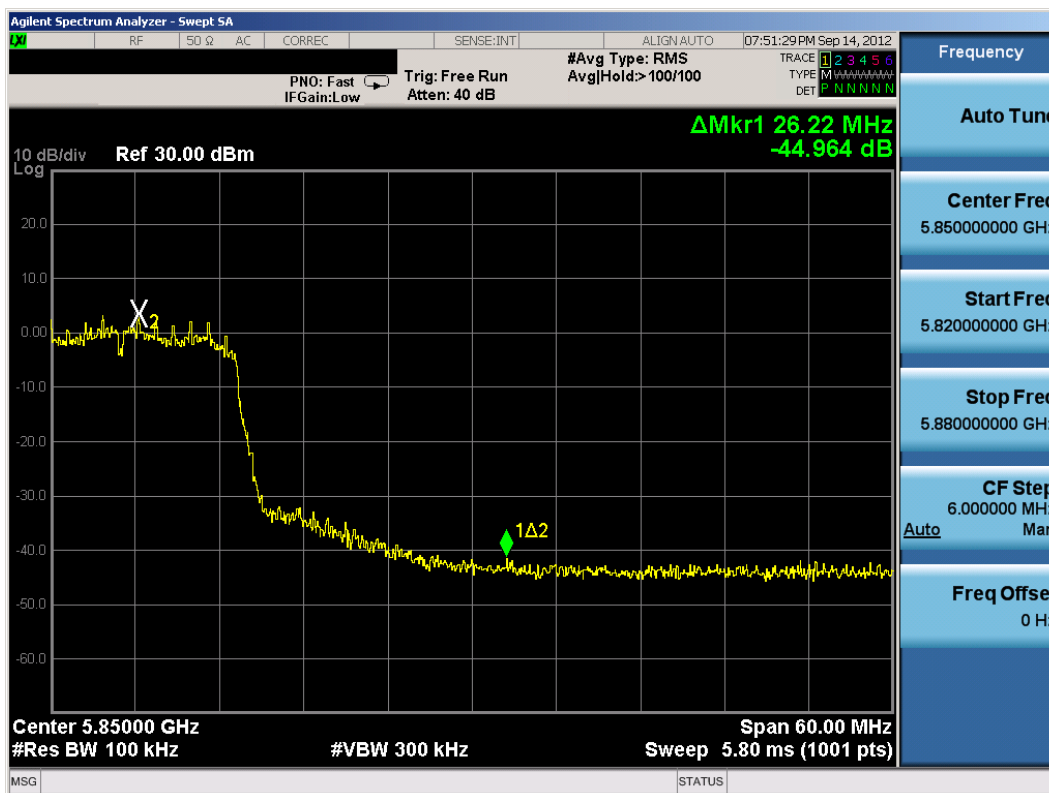
Plot 6-40. Band Edge Plot (802.11a – Ch. 165)
