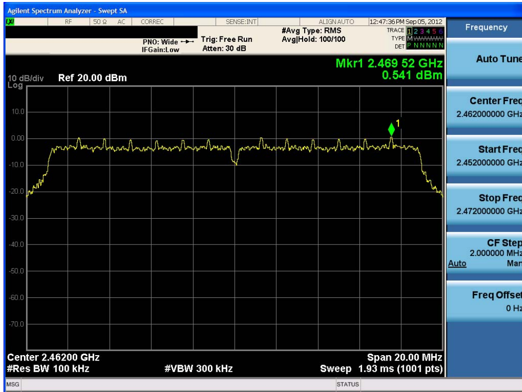
Plot 6-25. Power Spectral Density Plot (802.11n (2.4GHz) – Ch. 11)
