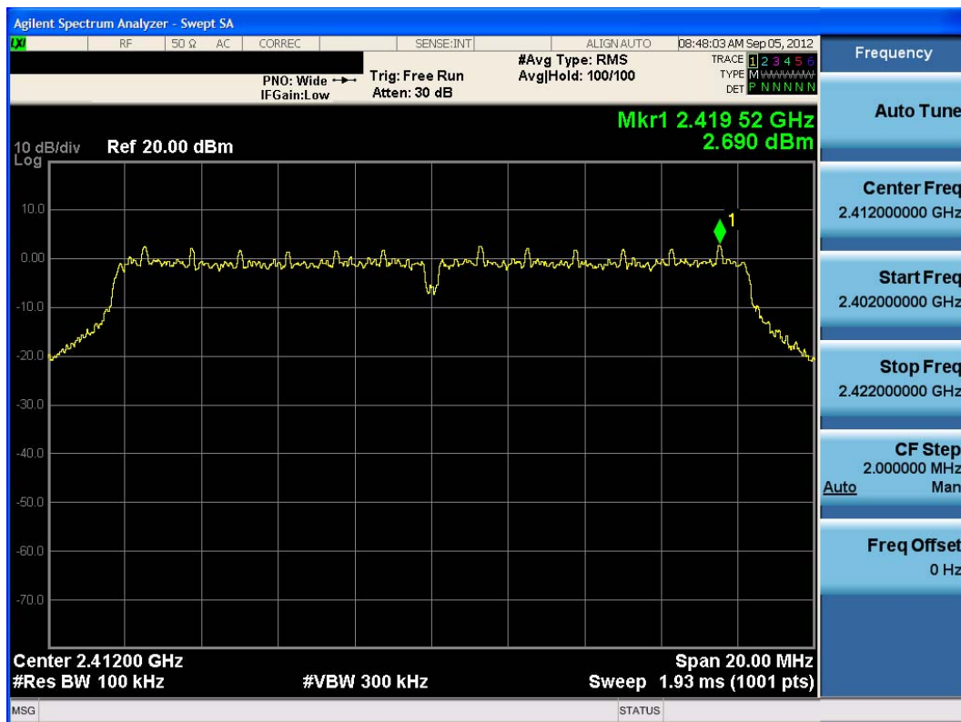
Plot 6-20. Power Spectral Density Plot (802.11g – Ch. 1)
