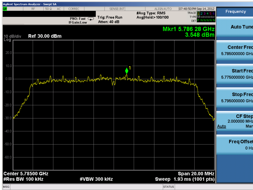
Plot 6-27. Power Spectral Density Plot (802.11a – Ch. 157)
