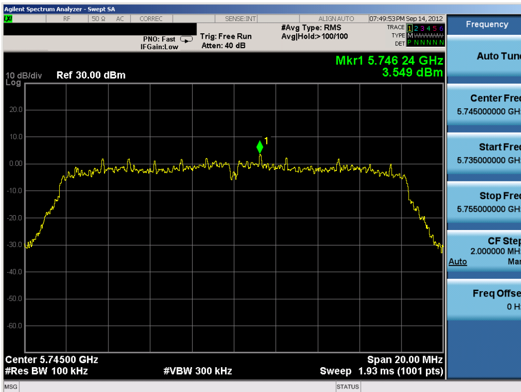
Plot 6-26. Power Spectral Density Plot (802.11a – Ch. 149)
