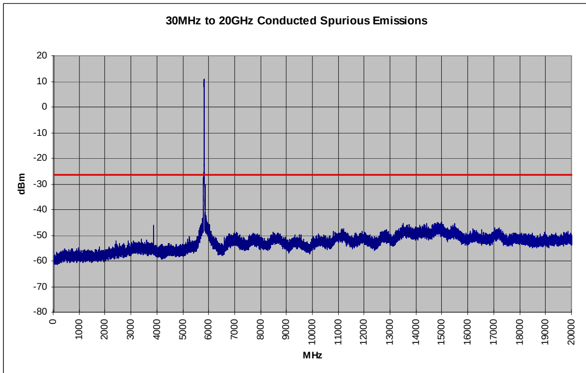
Plot 6-55. Conducted Spurious Plot (802.11a – Ch. 165)
