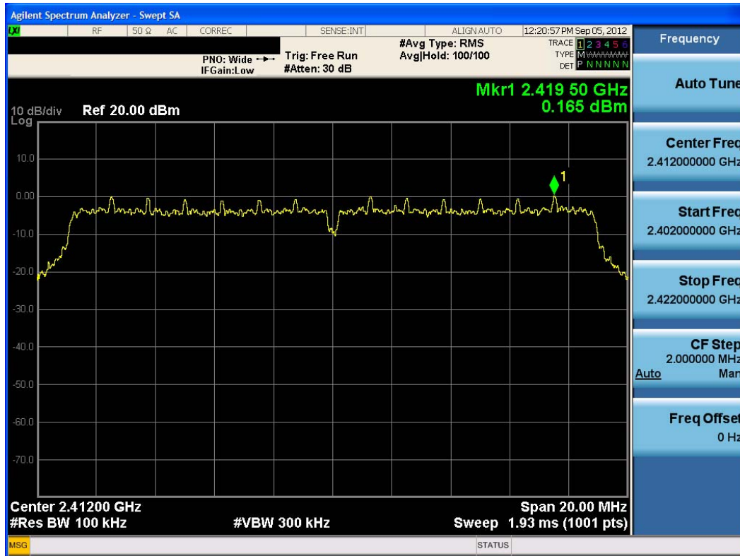
Plot 6-23. Power Spectral Density Plot (802.11n (2.4GHz) – Ch. 1)
