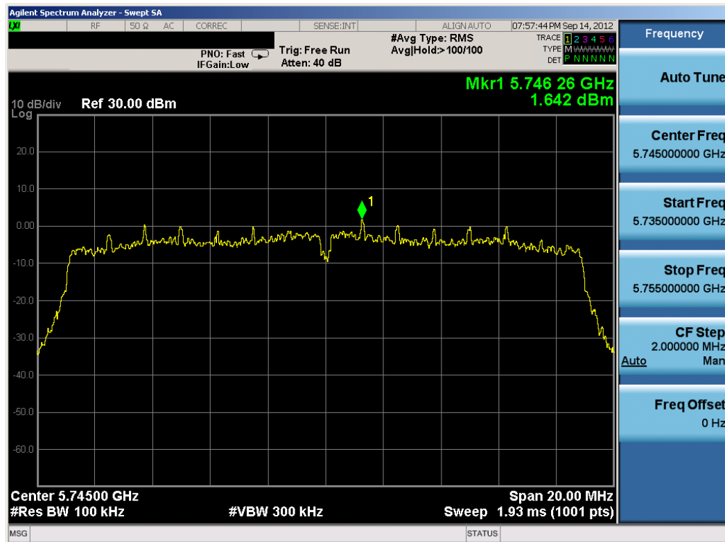
Plot 6-29. Power Spectral Density Plot (20MHz BW 802.11n (5.8GHz) - Ch. 149)
