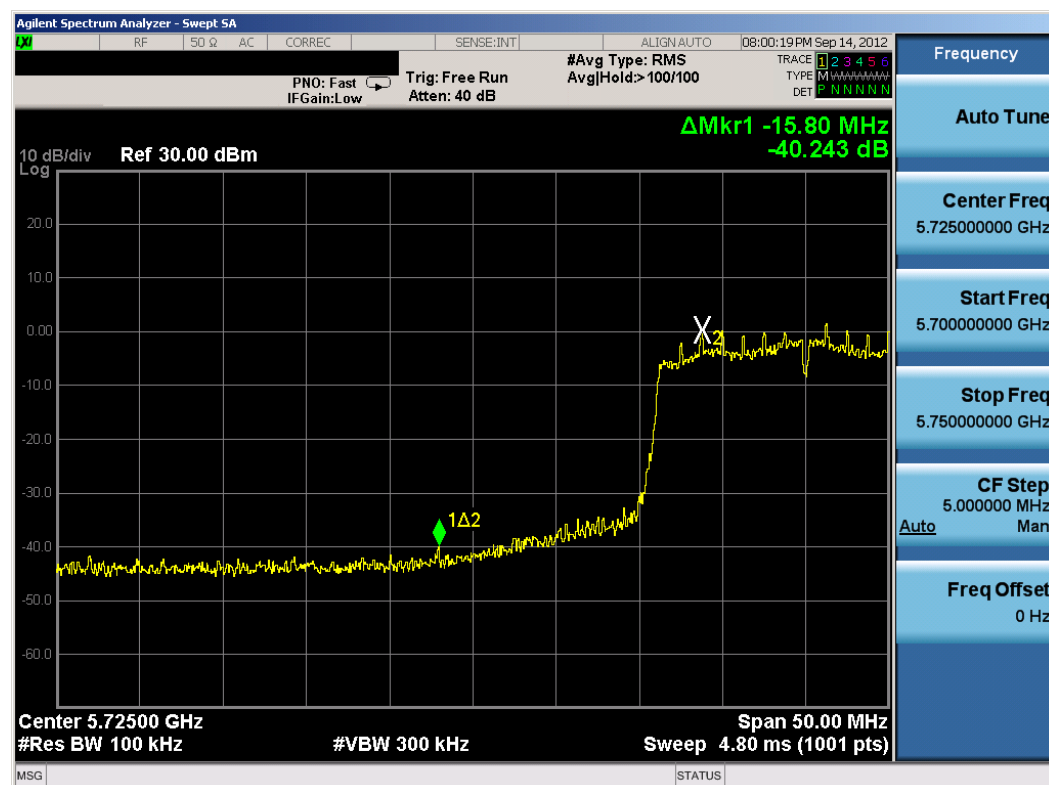
Plot 6-41. Band Edge Plot (20MHz BW 802.11n (5.8GHz) – Ch. 149)
