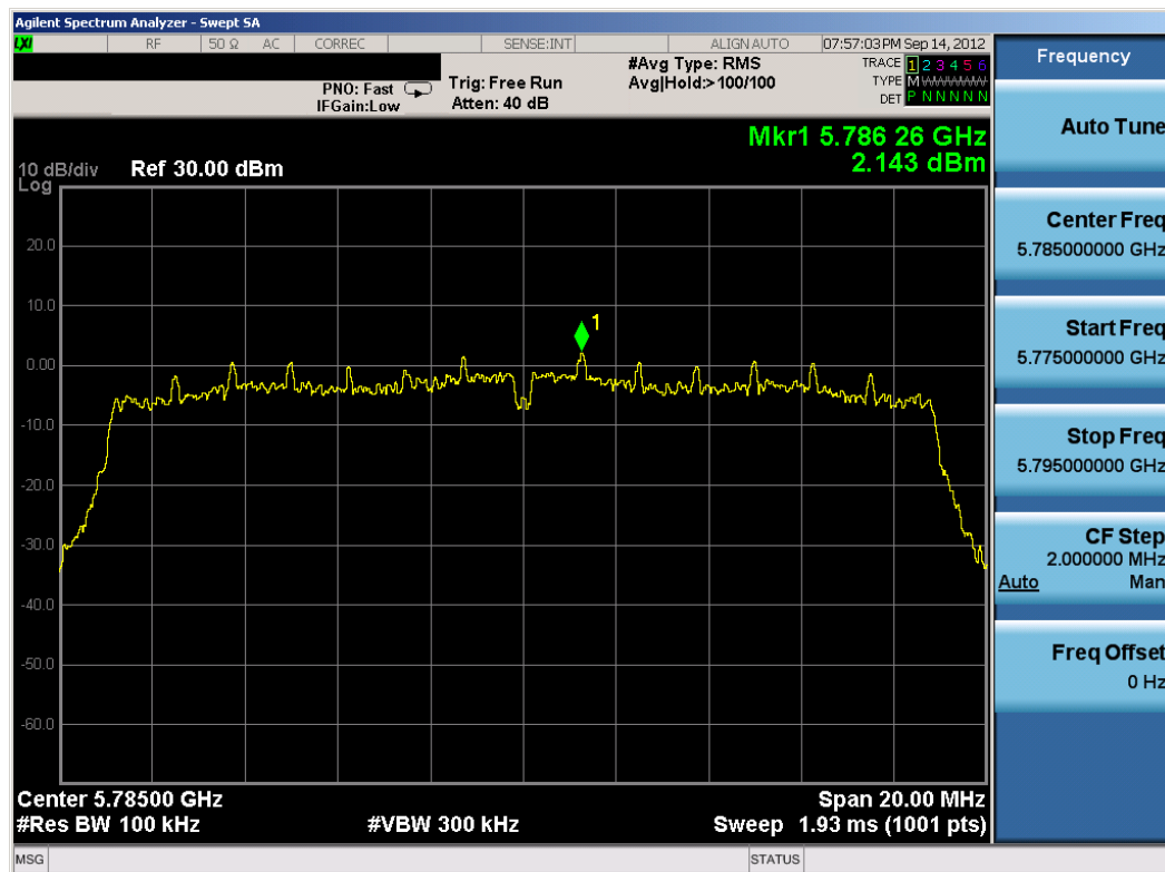
Plot 6-30. Power Spectral Density Plot (20MHz BW 802.11n (5.8GHz) - Ch. 157)
