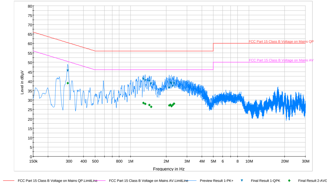
Plot 6-58. Line Conducted Plot with 802.11b (N)
