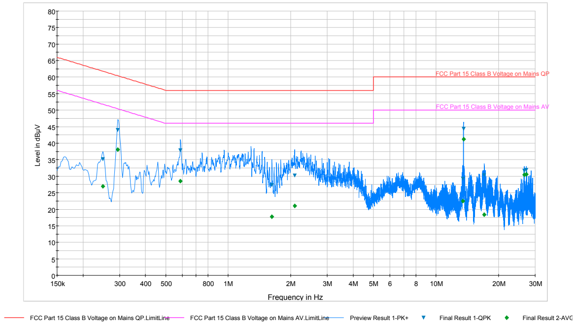
Plot 8-1. Line-Conducted Test Plot (L1)
