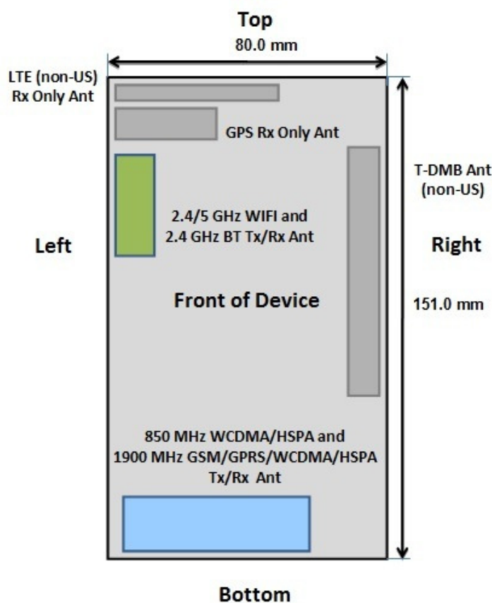
Figure 1-1 DUT Antenna Locations
