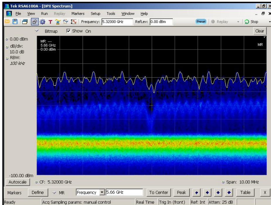
Figure 5-4. Real-Time Spectrum Display, WLAN Traffic (Streaming Video)
