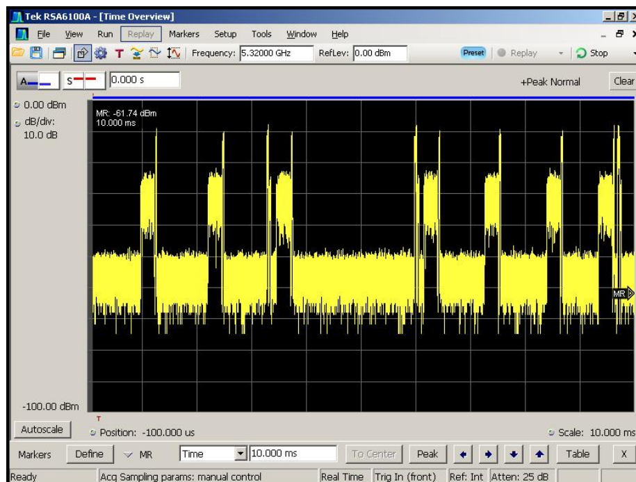
Figure 5-2. Time Display WLAN Channel Traffic (Streaming Video)
