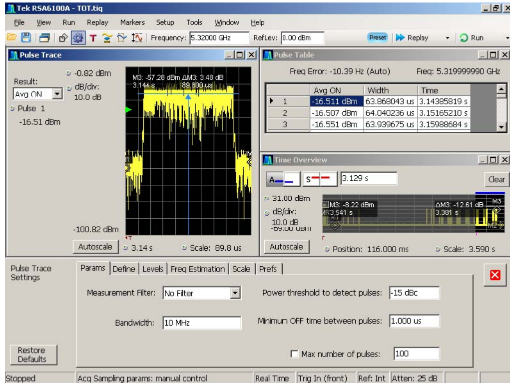
Figure 6-7. Pulse width analysis using Pulse Table and Pulse Trace Function
