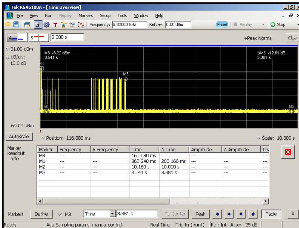
Figure 5-5. Channel Move Time (< 10sec)
