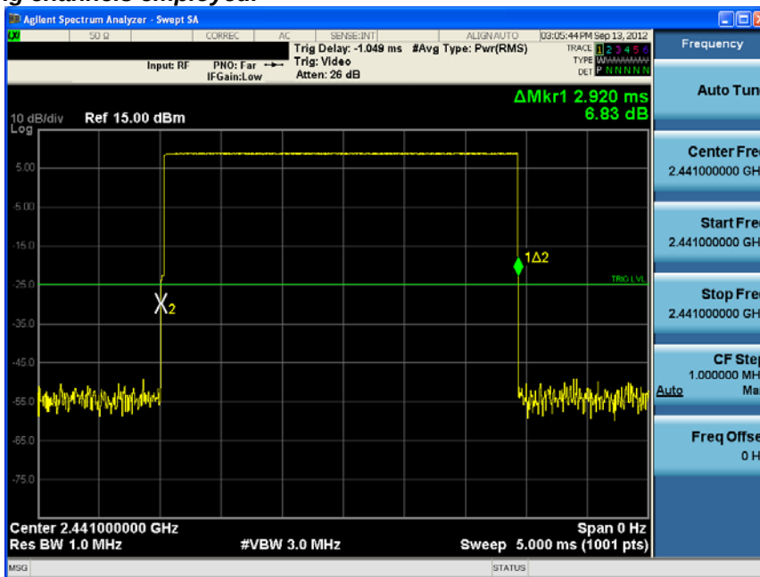
Plot 6-24. Time of Occupancy Plot (Bluetooth)
