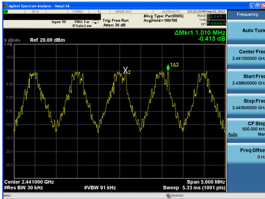
Plot 6-23. Channel Spacing Plot (Bluetooth)
