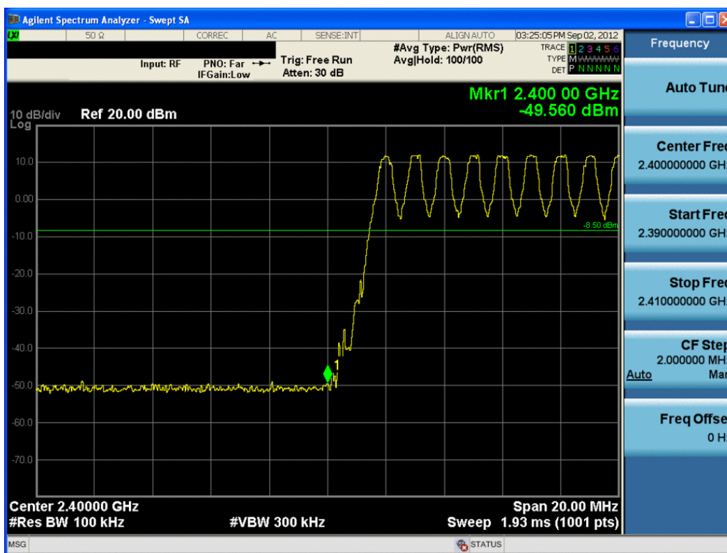
Plot 6-21. Band Edge Plot (Bluetooth with Hopping Enabled, 3Mbps)
