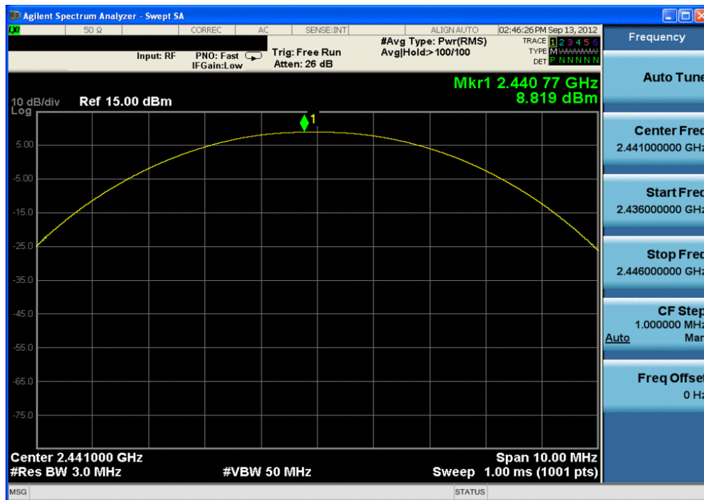
Plot 6-11 Peak Conducted Power (1Mbps – Ch. 39)
