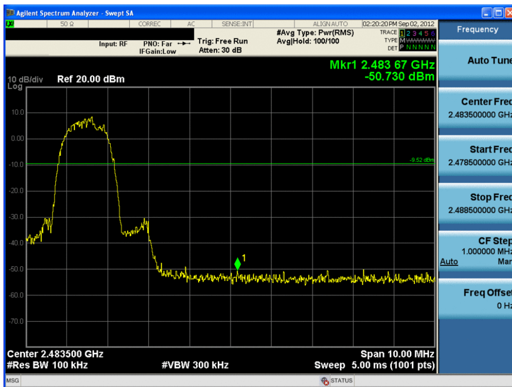
Plot 6-20. Band Edge Plot (Bluetooth with Hopping Disabled, 3Mbps – Ch. 78)
