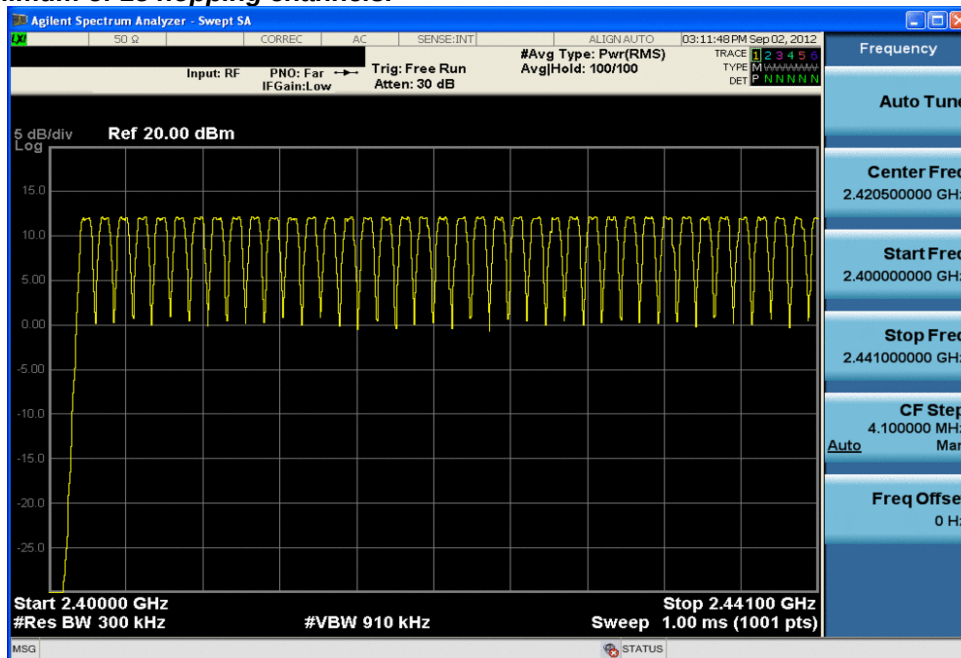
Plot 6-25. Low End Spectrum Channel Hopping Plot (Bluetooth)
