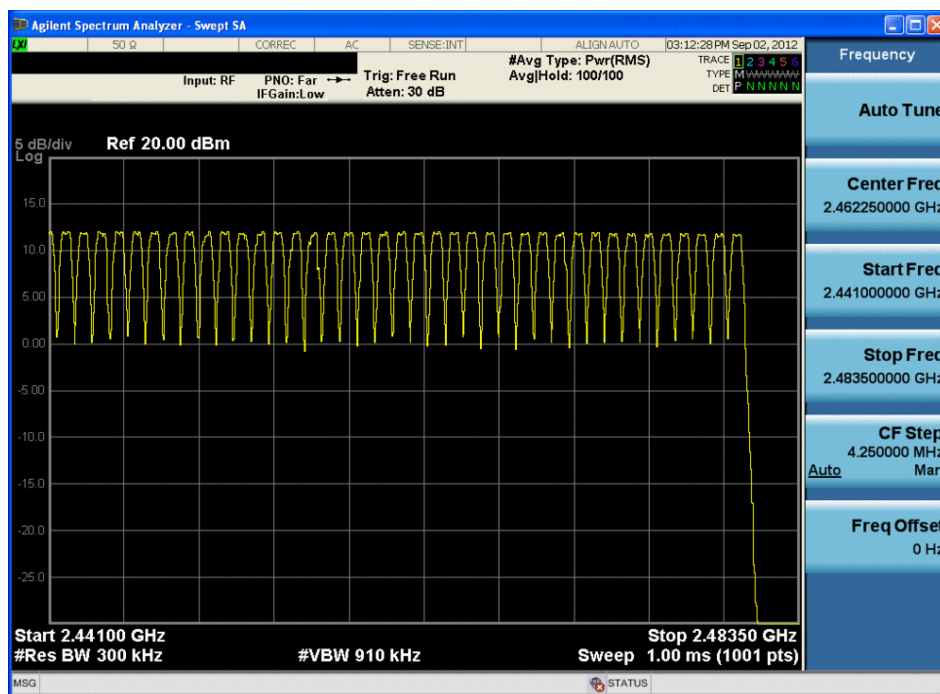
Plot 6-26. High End Spectrum Channel Hopping Plot (Bluetooth)
