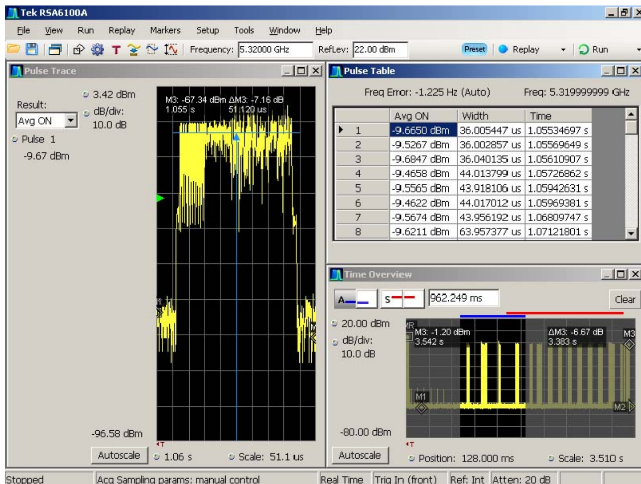
Figure 5-6. Aggregate Time using Pulse Table Capability
