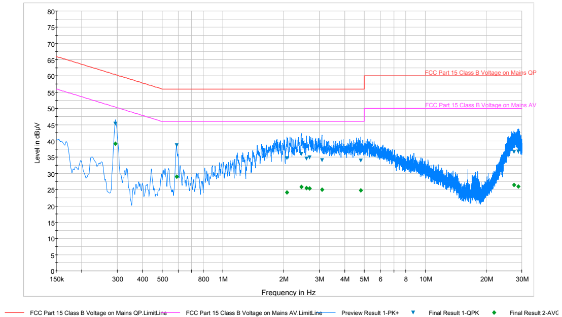
Plot 6-62. Line Conducted Plot with 802.11a (N)
