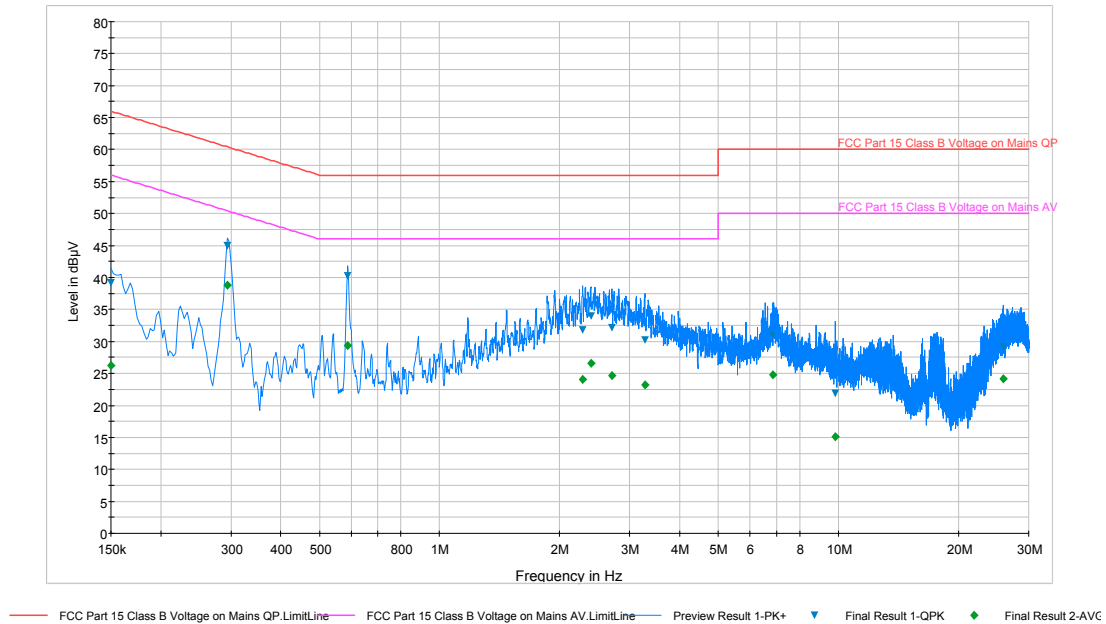
Plot 6-61. Line Conducted Plot with 802.11a (L1)
