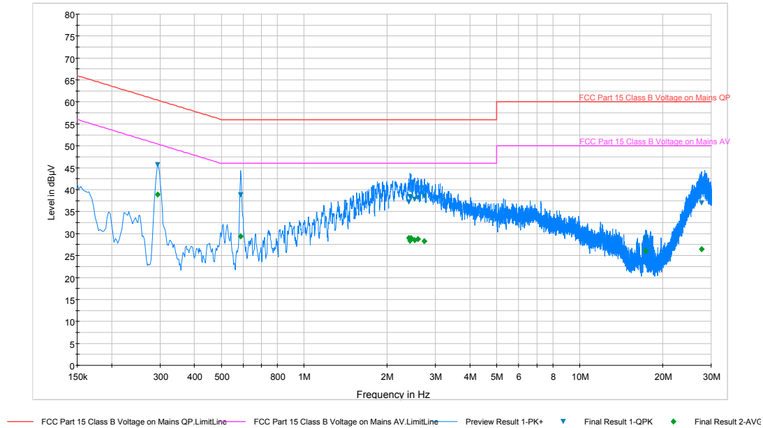
Plot 6-60. Line Conducted Plot with 802.11b (N)
