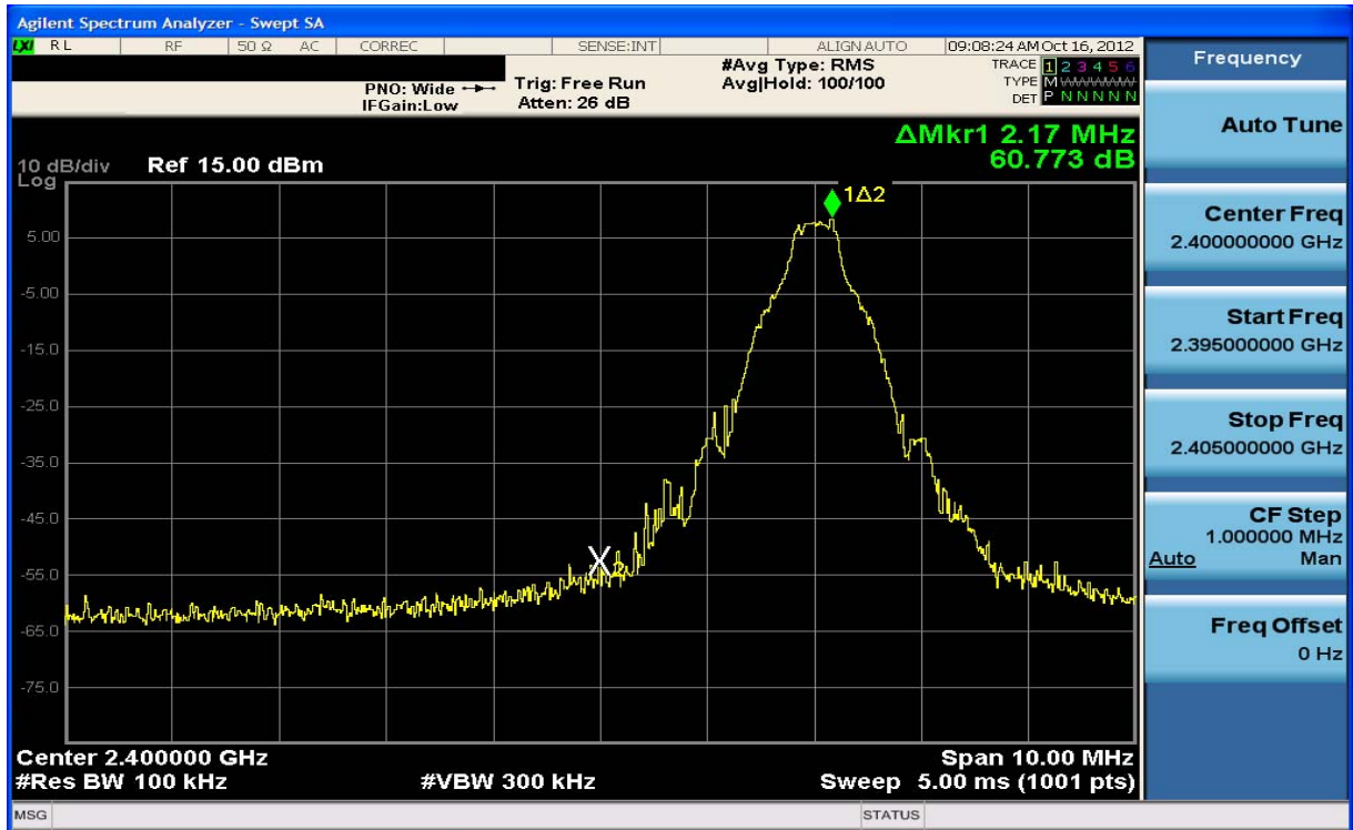
Plot 6-19. Band Edge Plot (Bluetooth with Hopping Disabled, 1Mbps – Ch. 0)
