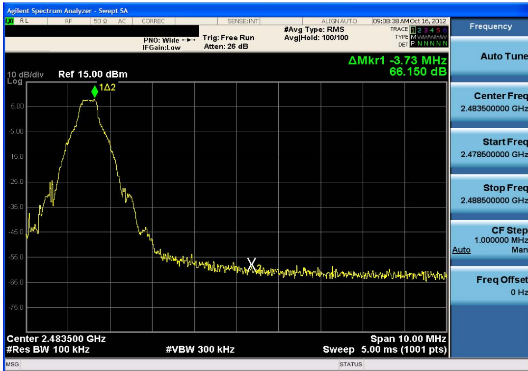
Plot 6-20. Band Edge Plot (Bluetooth with Hopping Disabled, 1Mbps – Ch. 78)
