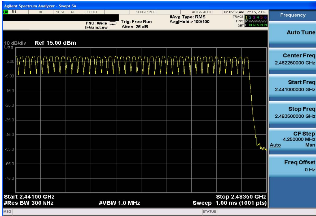
Plot 6-26. High End Spectrum Channel Hopping Plot (Bluetooth)
