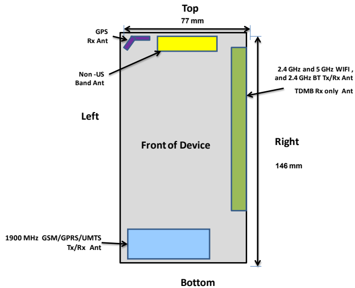
Figure 1-1 DUT Antenna Locations
