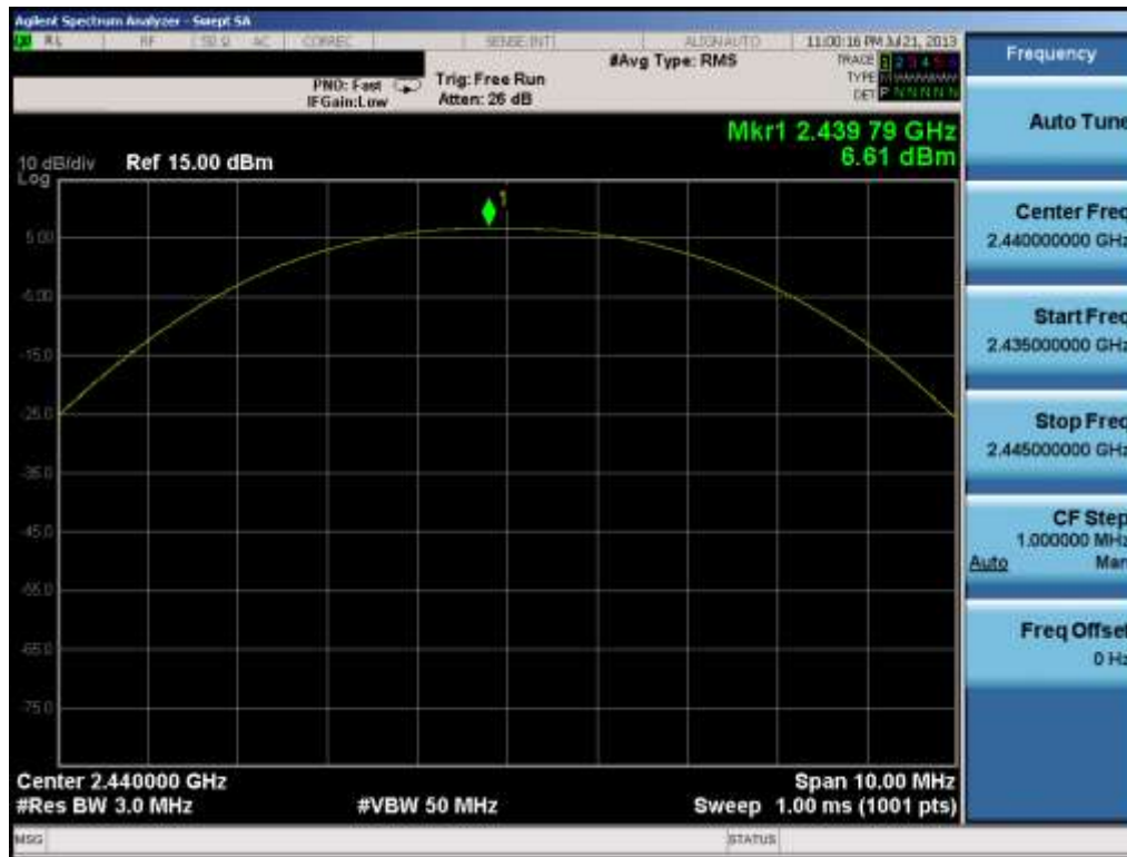
Plot 6-5. Peak Powery Plot (Bluetooth (LE) – Ch. 19)
