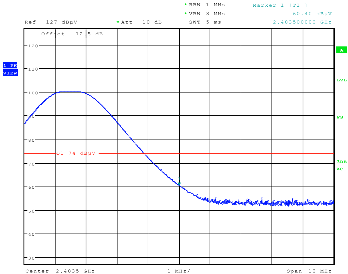
Plot 6-19. Radiated Restricted Upper Band Edge Measurement (Peak)
