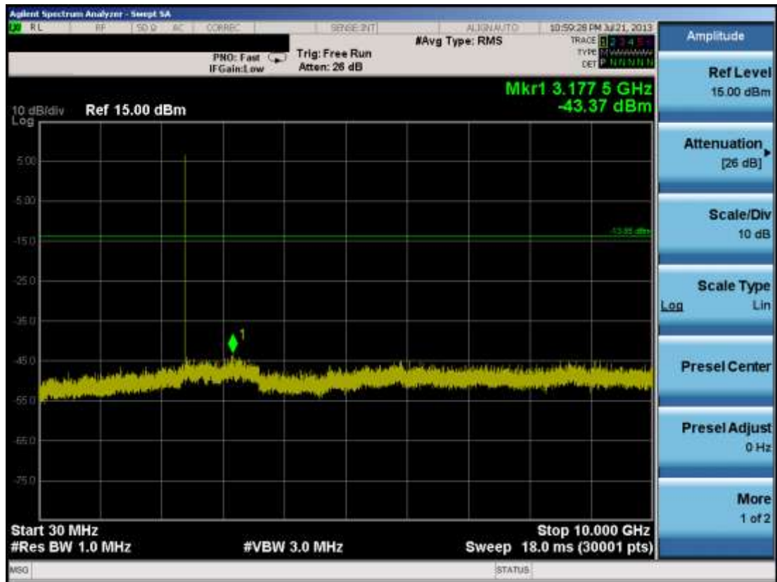
Plot 6-12. Conducted Spurious Plot (Bluetooth (LE) – Ch. 0)
