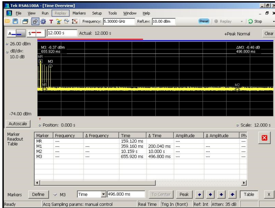
Figure 5-4. Channel Move Time (< 10sec)
