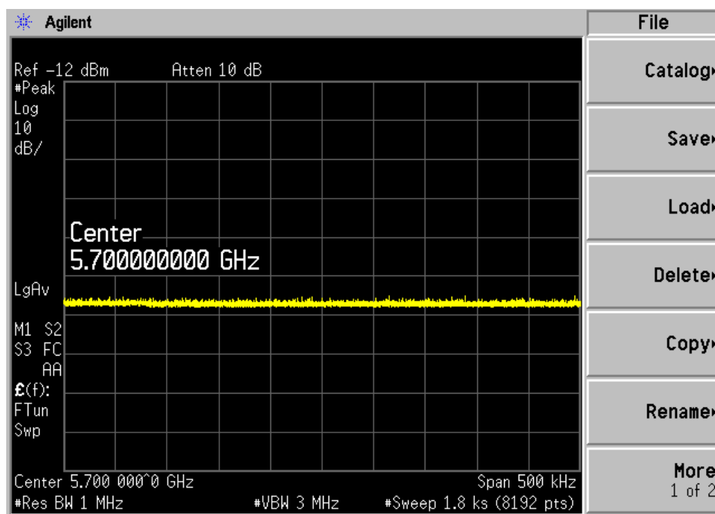
Figure 6-5. Non-occupancy Period - Monitoring live spectrum - Elapse time 30 minutes
