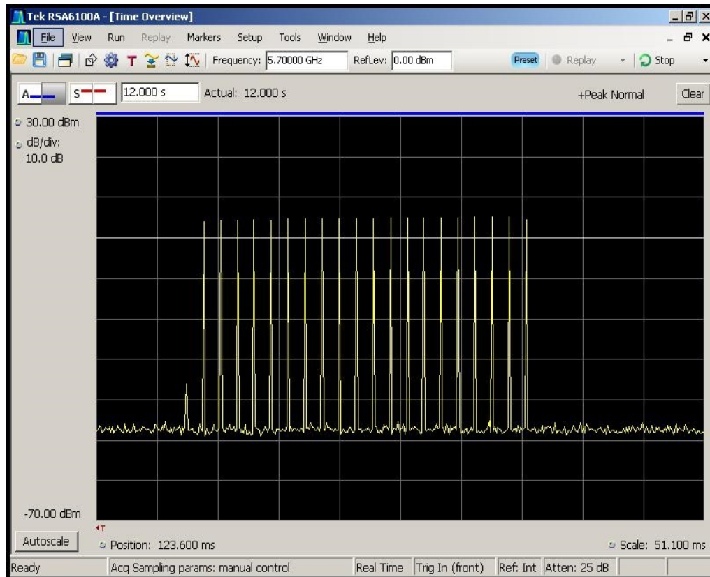
Figure 6-1. Type 1 Radar Pulse
