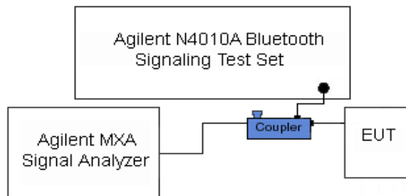
Figure 6-2. Test Instrument & Measurement Setup
