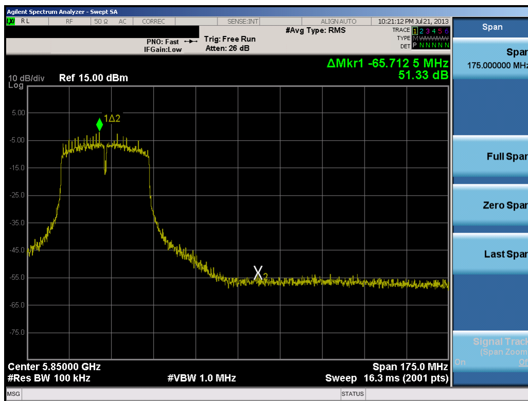
Plot 6-46. Band Edge Plot (40MHz BW 802.11n (5.8GHz) – Ch. 159)
