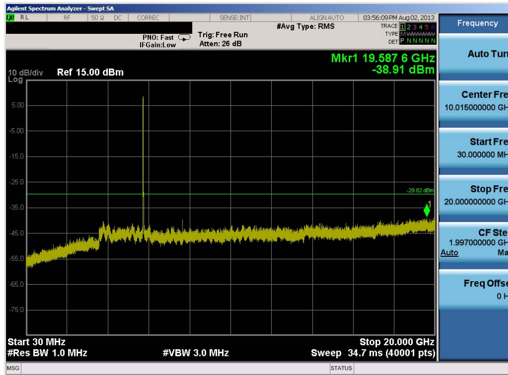
Plot 6-53. Conducted Spurious Plot (802.11a – Ch. 149)
