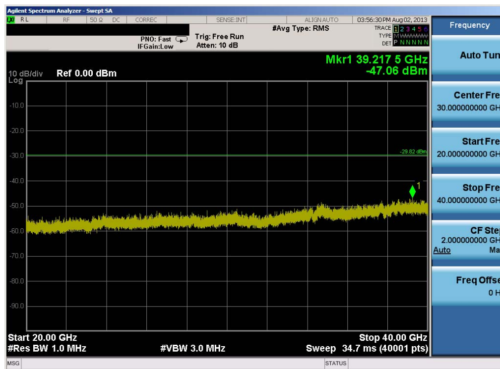
Plot 6-54. Conducted Spurious Plot (802.11a – Ch. 149)
