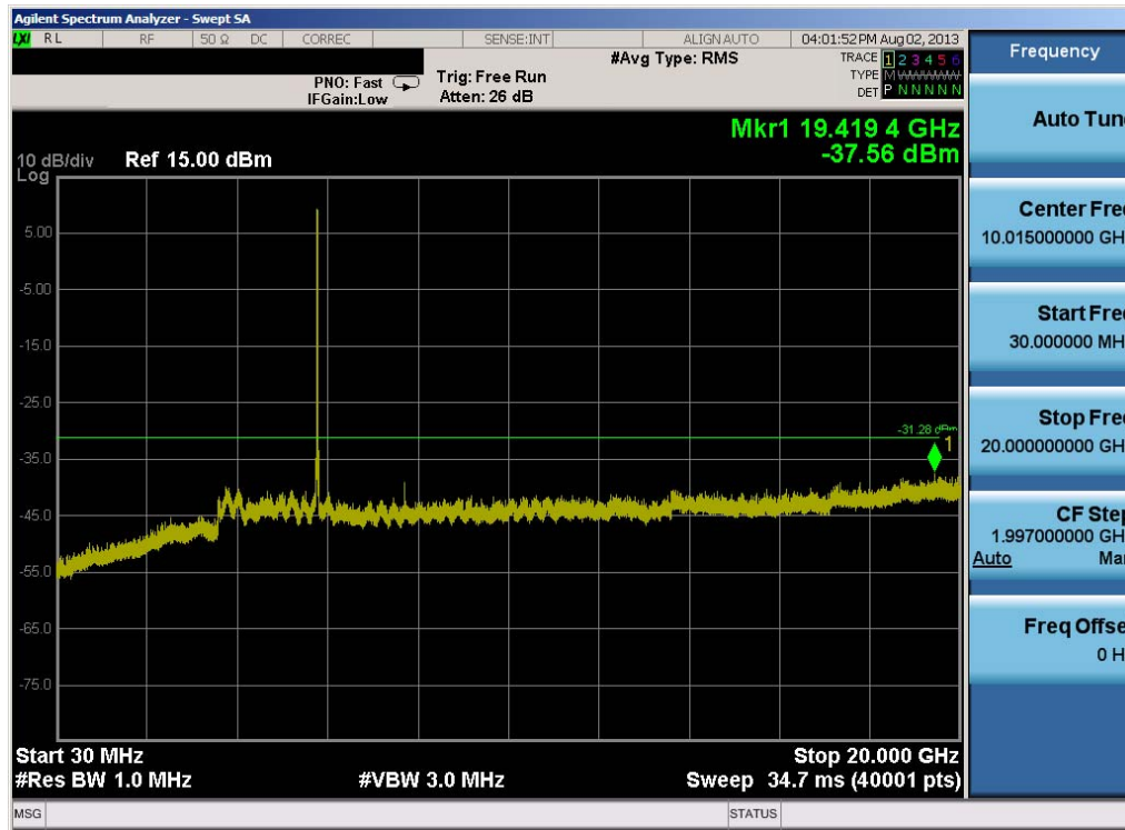
Plot 6-55. Conducted Spurious Plot (802.11a – Ch. 157)
