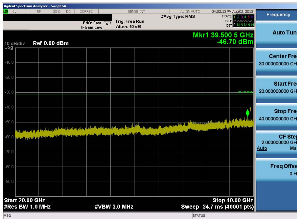
Plot 6-56. Conducted Spurious Plot (802.11a – Ch. 157)
