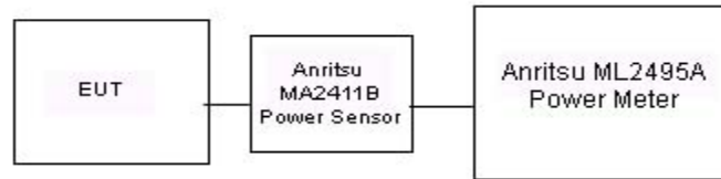
Figure 6-2. Test Instrument & Measurement Setup for Power Meter Measurements
