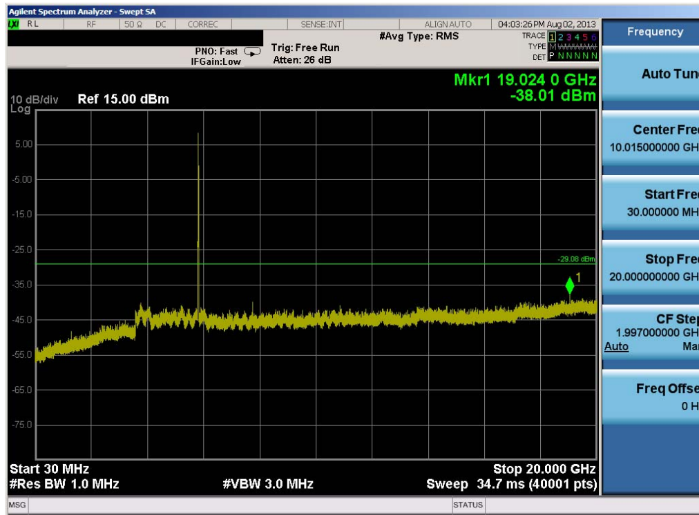
Plot 6-57. Conducted Spurious Plot (802.11a – Ch. 165)
