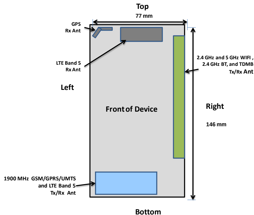
Figure 1-1 DUT Antenna Locations
