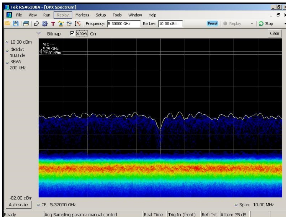
Figure 5-2. Real-Time Spectrum Display, No WLAN Traffic
