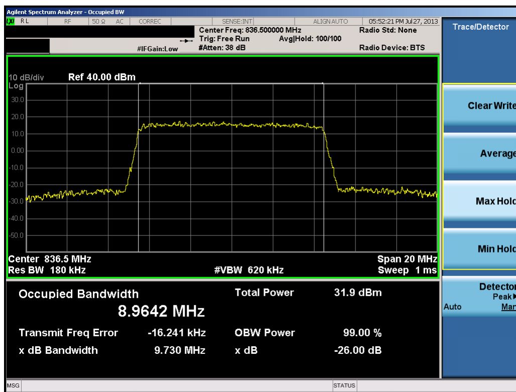
Plot 7-15. Occupied Bandwidth Plot (10.0MHz QPSK – RB Size 50)
