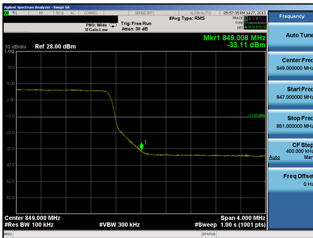
Plot 7-23. Upper Band Edge Plot (10.0MHz QPSK – RB Size 50)
