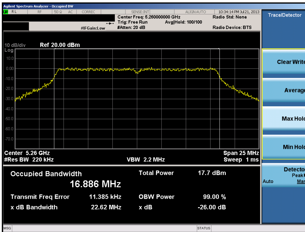
Plot 6-9. 26dB Bandwidth Plot (802.11a (UNII Band 2) – Ch. 52)
