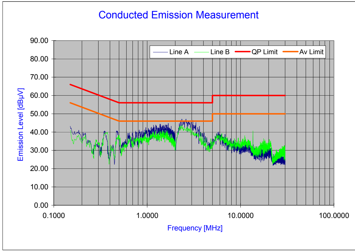
Plot 6-44. Line-Conducted Test Plot (L1)
