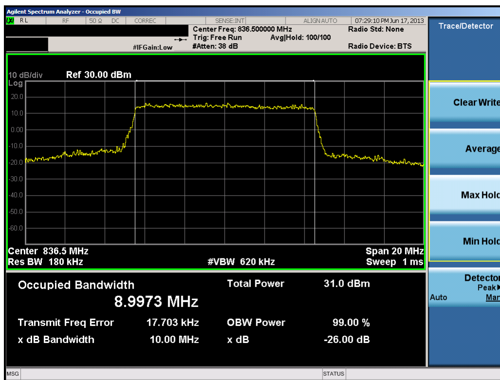
Plot 7-16. Occupied Bandwidth Plot (10.0MHz 16-QAM – RB Size 50)
