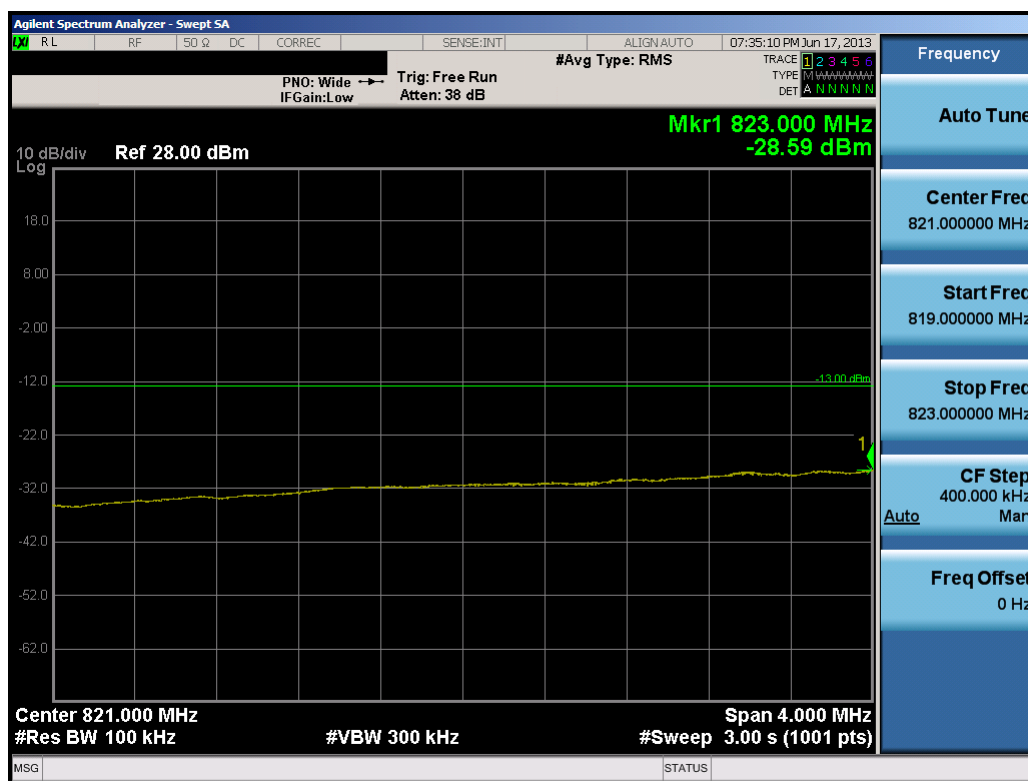
Plot 7-14. Lower Extended Band Edge Plot (10.0MHz QPSK – RB Size 50)
