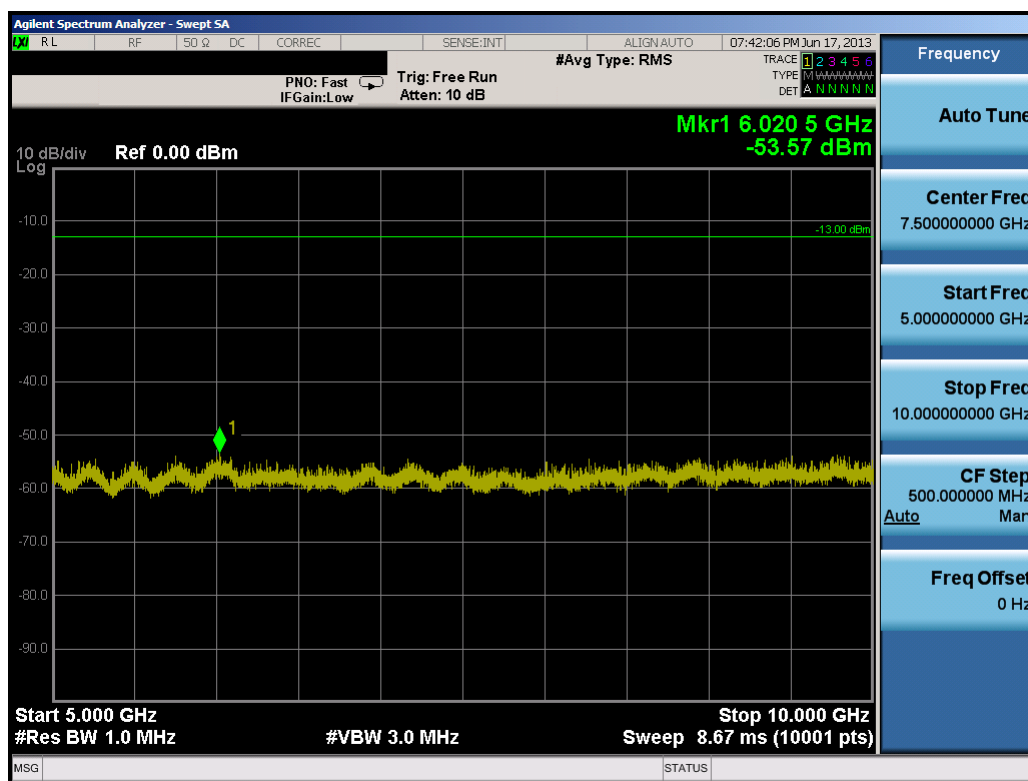
Plot 7-6. Conducted Spurious Plot (5.0MHz QPSK – RB Size 1, RB Offset 0 – Low Channel)
