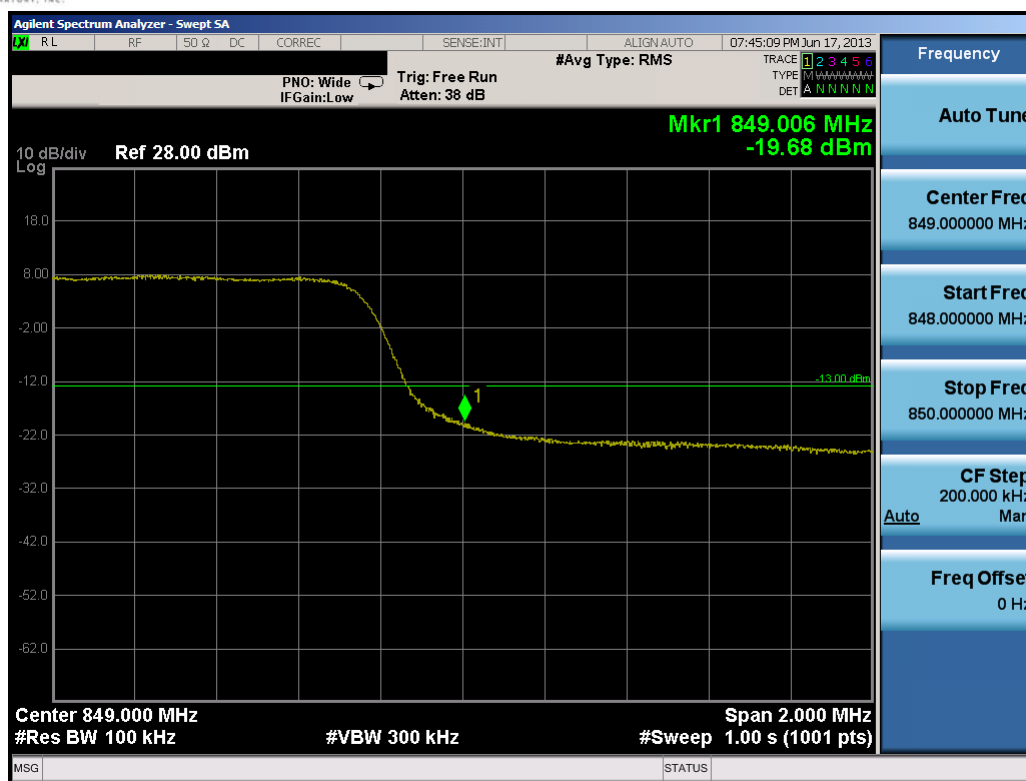
Plot 7-11. Upper Band Edge Plot (5.0MHz QPSK – RB Size 25)
