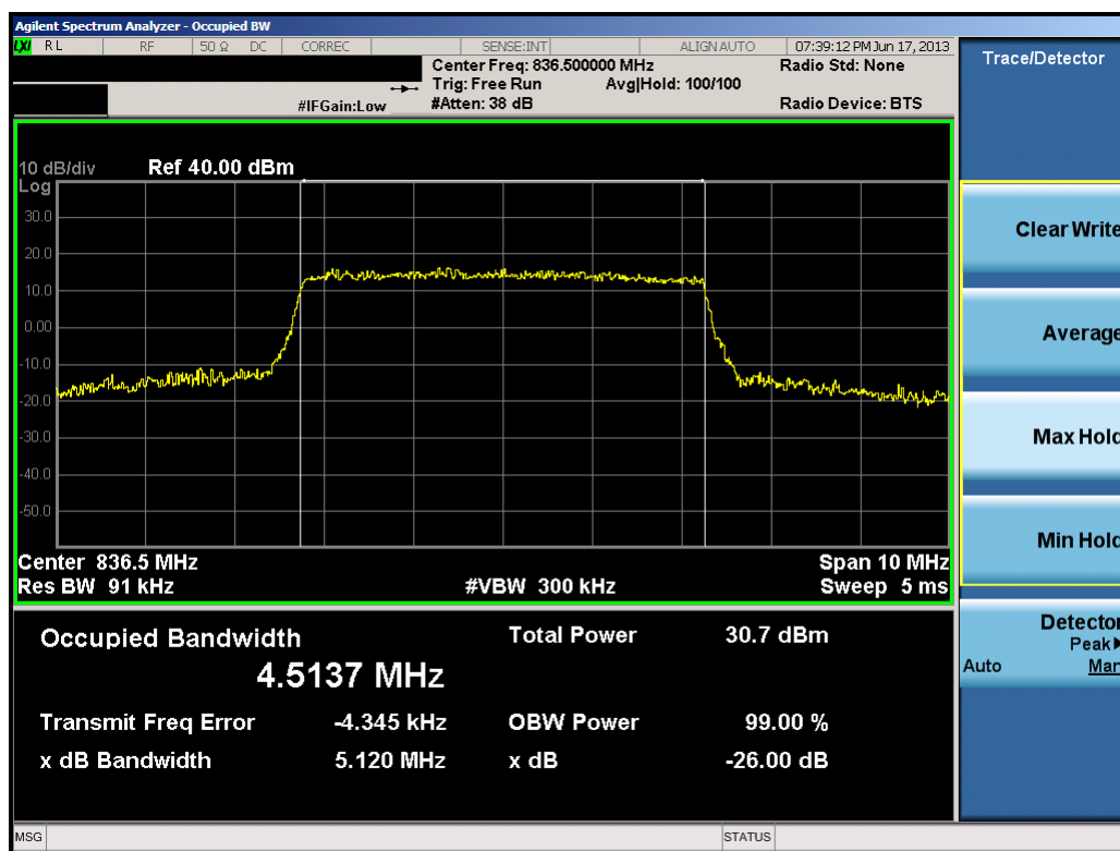
Plot 7-4. Occupied Bandwidth Plot (5.0MHz 16-QAM – RB Size 25)
