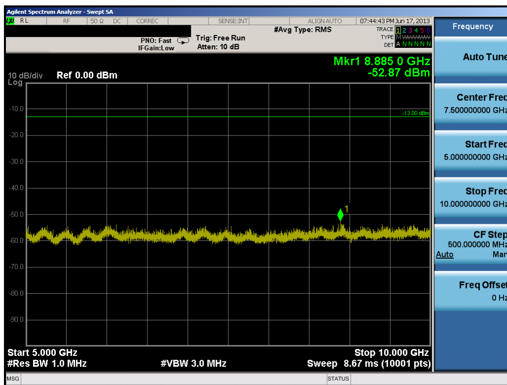
Plot 7-10. Conducted Spurious Plot (5.0MHz QPSK – RB Size 1, RB Offset 0 – High Channel)
