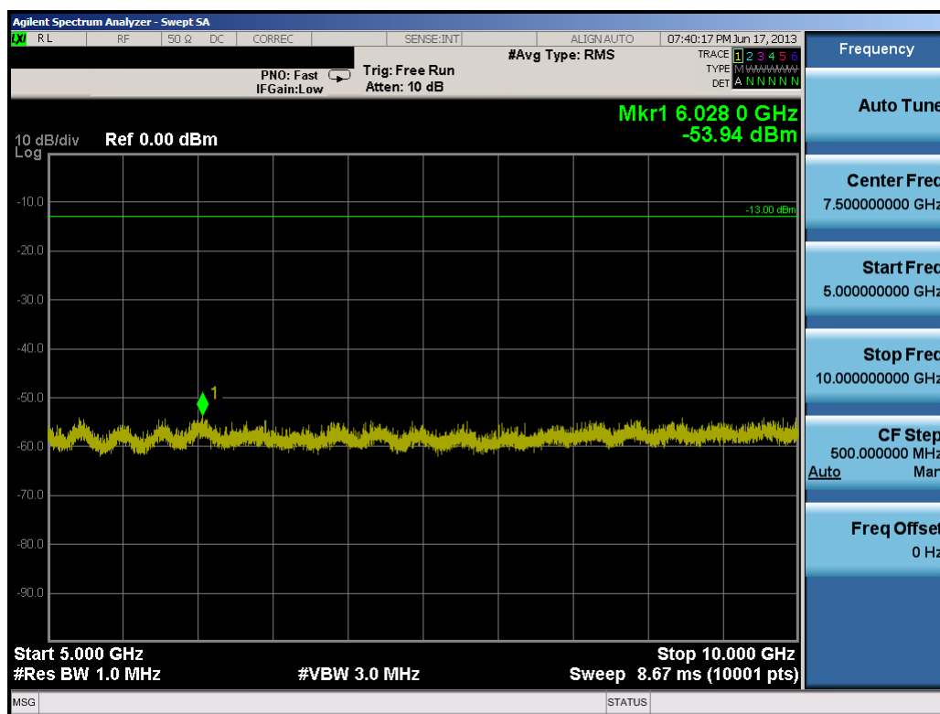
Plot 7-8. Conducted Spurious Plot (5.0MHz QPSK – RB Size 1, RB Offset 0 – Mid Channel)
