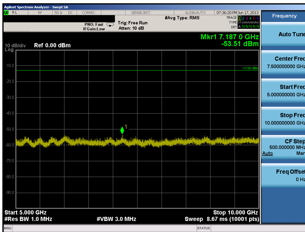
Plot 7-22. Conducted Spurious Plot (10.0MHz QPSK – RB Size 1, RB Offset 0 – High Channel)
