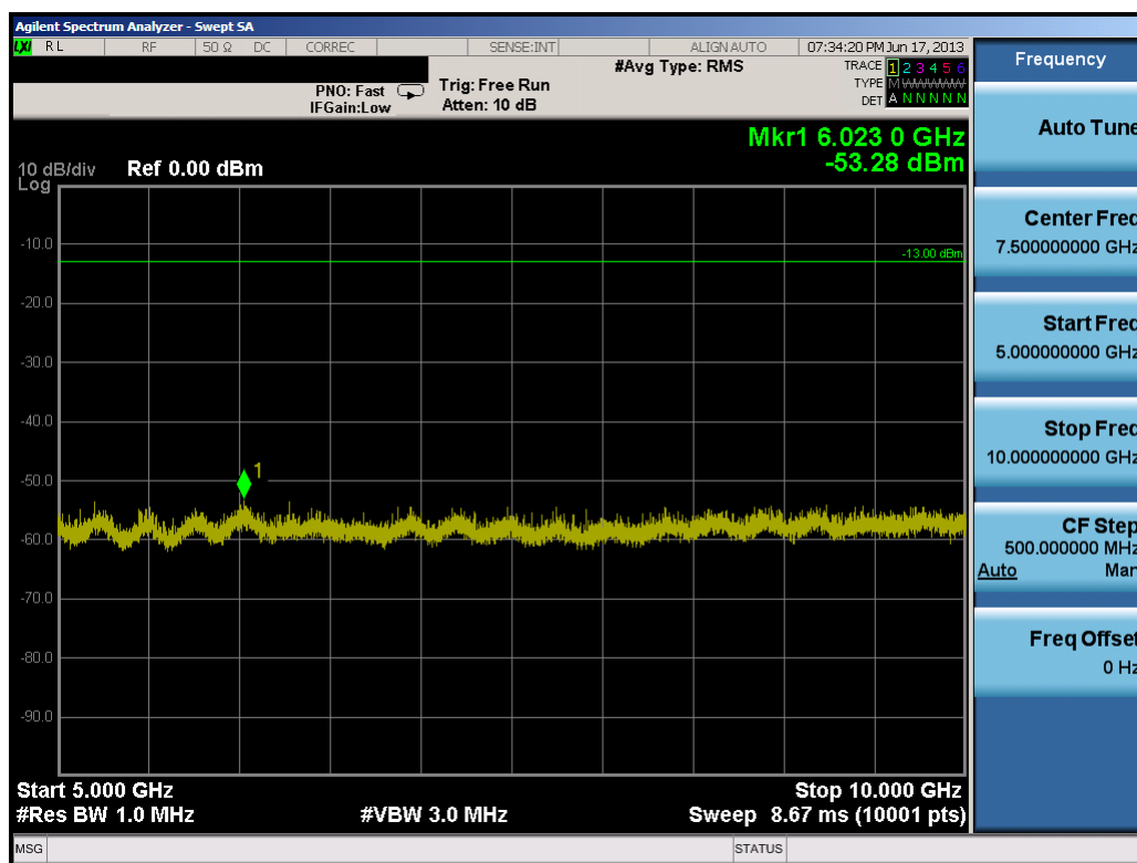
Plot 7-18. Conducted Spurious Plot (10.0MHz QPSK – RB Size 1, RB Offset 0 – Low Channel)
