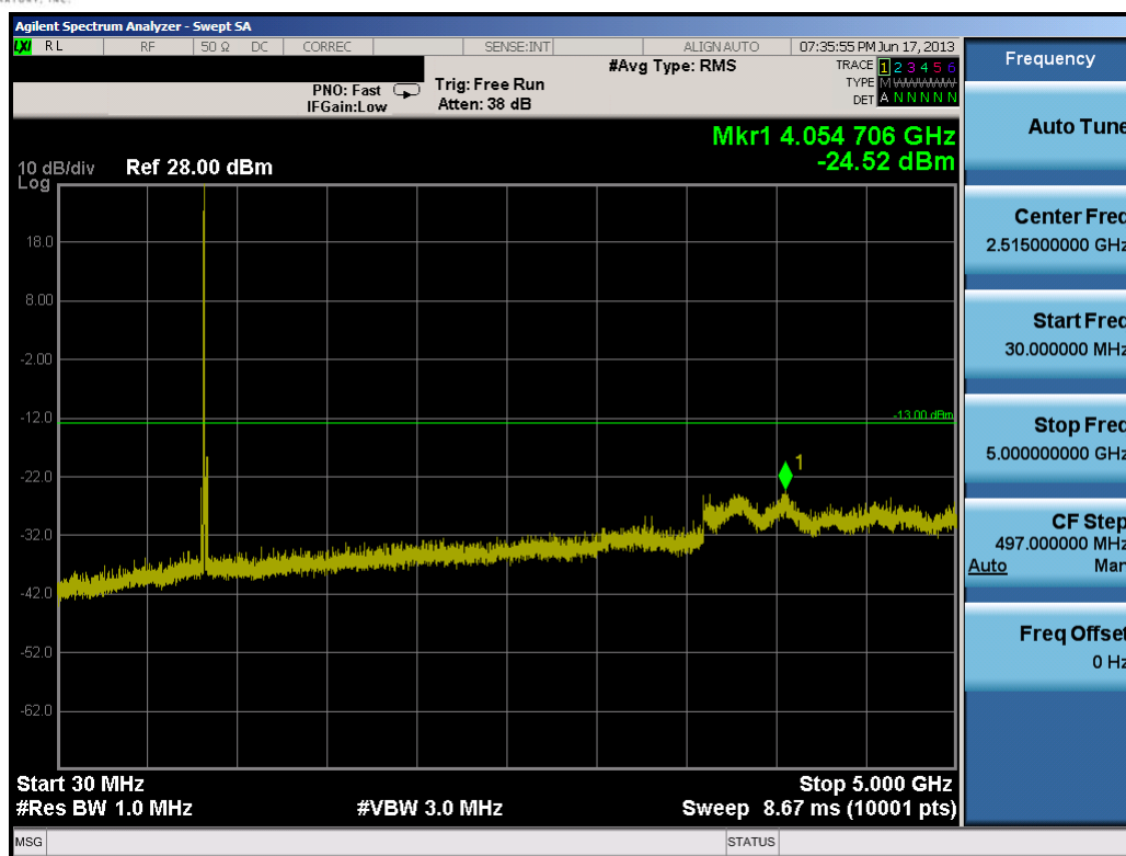
Plot 7-21. Conducted Spurious Plot (10.0MHz QPSK – RB Size 1, RB Offset 0 – High Channel)
