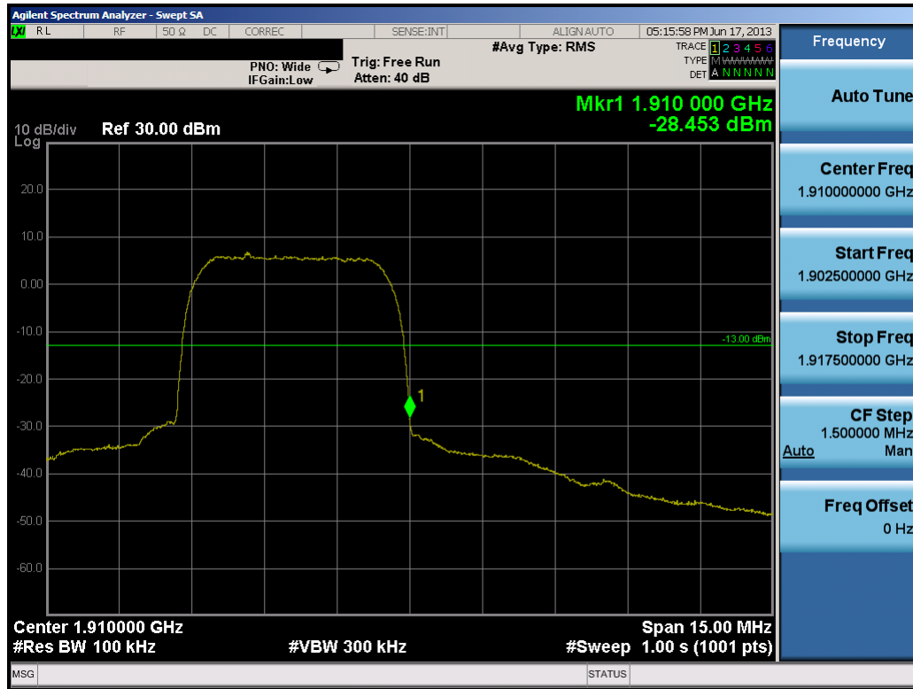
Plot 7-21. Band Edge Plot (PCS WCDMA Mode – Ch. 9538)
