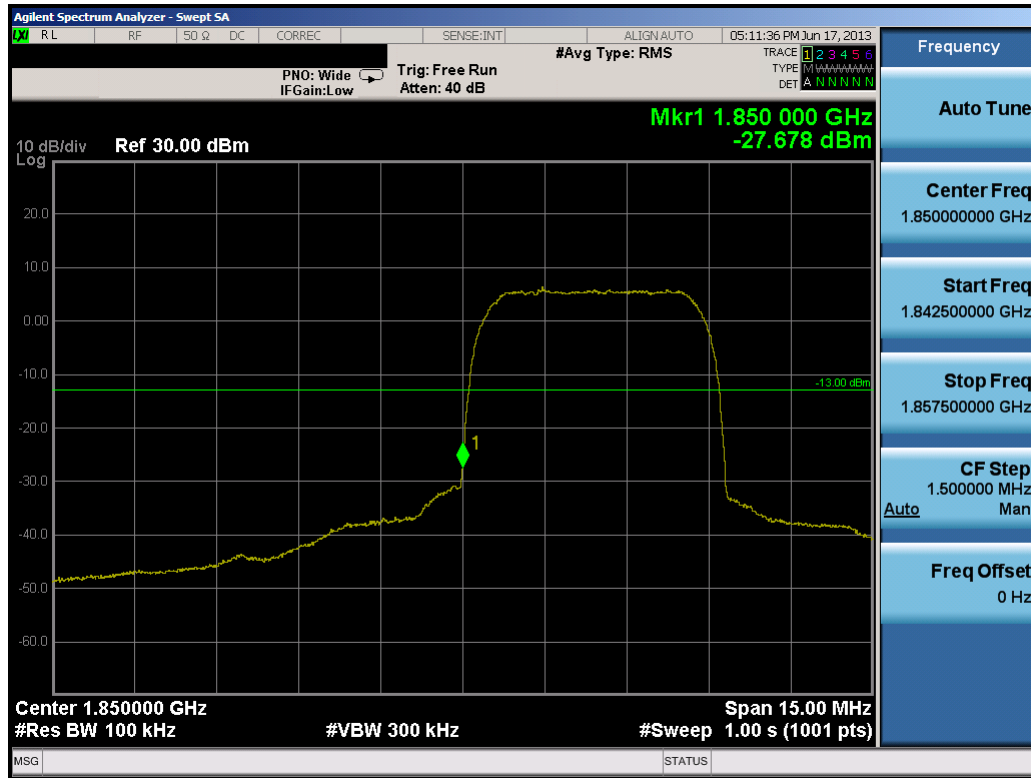
Plot 7-13. Band Edge Plot (PCS WCDMA Mode – Ch. 9262)
