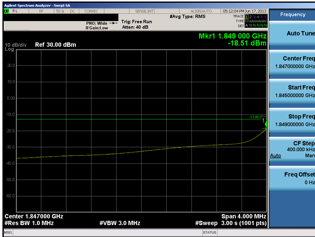
Plot 7-14. 4MHz Span Plot (PCS WCDMA Mode – Ch. 9262)
