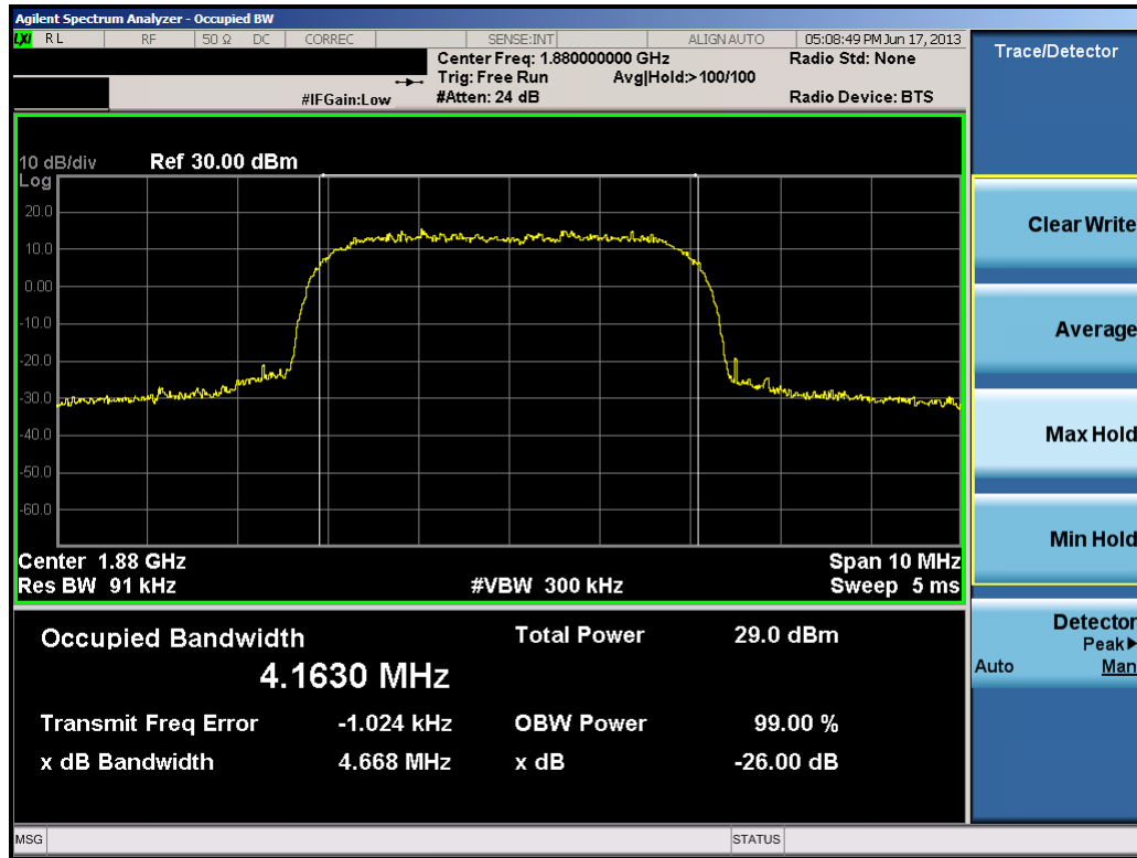
Plot 7-17. Occupied Bandwidth Plot (PCS WCDMA Mode – Ch. 9400)
