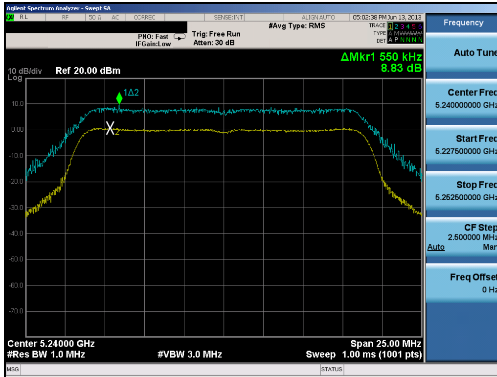
Plot 6-55. Peak Excursion Ratio Plot (20MHz BW 802.11n)
