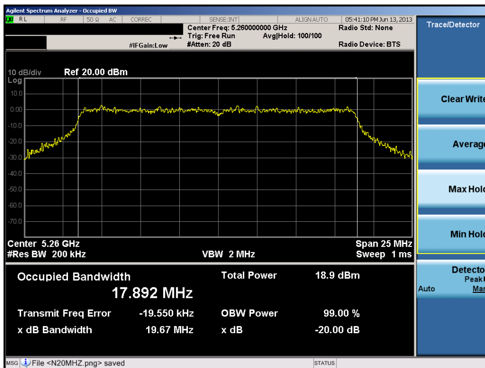
Plot 6-27. 20dB Bandwidth Plot (20MHz BW 802.11n (UNII Band 2) – Ch. 52)
