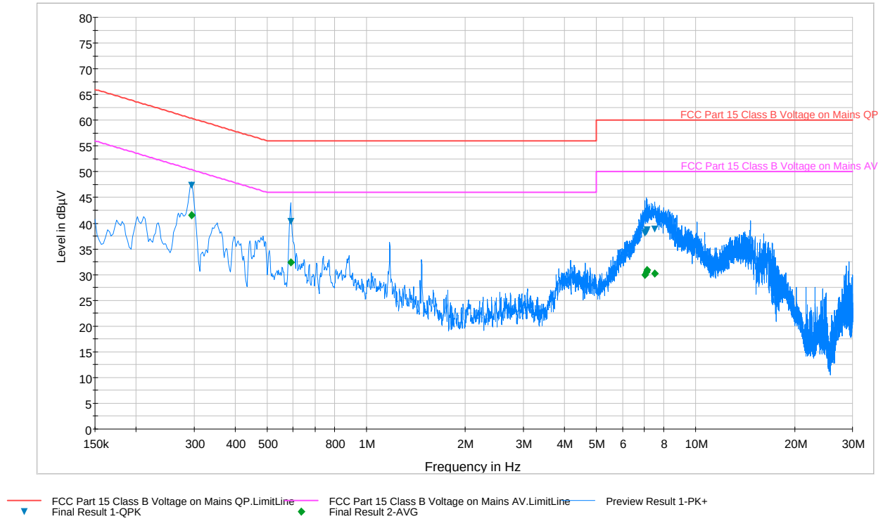
Plot 6-74. Line Conducted Plot with 802.11a UNII Band 2 (N)
