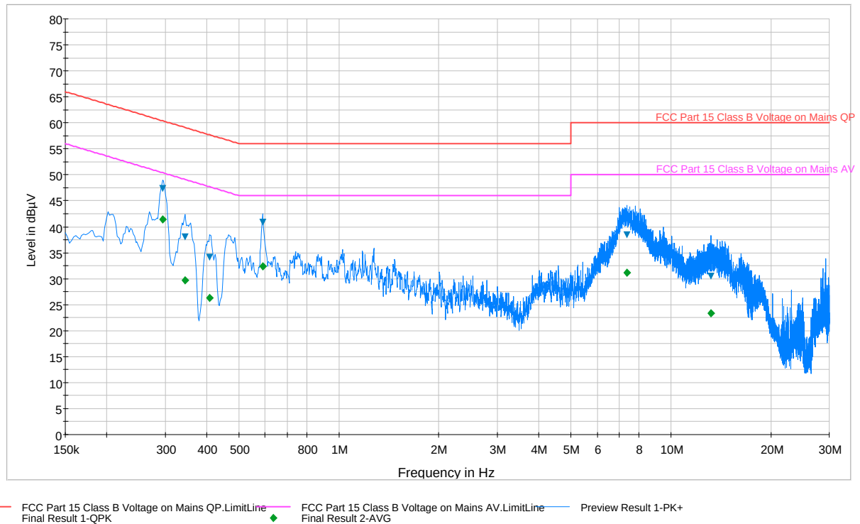
Plot 6-73. Line Conducted Plot with 802.11a UNII Band 2 (L1)
