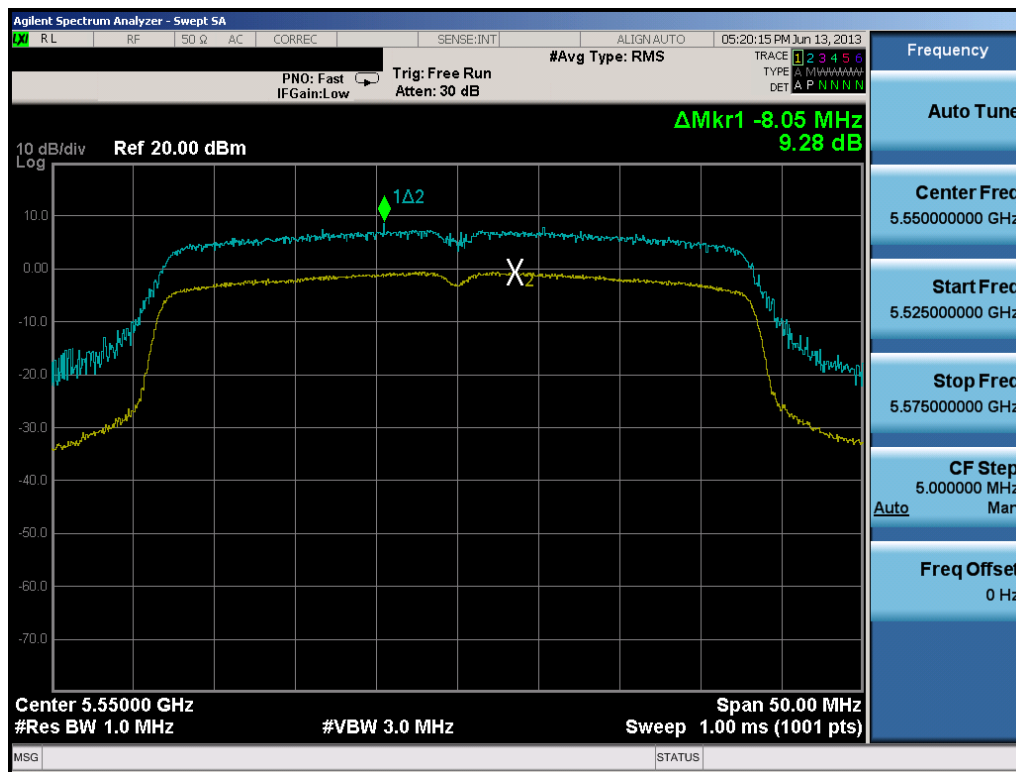
Plot 6-56. Peak Excursion Ratio Plot (40MHz BW 802.11n)
