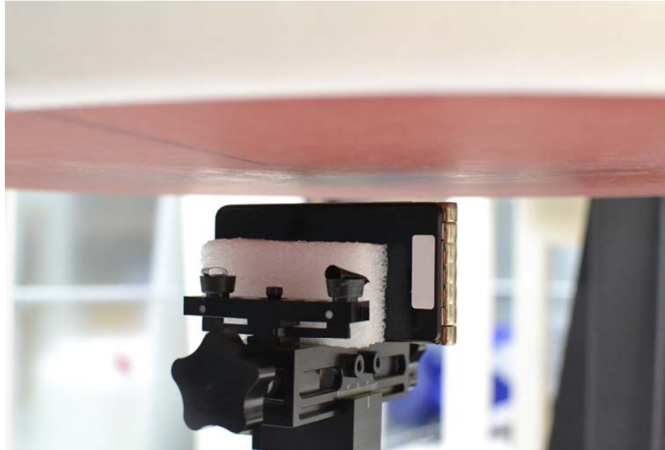
SAR Test Setup Photo 12: Left Edge at 1.0 cm
