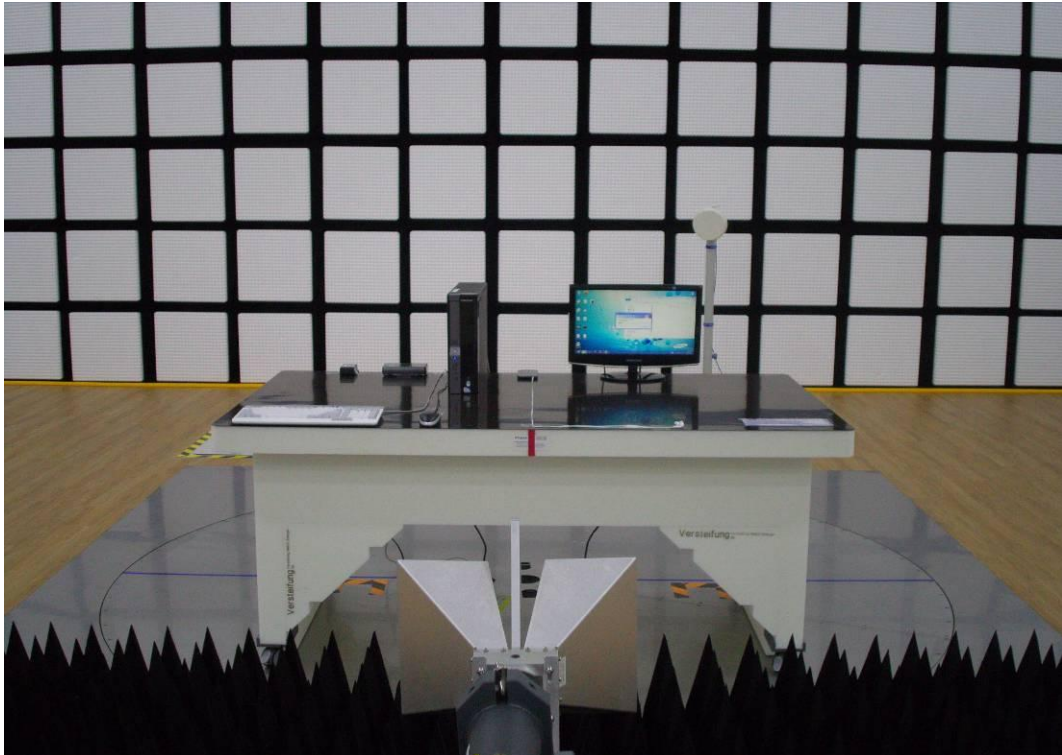
[ Radiated Disturbance for Above 1 GHz – Front ]
