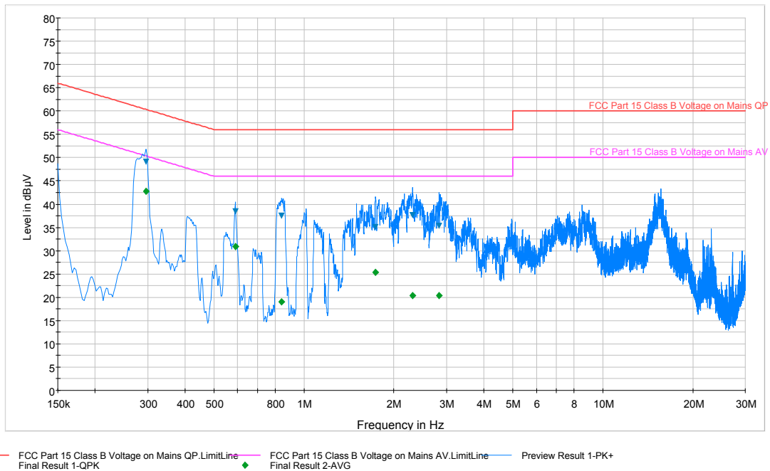
Plot 6-43. Line-Conducted Test Plot (L1)
