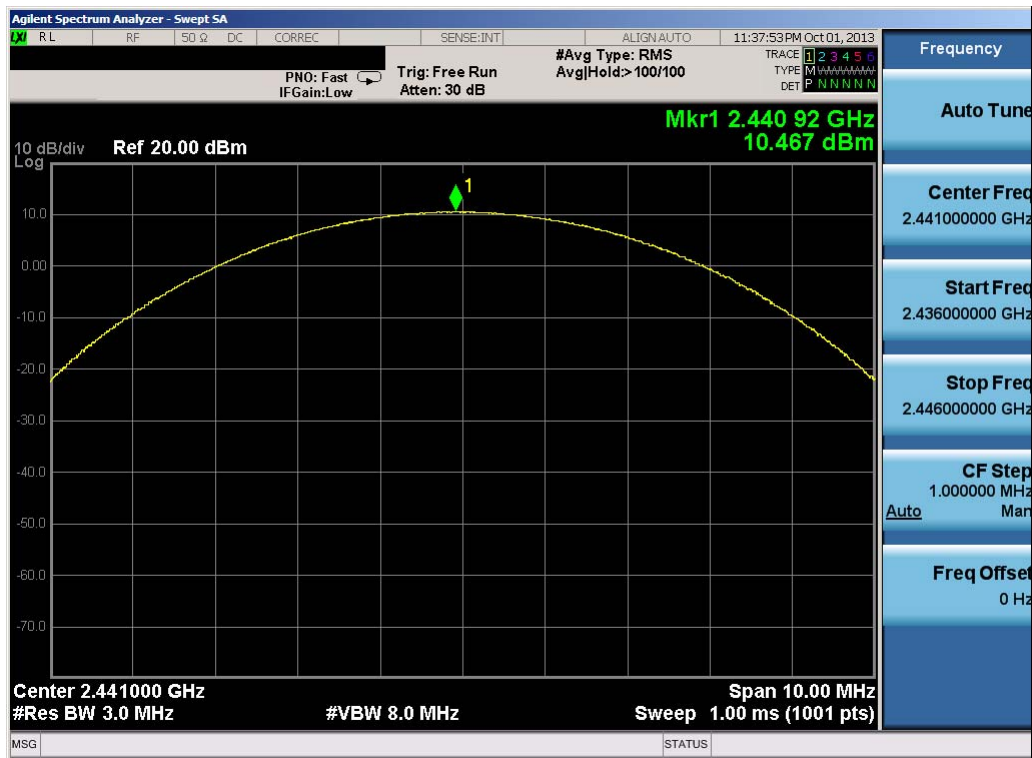
Plot 6-17. Peak Conducted Power (3Mbps – Ch. 39)
