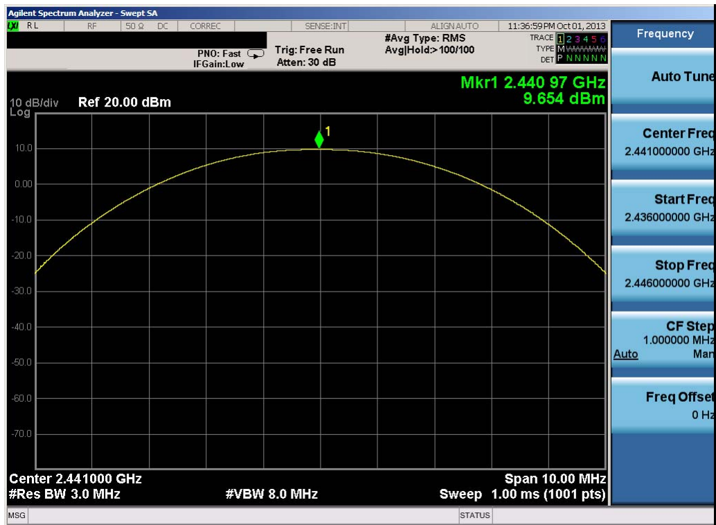
Plot 6-11. Peak Conducted Power (1Mbps - Ch. 39)
