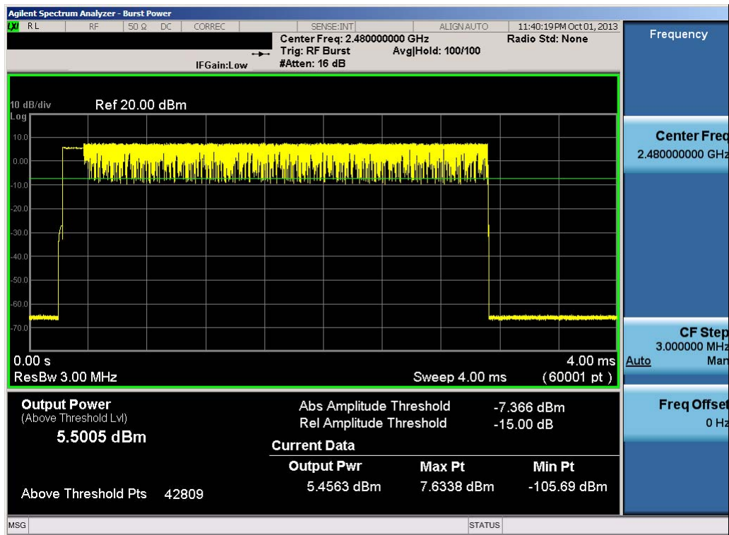
Plot 6-27. Average Conducted Power (3Mbps – Ch. 78)
