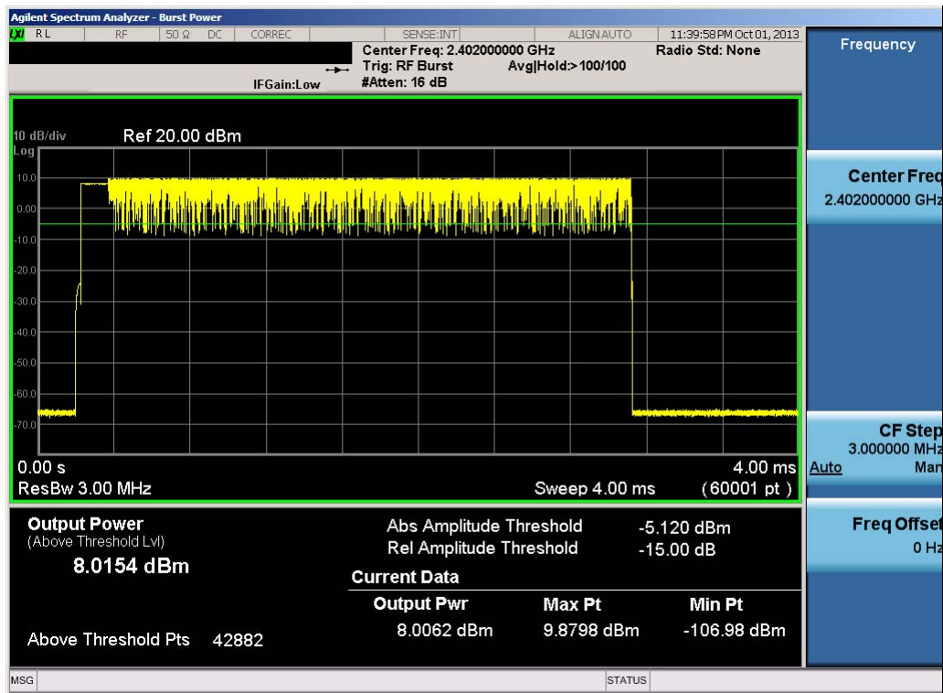
Plot 6-25. Average Conducted Power (3Mbps – Ch. 0)
