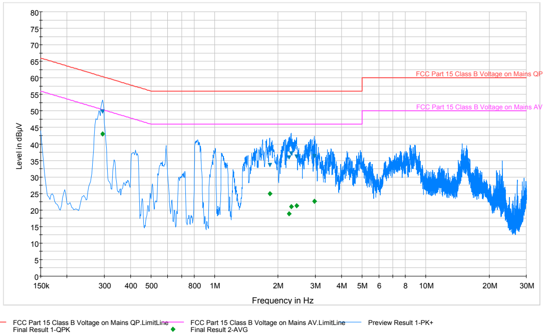
Plot 6-44. Line-Conducted Test Plot (N)
