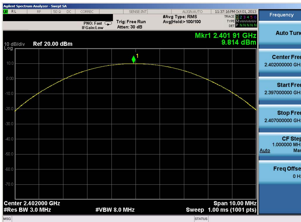
Plot 6-13. Peak Conducted Power (2Mbps – Ch. 0)
