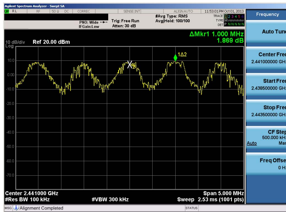
Plot 6-32. Channel Spacing Plot (Bluetooth)
