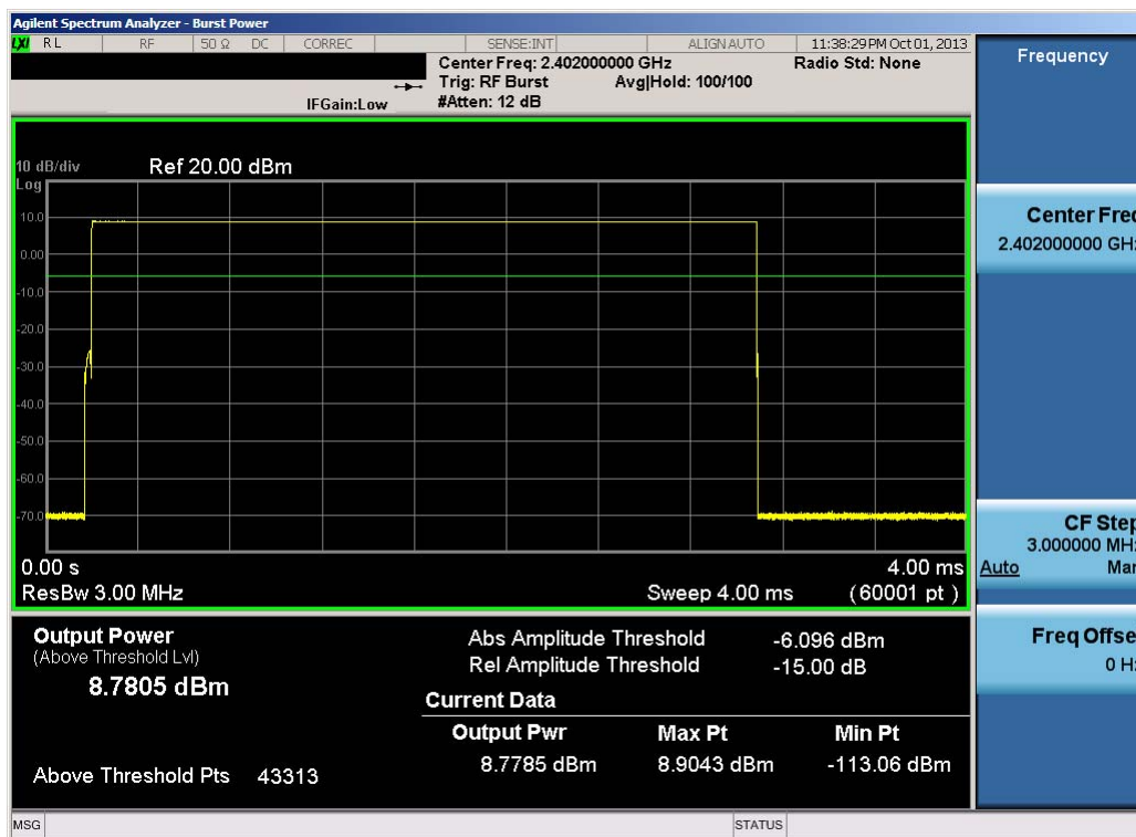
Plot 6-19. Average Conducted Power (1Mbps – Ch. 0)
