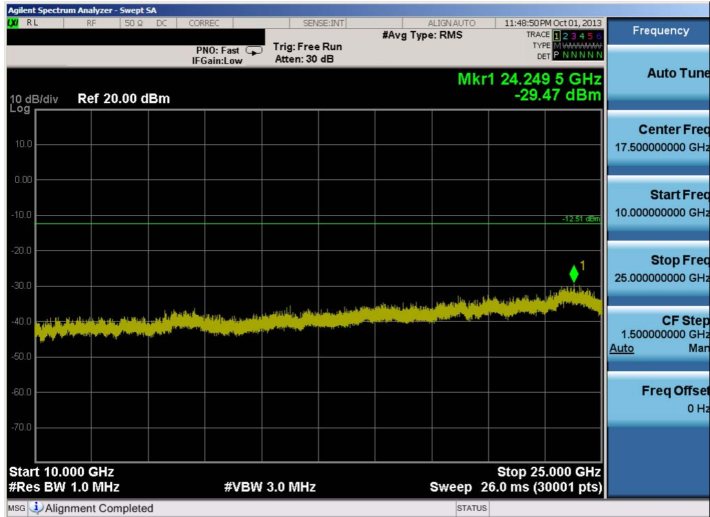
Plot 6-37. Conducted Spurious Plot (Bluetooth, 3Mbps – Ch. 0)
