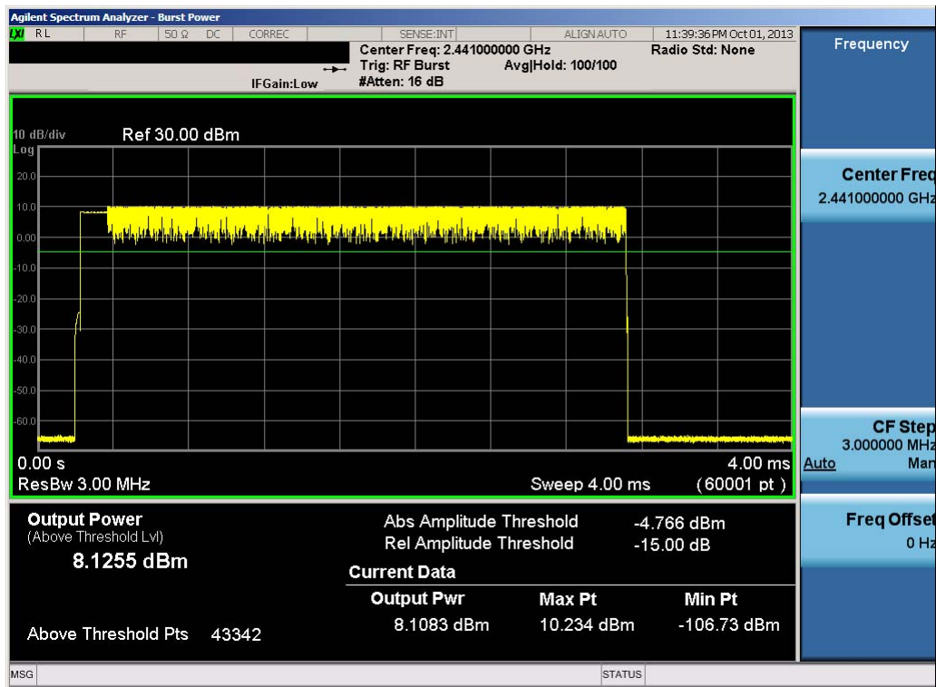
Plot 6-23. Average Conducted Power (2Mbps - Ch. 39)
