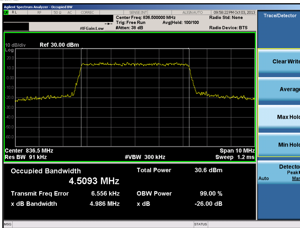
Plot 7-2. Occupied Bandwidth Plot (5.0MHz QPSK – RB Size 25)
