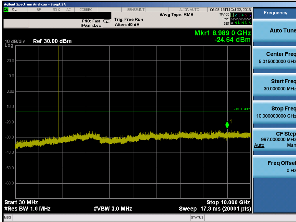
Plot 6-3. Conducted Spurious Plot (PCS GSM Mode – Ch. 512)
