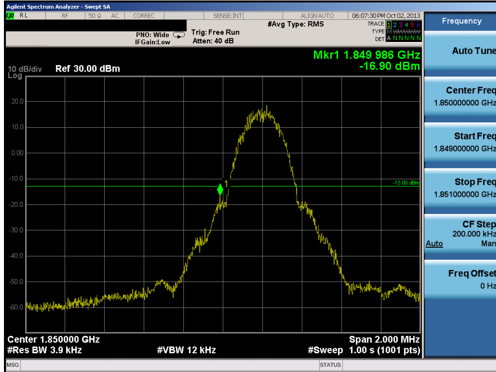
Plot 6-15. Band Edge Plot (PCS GSM Mode – Ch. 512)
