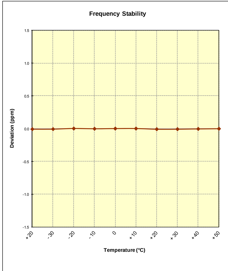
Figure 6-8. Frequency Stability Graph (PCS WCDMA Mode – Ch. 9400)
