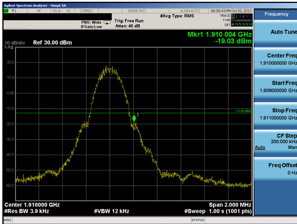
Plot 6-16. Band Edge Plot (PCS GSM Mode – Ch. 810)
