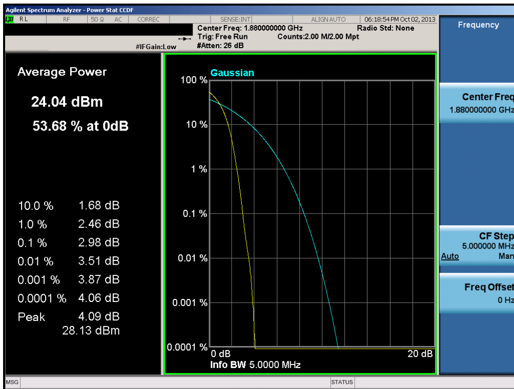
Plot 6-22. Peak-Average Ratio Plot (PCS WCDMA Mode – Ch. 9400)
