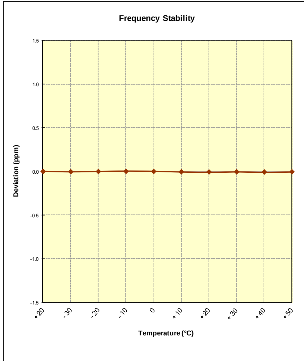
Figure 6-7. Frequency Stability Graph (PCS GSM Mode – Ch. 661)
