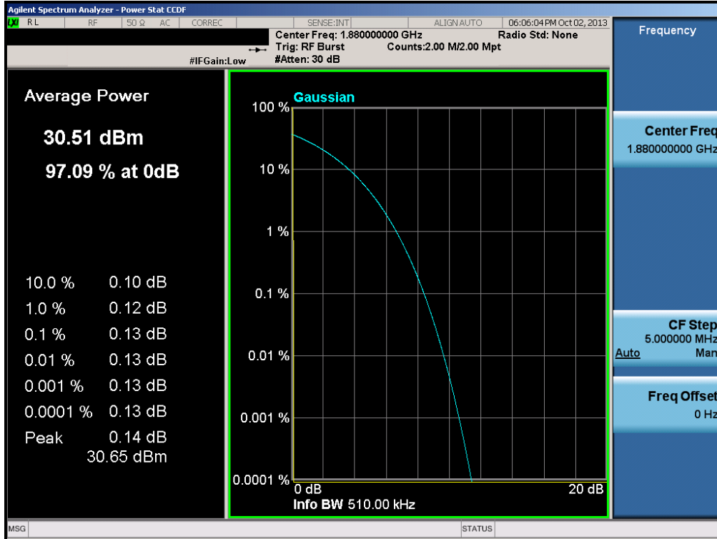
Plot 6-21. Peak-Average Ratio Plot (PCS GSM Mode – Ch. 661)
