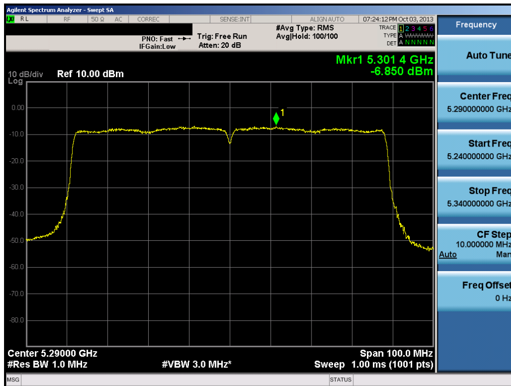
Plot 6-49. Peak Power Spectral Density Plot (80MHz BW 802.11ac (UNII Band 2) – Ch. 58)
