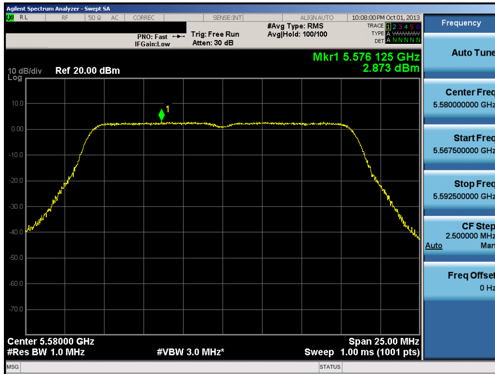
Plot 6-51. Peak Power Spectral Density Plot (802.11a (UNII Band 3) – Ch. 116)
