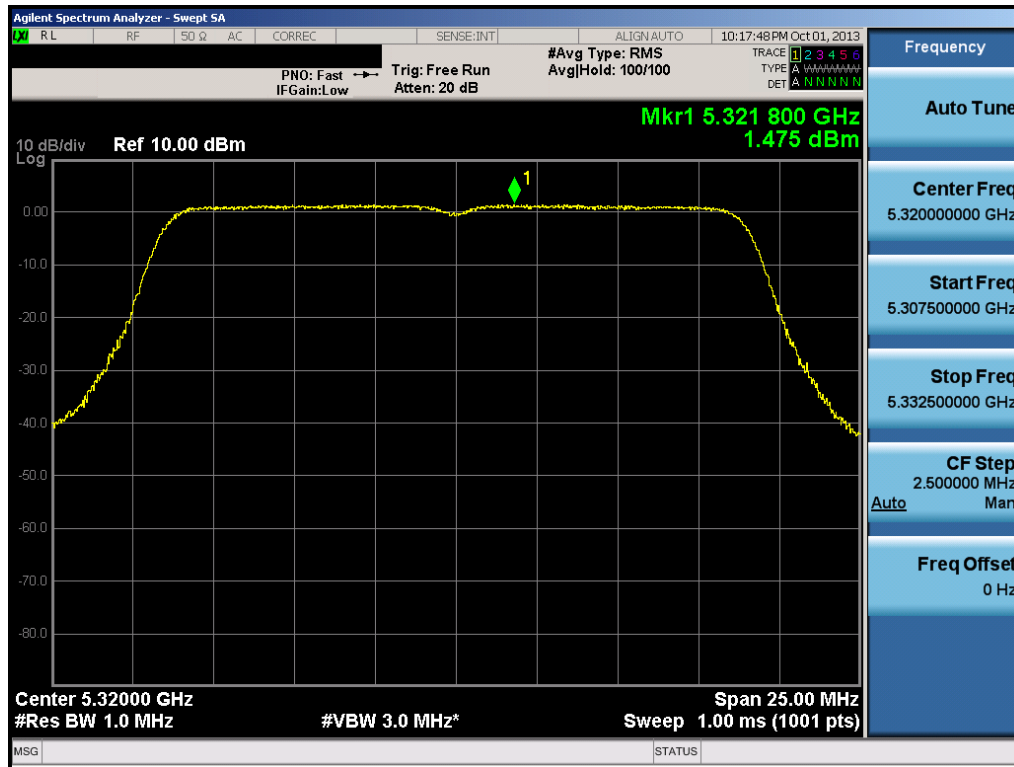
Plot 6-46. Peak Power Spectral Density Plot (20MHz BW 802.11n (UNII Band 2) – Ch. 64)
