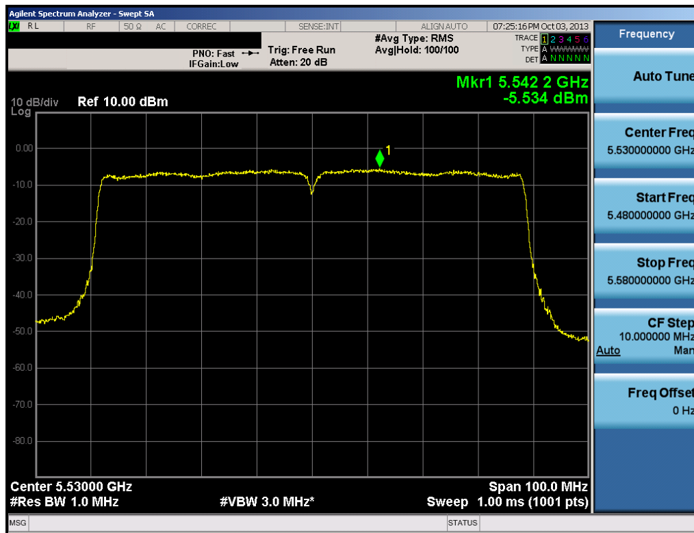
Plot 6-59. Peak Power Spectral Density Plot (80MHz BW 802.11ac (UNII Band 3) – Ch. 106)
