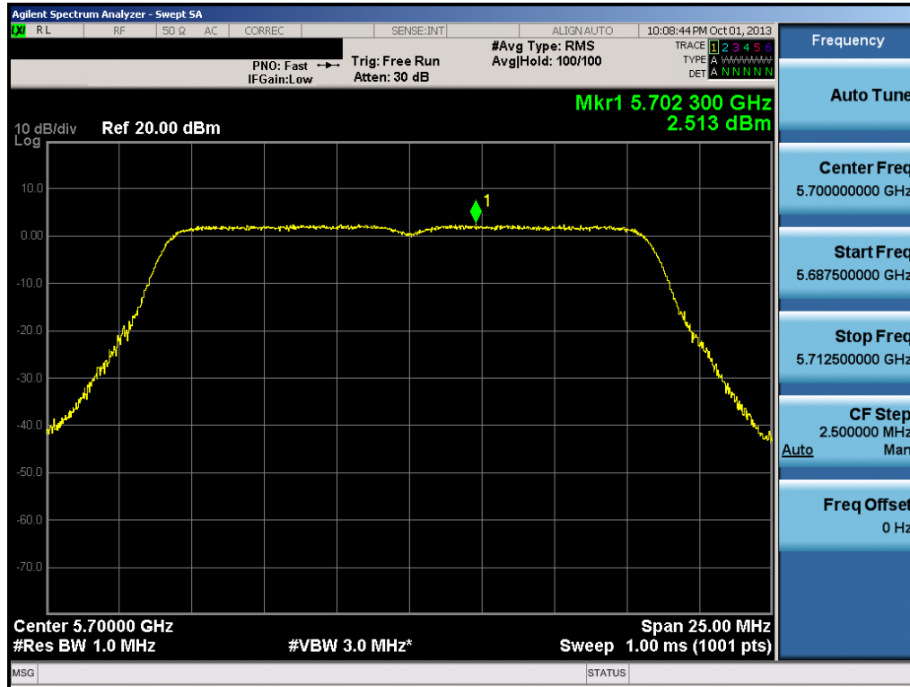
Plot 6-52. Peak Power Spectral Density Plot (802.11a (UNII Band 3) – Ch. 140)
