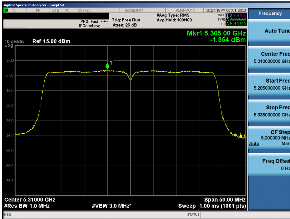
Plot 6-48. Peak Power Spectral Density Plot (40MHz BW 802.11n (UNII Band 2) – Ch. 62)
