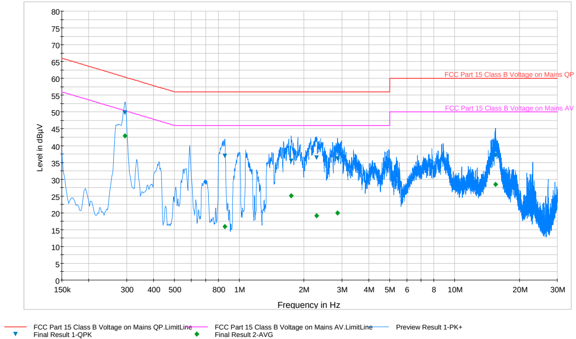
Plot 6-86. Line Conducted Plot with 802.11a UNII Band 2 (L1)
