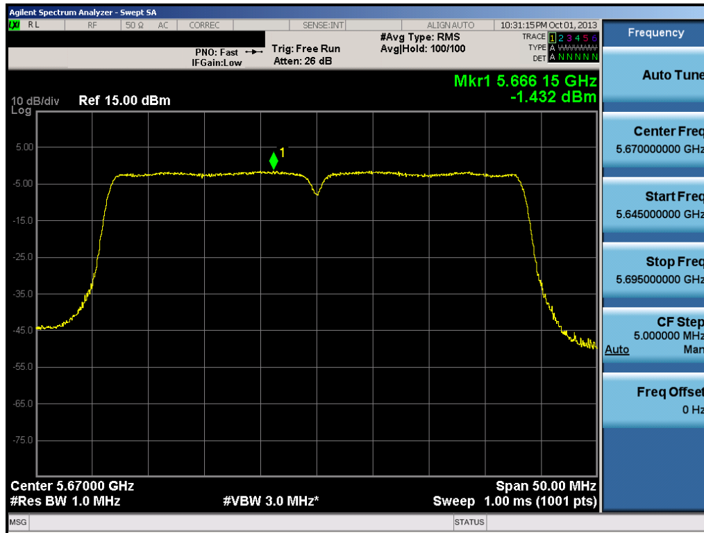
Plot 6-58. Peak Power Spectral Density Plot (40MHz BW 802.11n (UNII Band 3) – Ch. 134)
