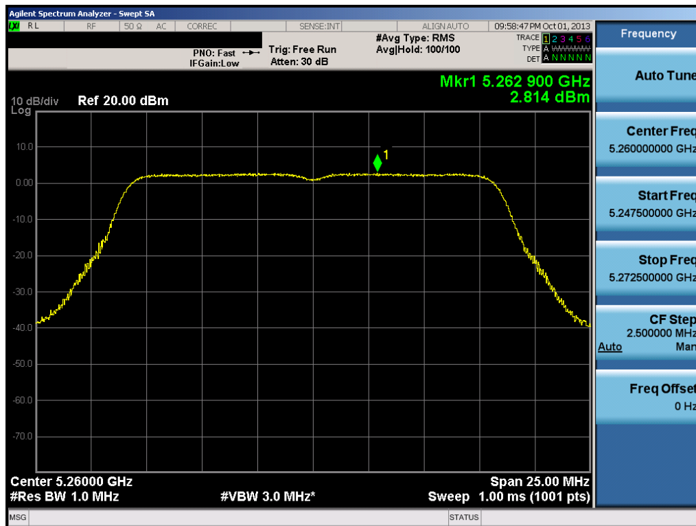
Plot 6-41. Peak Power Spectral Density Plot (802.11a (UNII Band 2) – Ch. 52)
