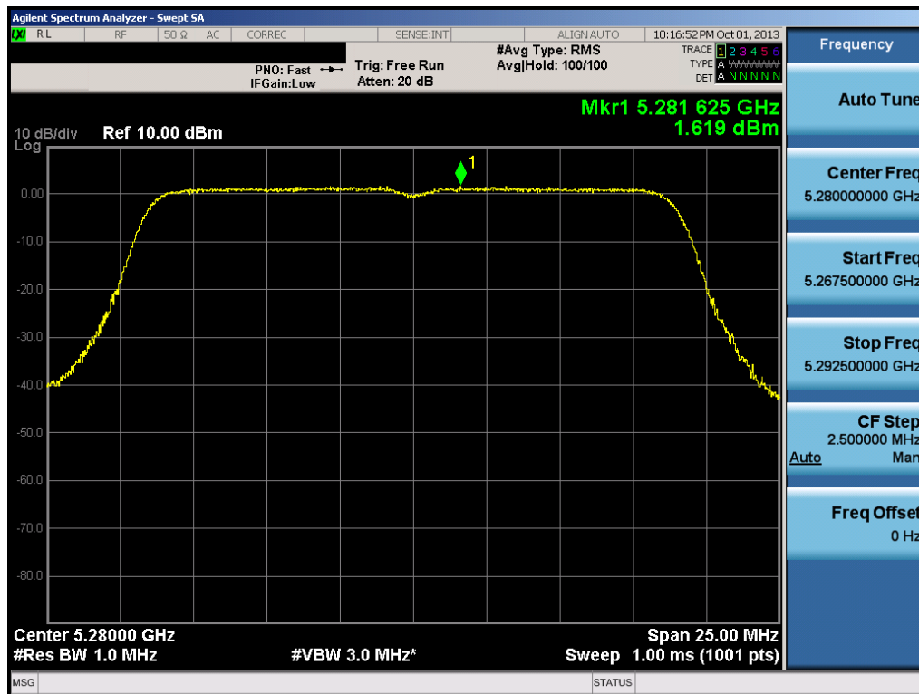
Plot 6-45. Peak Power Spectral Density Plot (20MHz BW 802.11n (UNII Band 2) – Ch. 56)
