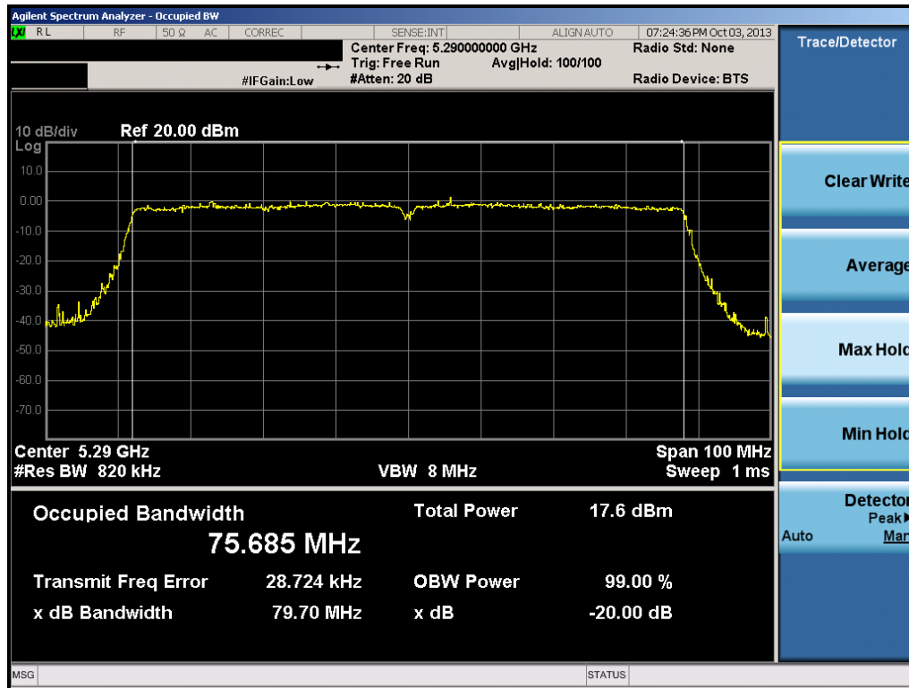
Plot 6-31. 20dB Bandwidth Plot (80MHz BW 802.11ac (UNII Band 2) – Ch. 58)
