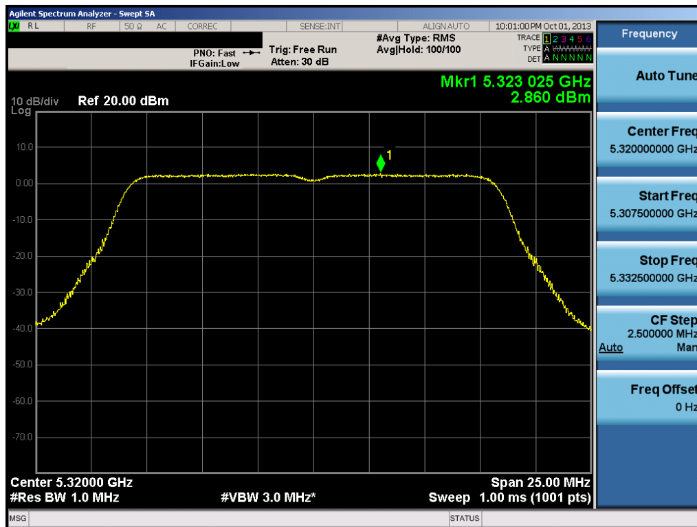
Plot 6-43. Peak Power Spectral Density Plot (802.11a (UNII Band 2) – Ch. 64)
