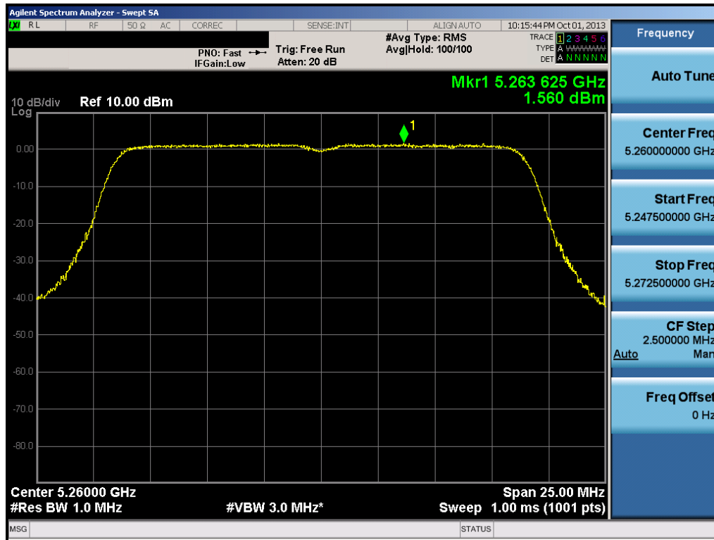
Plot 6-44. Peak Power Spectral Density Plot (20MHz BW 802.11n (UNII Band 2) – Ch. 52)
