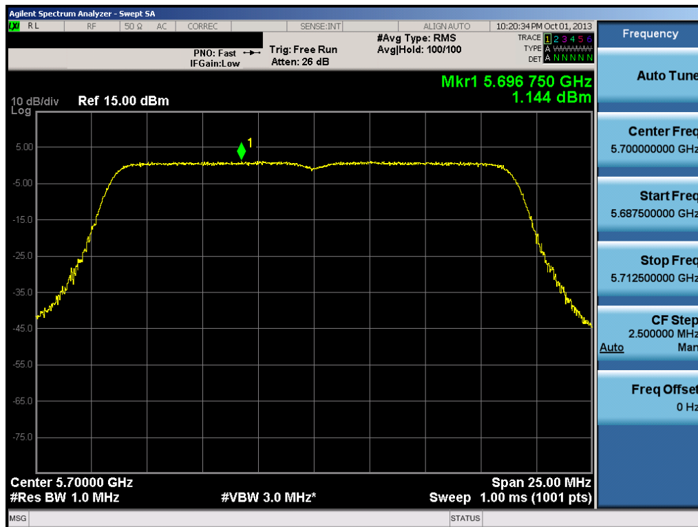
Plot 6-55. Peak Power Spectral Density Plot (20MHz BW 802.11n (UNII Band 3) – Ch. 140)
