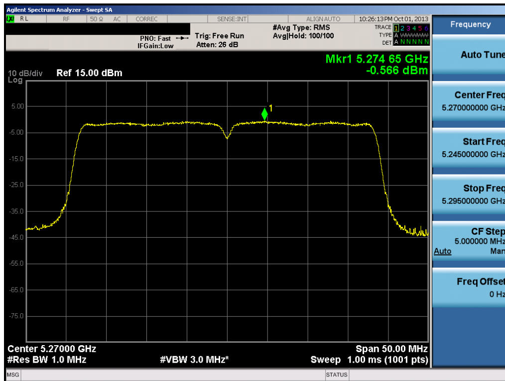
Plot 6-47. Peak Power Spectral Density Plot (40MHz BW 802.11n (UNII Band 2) – Ch. 54)
