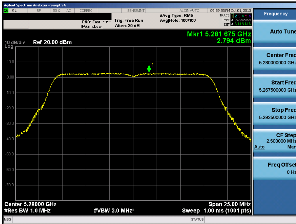
Plot 6-42. Peak Power Spectral Density Plot (802.11a (UNII Band 2) – Ch. 56)
