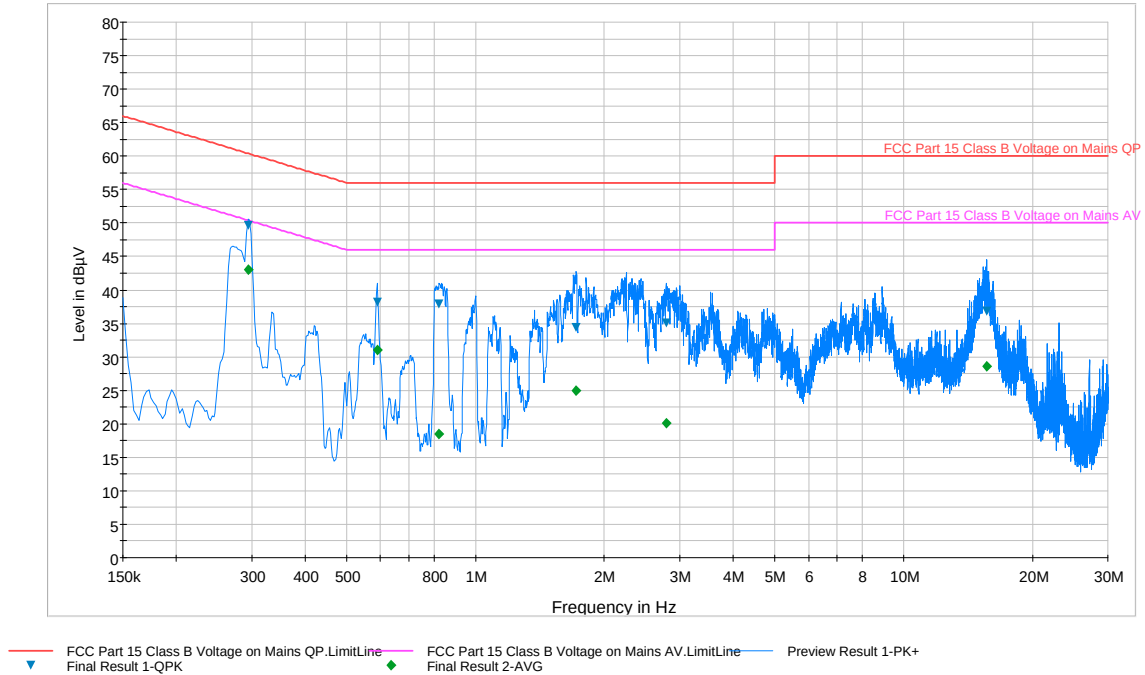
Plot 6-88. Line Conducted Plot with 802.11a UNII Band 3 (L1)
