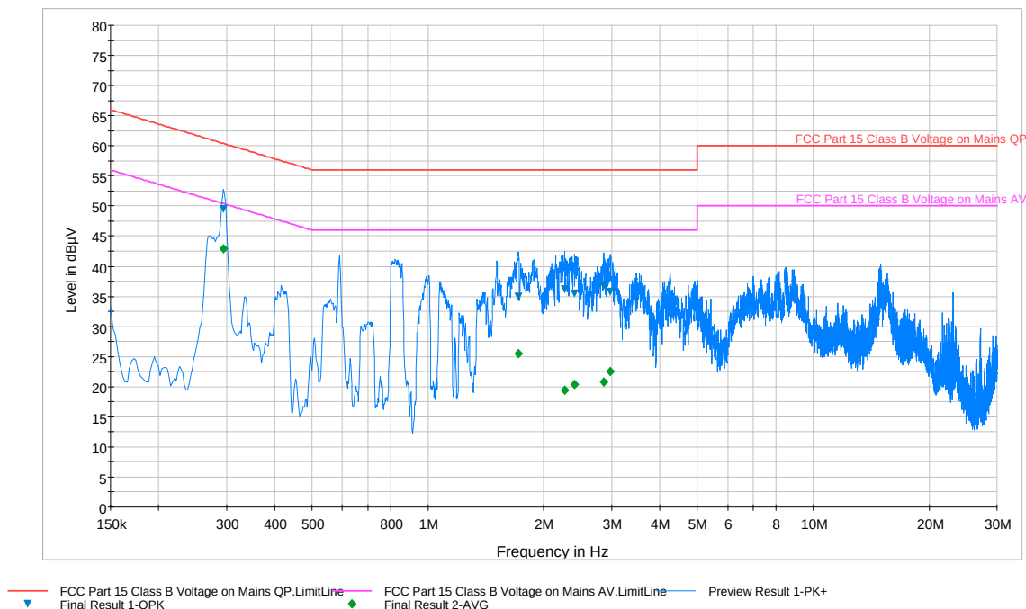
Plot 6-87. Line Conducted Plot with 802.11a UNII Band 2 (N)
