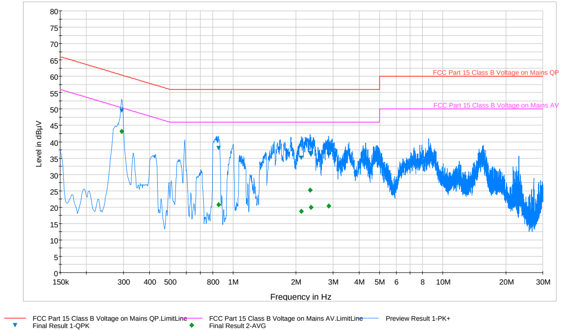
Plot 6-89. Line Conducted Plot with 802.11a UNII Band 3 (N)
