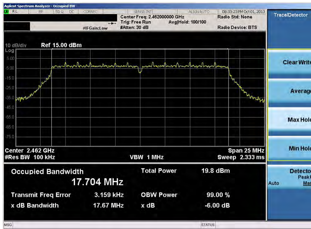
Plot 6-9. 6dB Bandwidth Plot (802.11n (2.4GHz) – Ch. 11)
