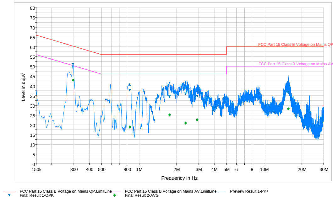
Plot 6-67. Line Conducted Plot with 802.11b (L1)
