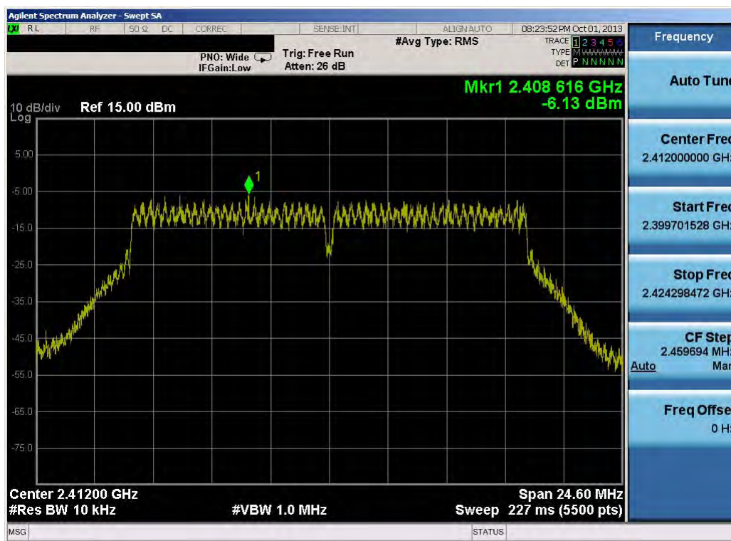
Plot 6-22. Power Spectral Density Plot (802.11g – Ch. 1)
