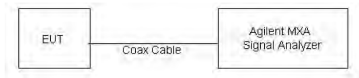
Figure 6-3. Test Instrument & Measurement Setup for Signal Analyzer Measurements
