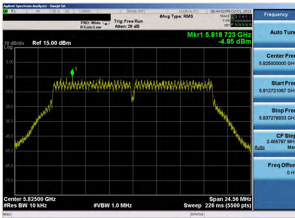
Plot 6-30. Power Spectral Density Plot (802.11a - Ch. 165)
