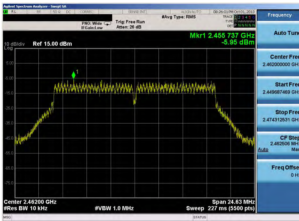
Plot 6-24. Power Spectral Density Plot (802.11g – Ch. 11)
