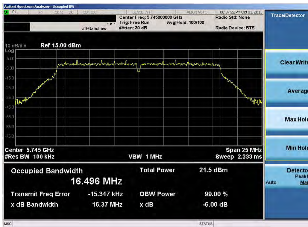
Plot 6-10. 6dB Bandwidth Plot (802.11a – Ch. 149)
