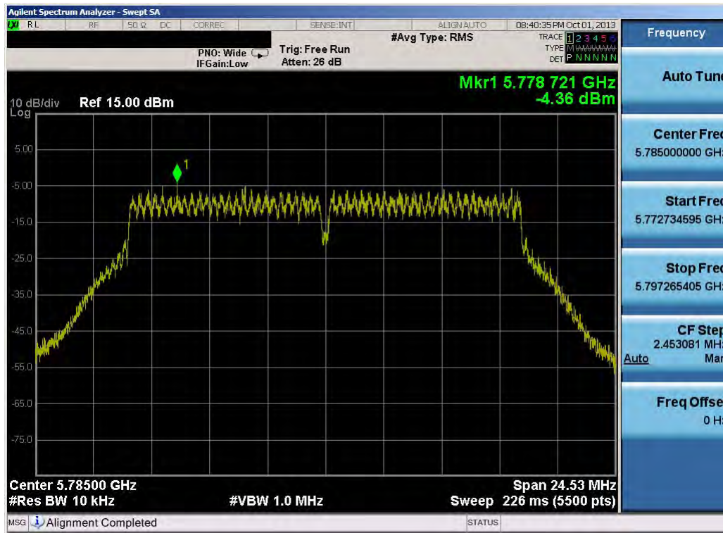
Plot 6-29. Power Spectral Density Plot (802.11a - Ch. 157)
