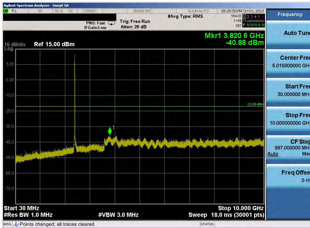
Plot 6-51. Conducted Spurious Plot (802.11b – Ch. 1)
