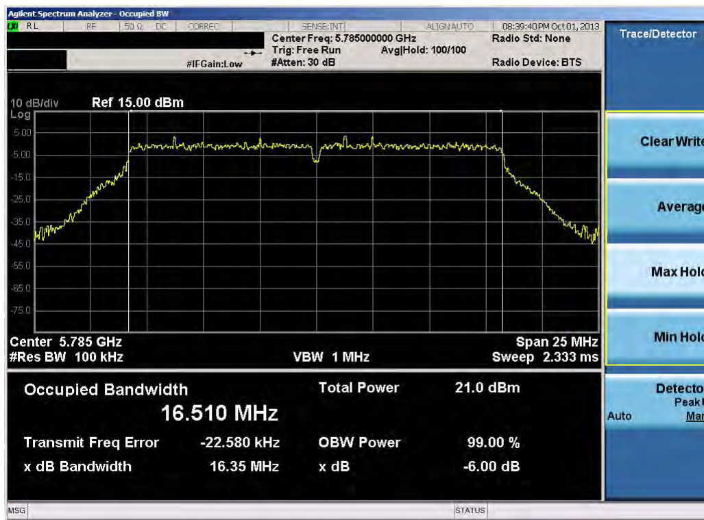
Plot 6-11. 6dB Bandwidth Plot (802.11a – Ch. 157)
