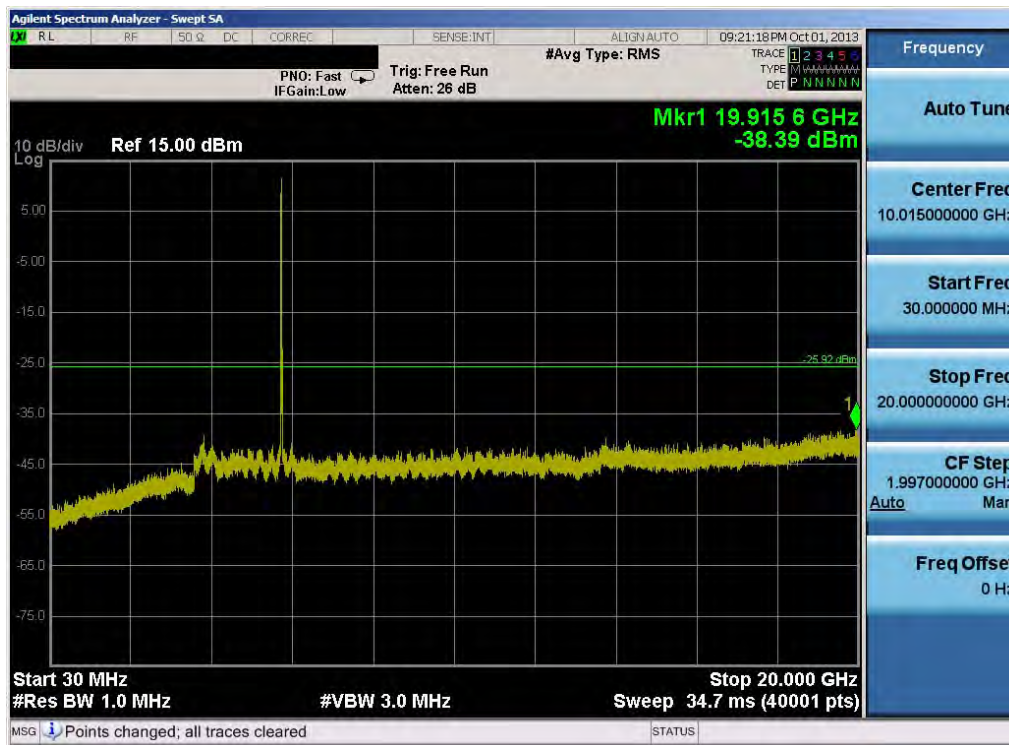
Plot 6-57. Conducted Spurious Plot (802.11a – Ch. 149)
