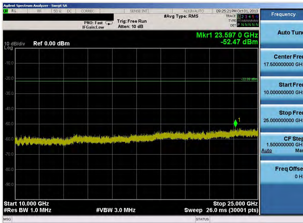
Plot 6-52. Conducted Spurious Plot (802.11b – Ch. 1)
