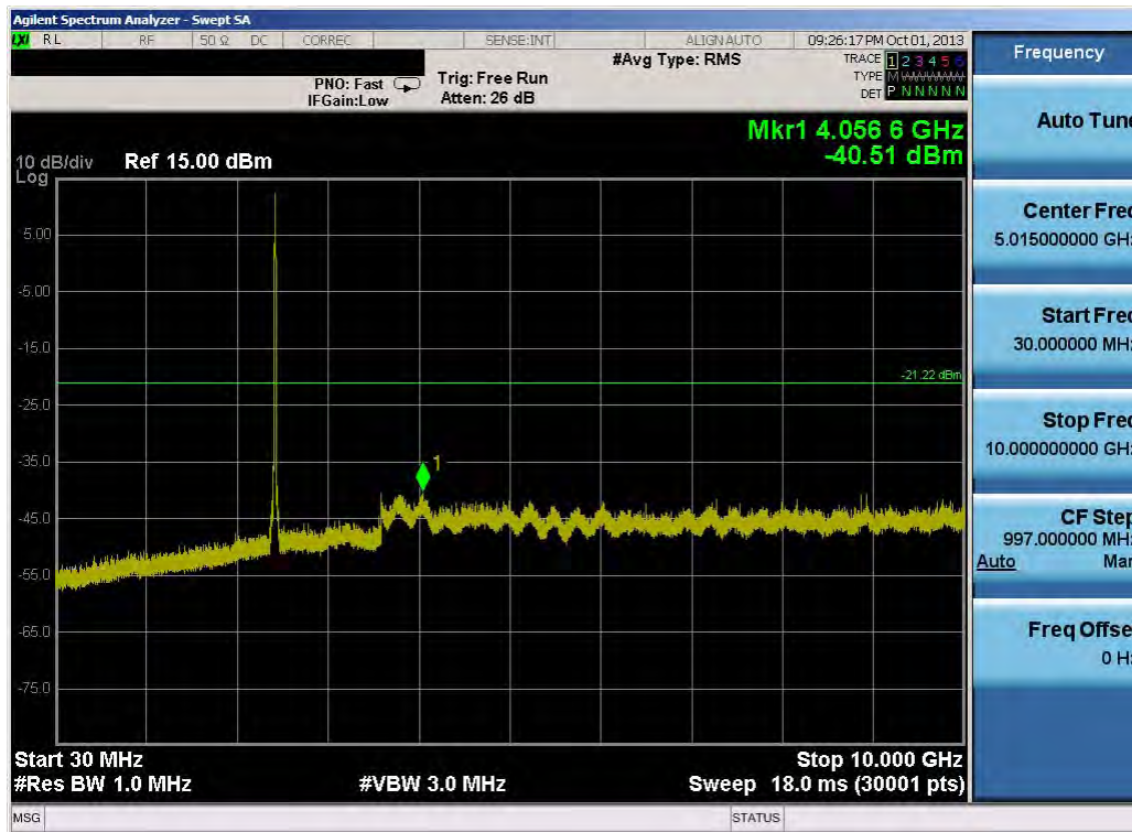
Plot 6-53. Conducted Spurious Plot (802.11b – Ch. 6)
