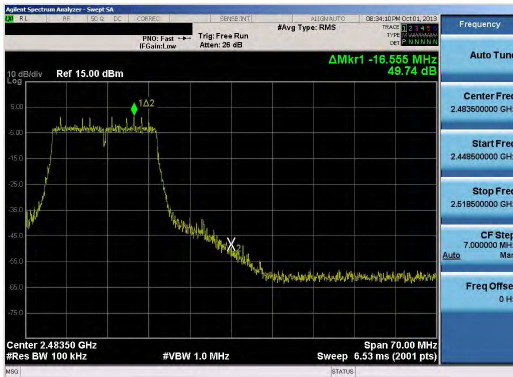
Plot 6-42. Band Edge Plot (802.11n (2.4GHz) – Ch. 11)
