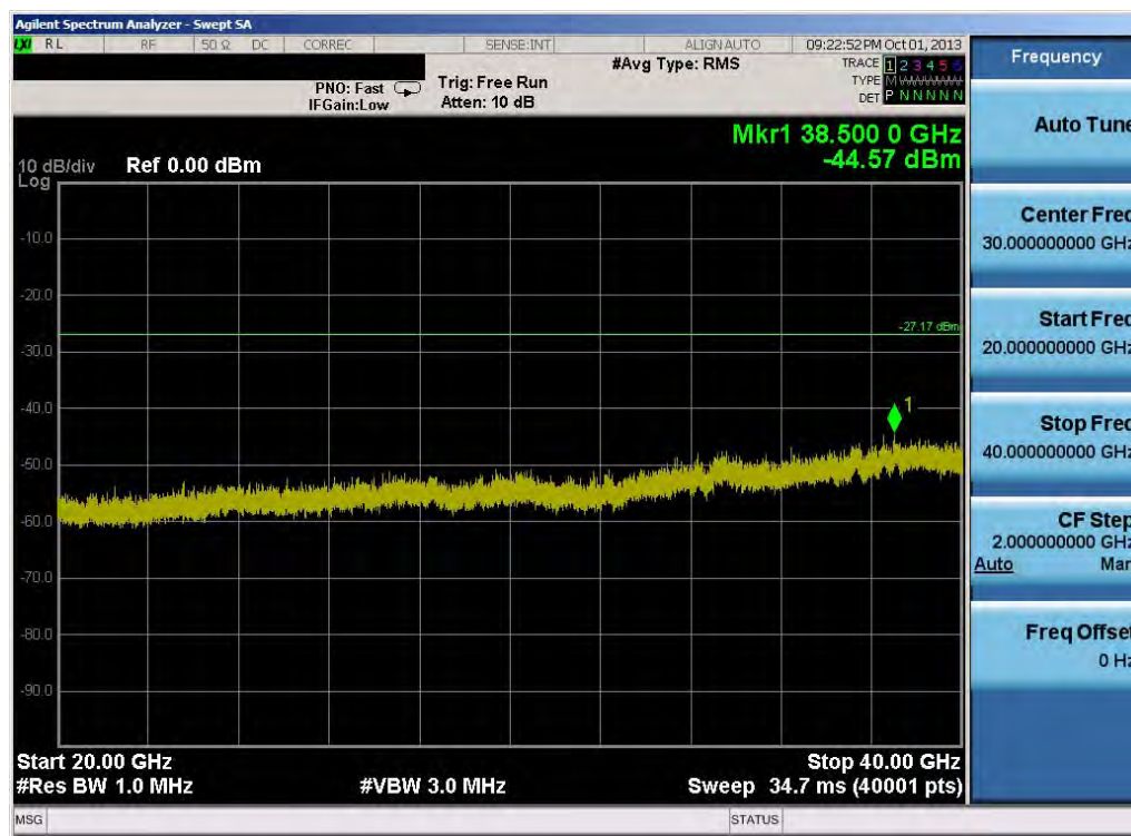
Plot 6-60. Conducted Spurious Plot (802.11a – Ch. 157)
