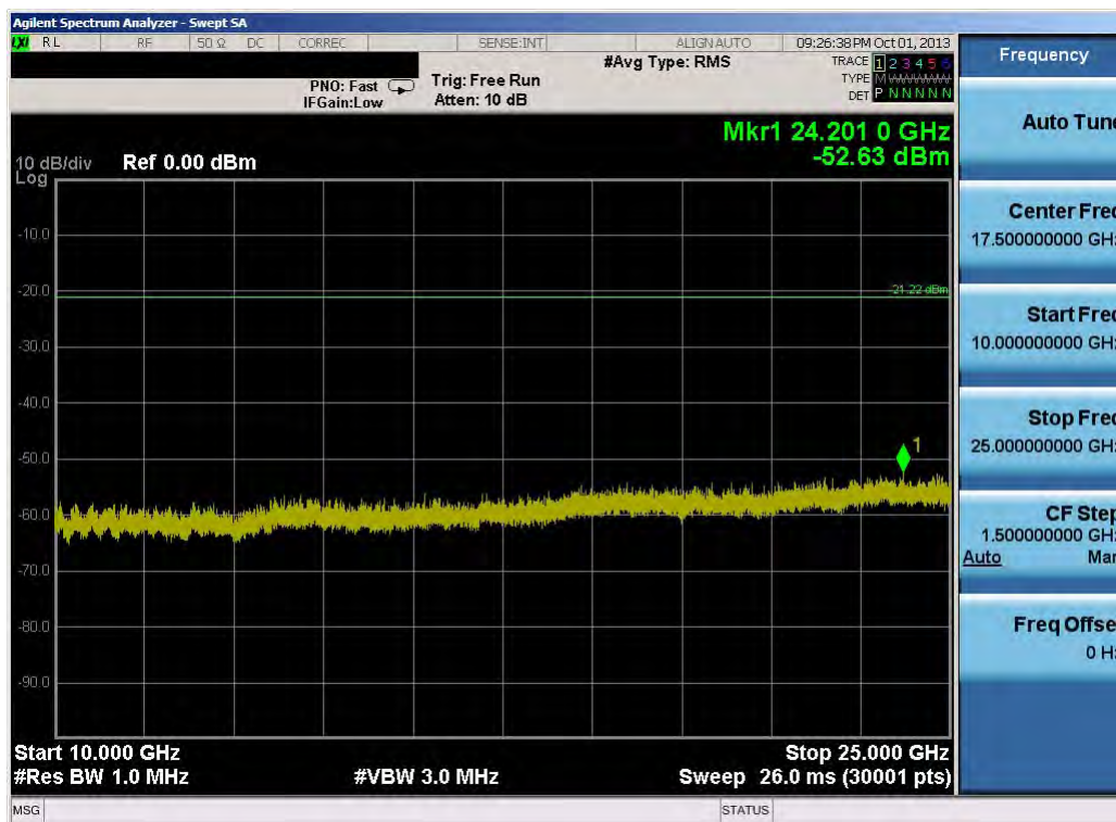
Plot 6-54. Conducted Spurious Plot (802.11b – Ch. 6)
