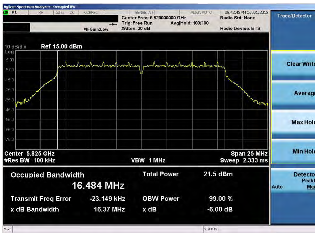
Plot 6-12. 6dB Bandwidth Plot (802.11a – Ch. 165)
