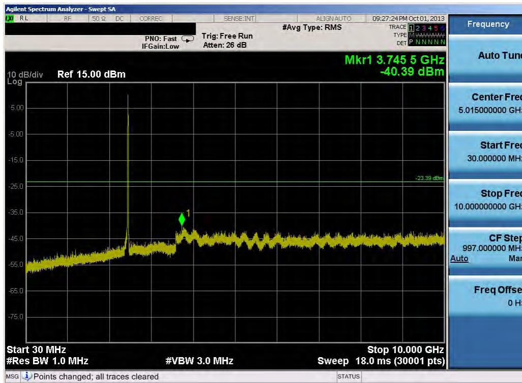
Plot 6-55. Conducted Spurious Plot (802.11b – Ch. 11)
