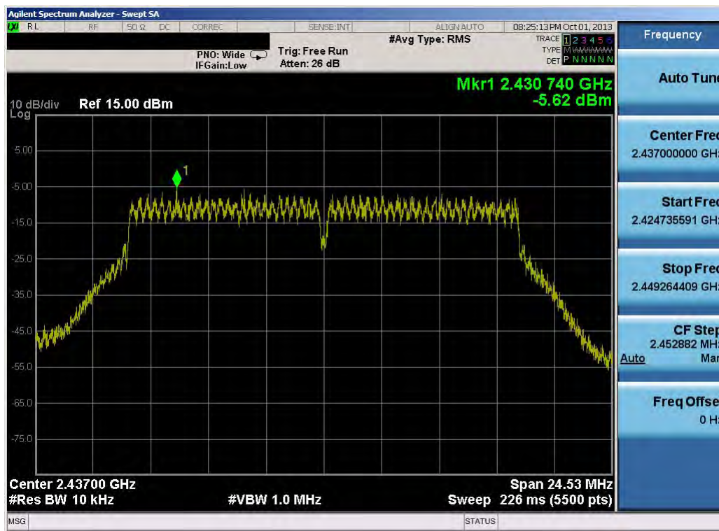
Plot 6-23. Power Spectral Density Plot (802.11g – Ch. 6)
