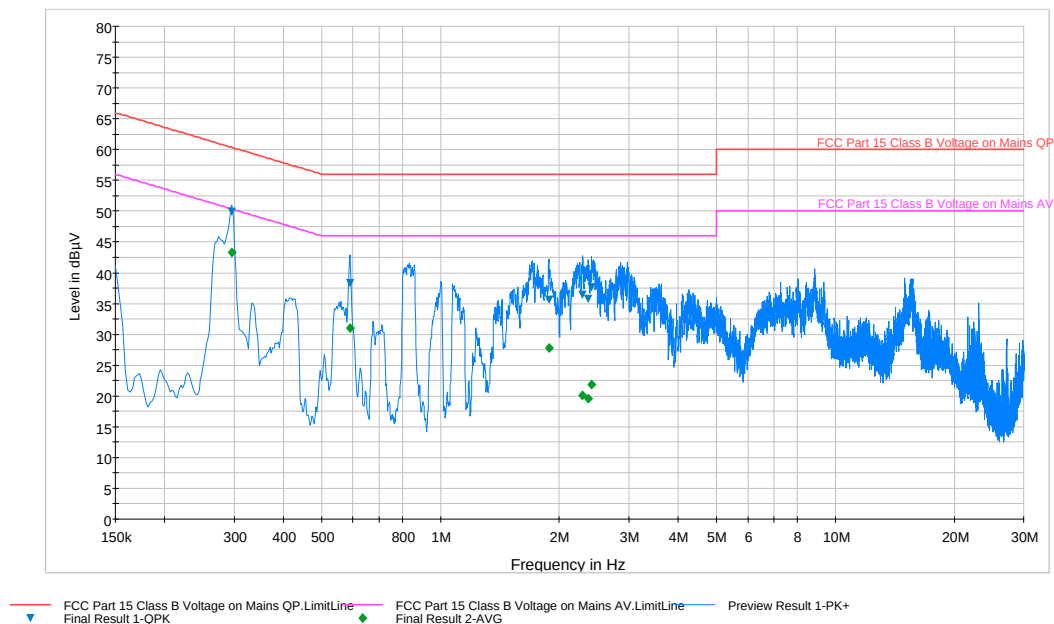
Plot 6-68. Line Conducted Plot with 802.11b (N)
