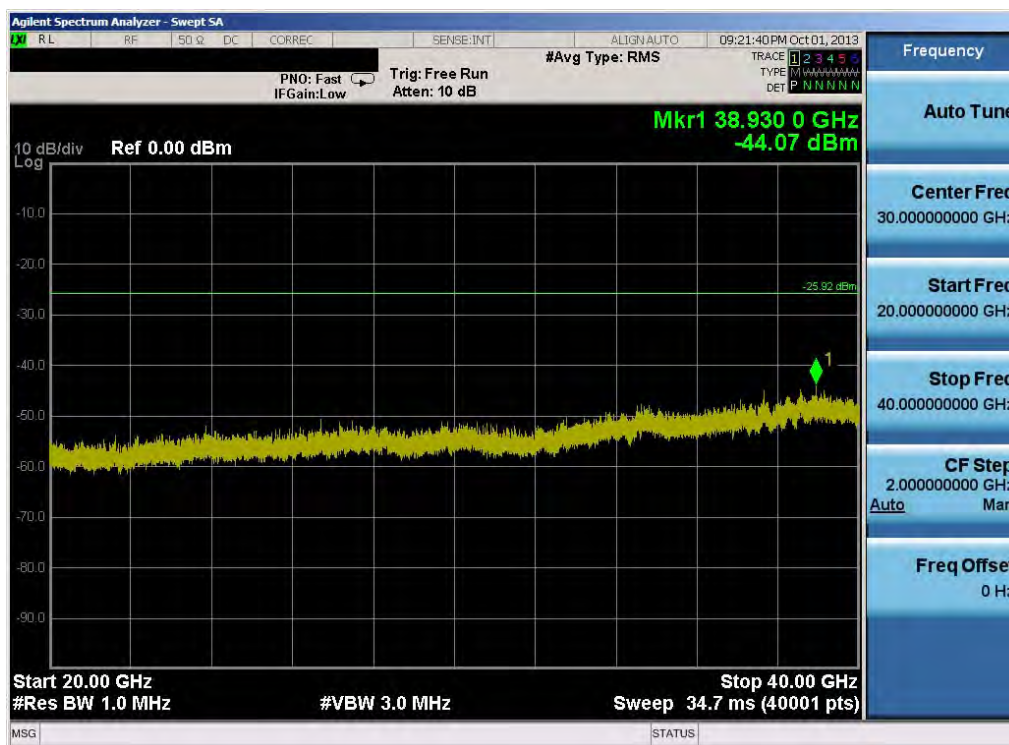
Plot 6-58. Conducted Spurious Plot (802.11a – Ch. 149)
