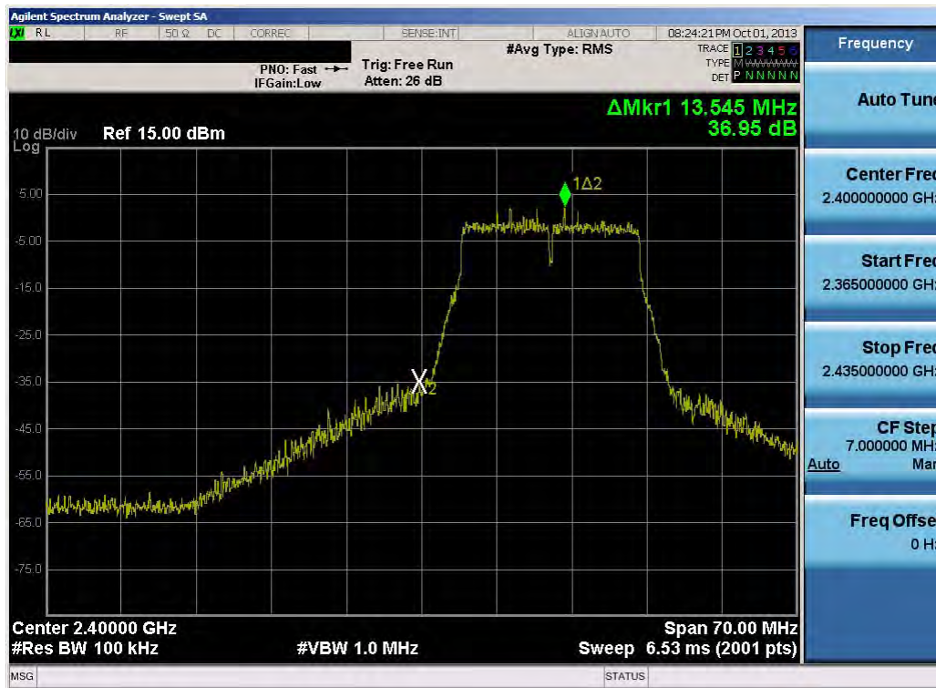
Plot 6-39. Band Edge Plot (802.11g- Ch. 1)
