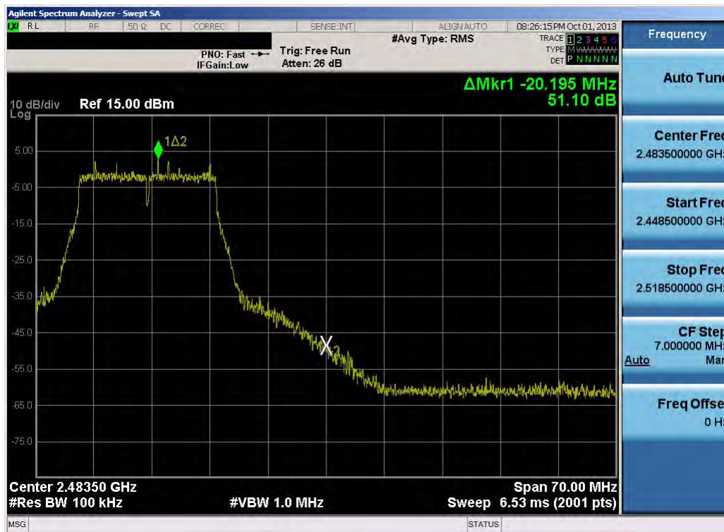
Plot 6-40. Band Edge Plot (802.11g - Ch. 11)
