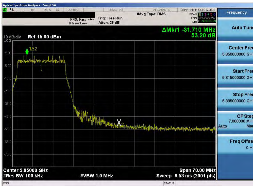
Plot 6-44. Band Edge Plot (802.11a – Ch. 165)
