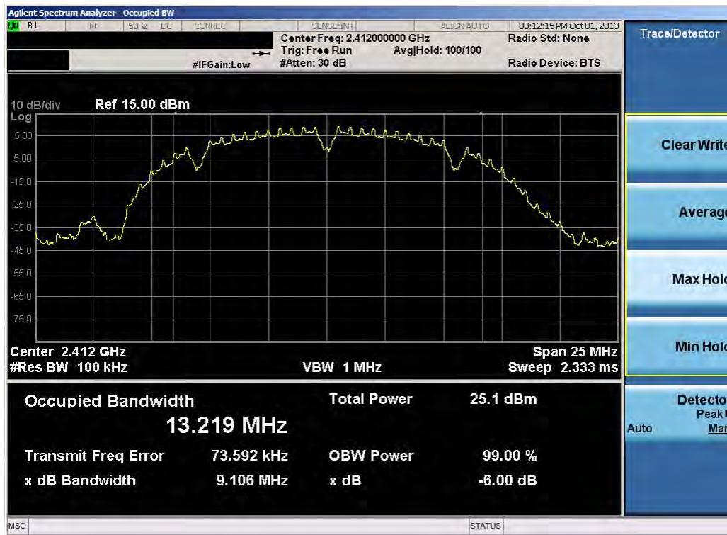
Plot 6-1. 6dB Bandwidth Plot (802.11b – Ch. 1)
