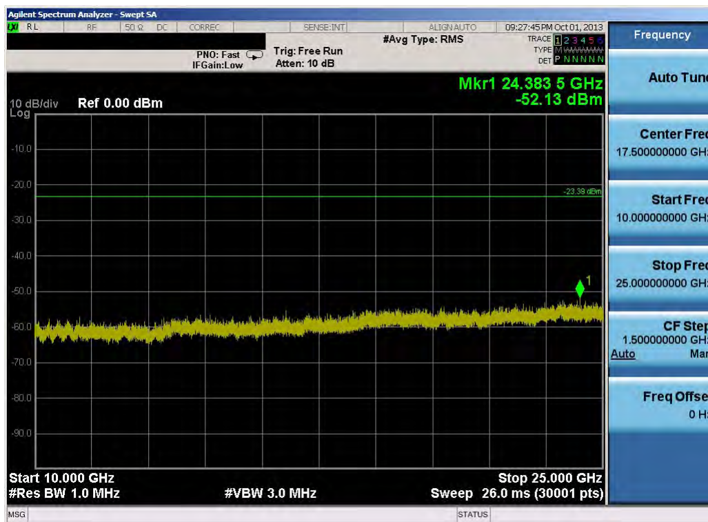
Plot 6-56. Conducted Spurious Plot (802.11b – Ch. 11)
