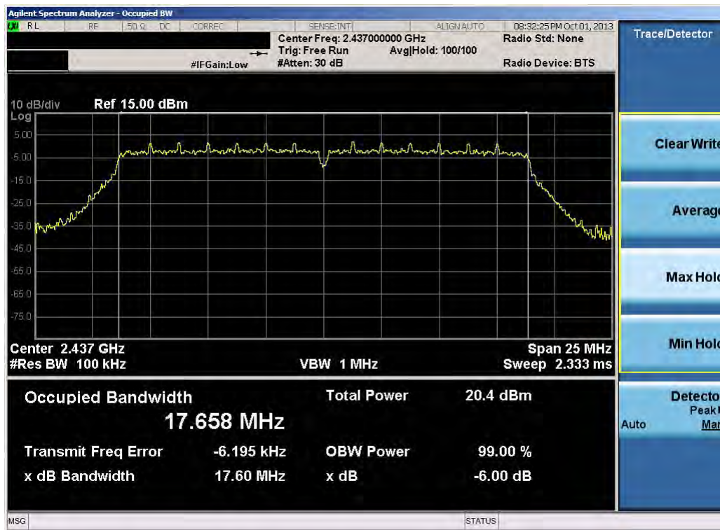
Plot 6-8. 6dB Bandwidth Plot (802.11n (2.4GHz) – Ch. 6)
