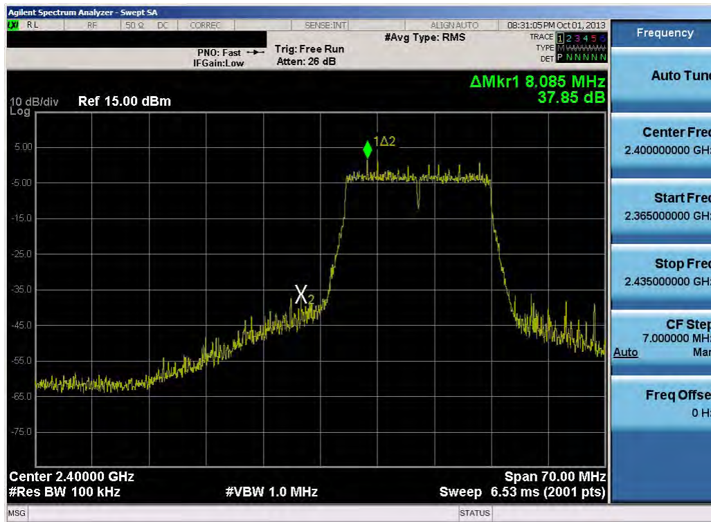
Plot 6-41. Band Edge Plot (802.11n (2.4GHz) – Ch. 1)
