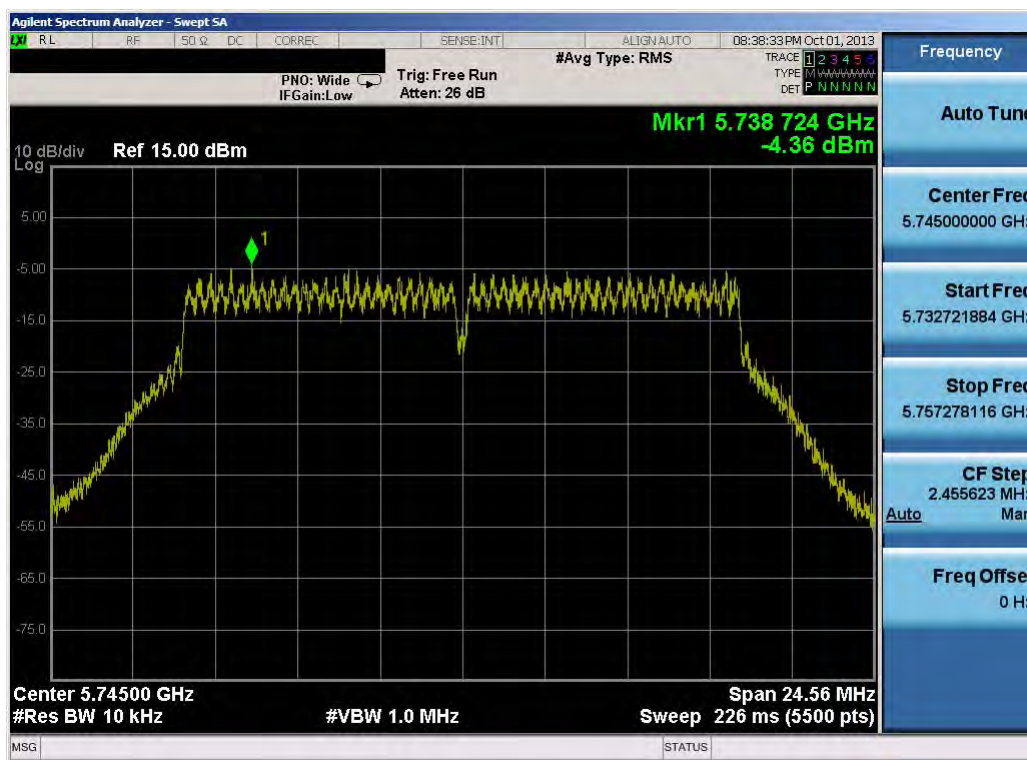
Plot 6-28. Power Spectral Density Plot (802.11a – Ch. 149)
