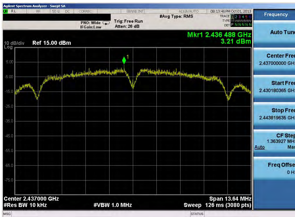
Plot 6-20. Power Spectral Density Plot (802.11b – Ch. 6)
