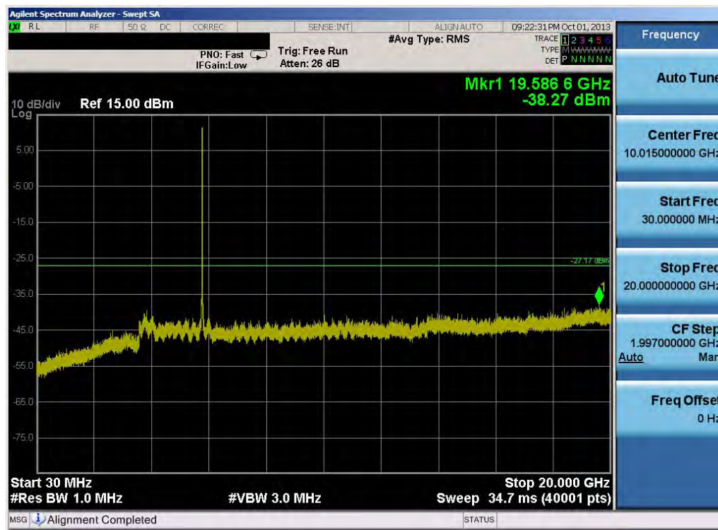
Plot 6-59. Conducted Spurious Plot (802.11a – Ch. 157)
