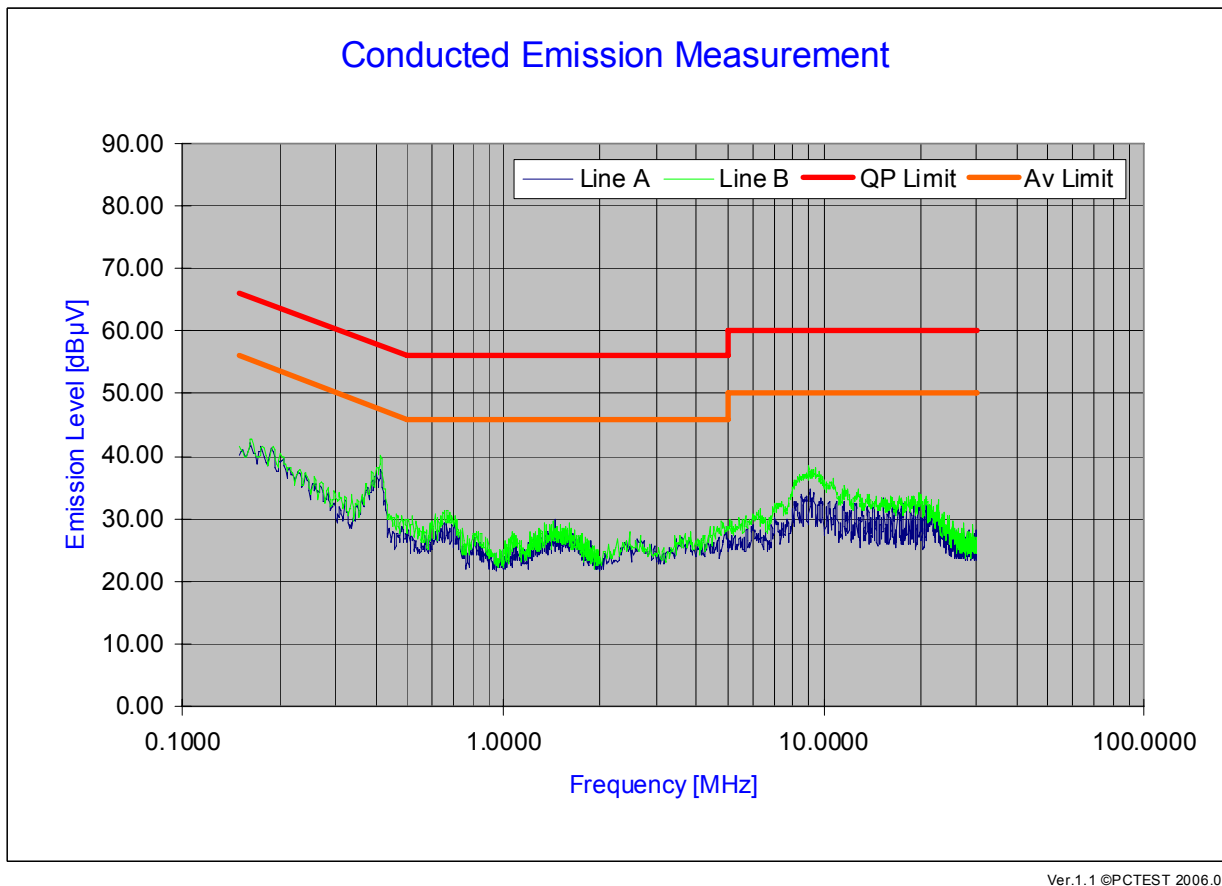
lot 6-18. Line Conducted Plot with Bluetooth
