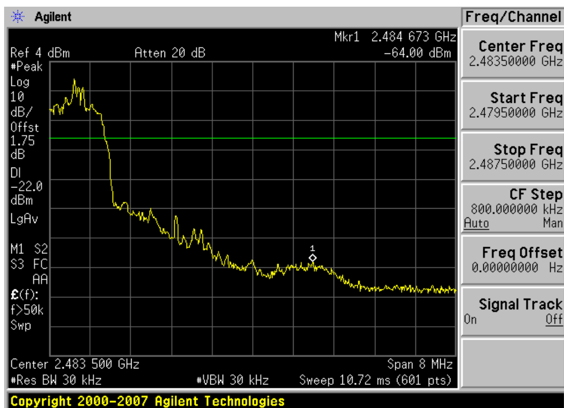
Plot 6-7. Band Edge Plot (Bluetooth 2.1 with Enhanced Data Rates – Ch. 78)
