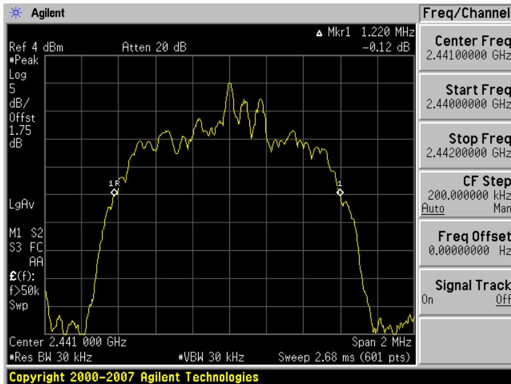
Plot 6-2. 20dB Bandwidth Plot (Bluetooth 2.1 with Enhanced Data Rates – Ch. 39)
