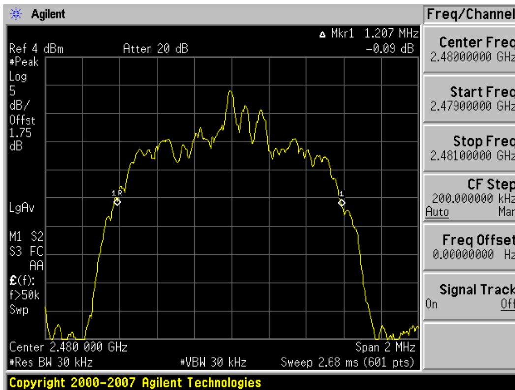
Plot 6-3. 20dB Bandwidth Plot (Bluetooth 2.1 with Enhanced Data Rates – Ch. 78)
