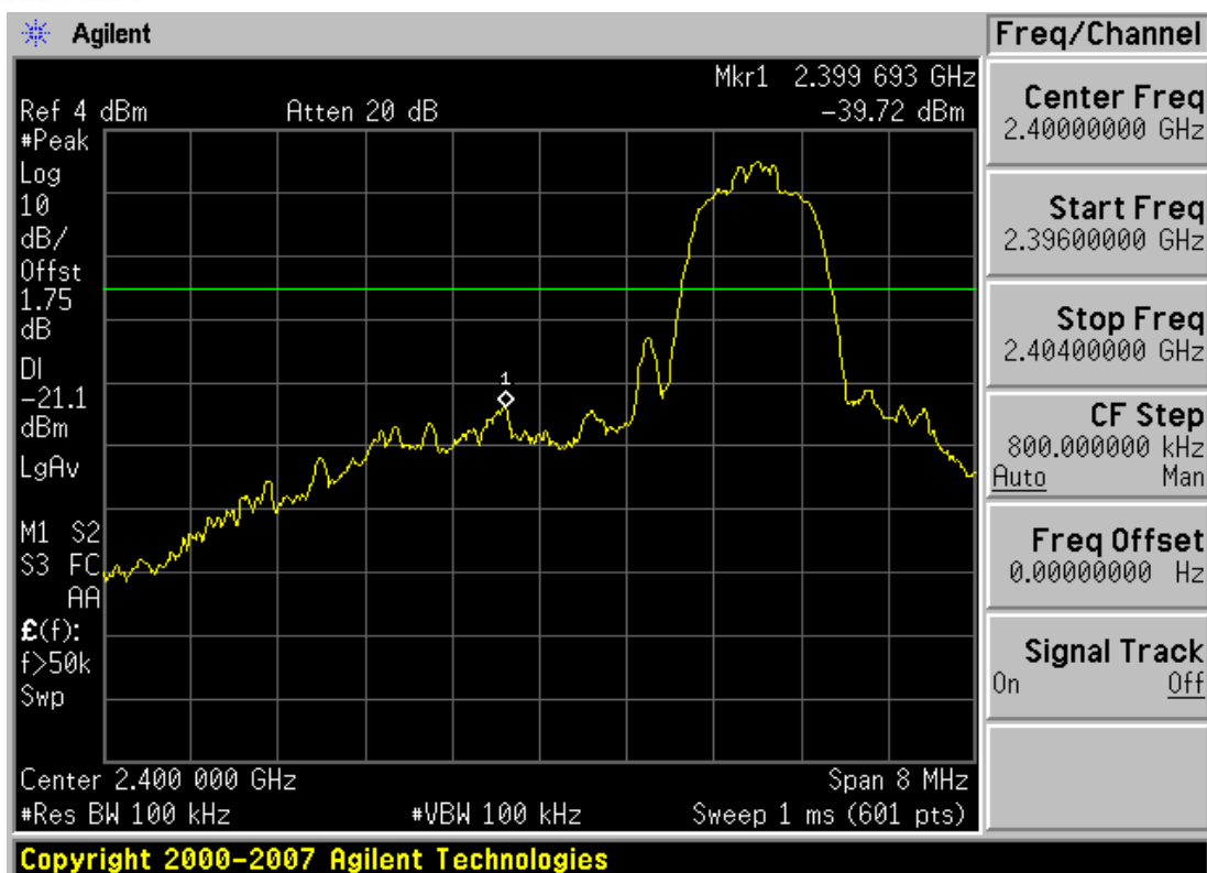
Plot 6-6. Band Edge Plot (Bluetooth 2.1 with Enhanced Data Rates – Ch. 0)
