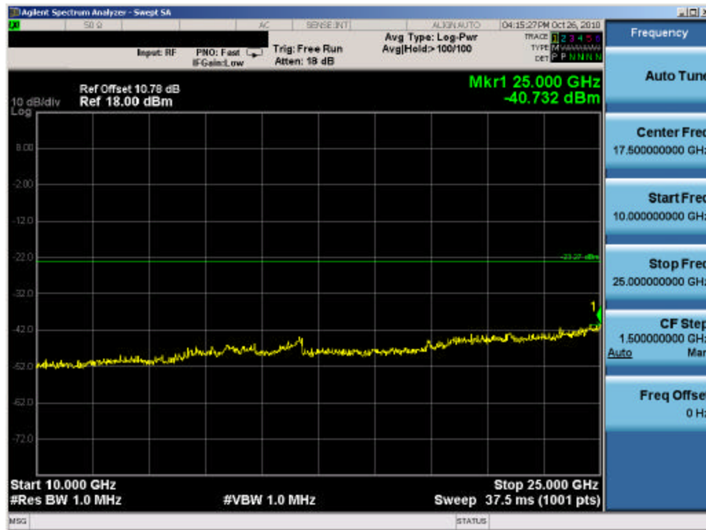
Plot 6-18. Conducted Spurious Plot (802.11b – Ch. 1)
