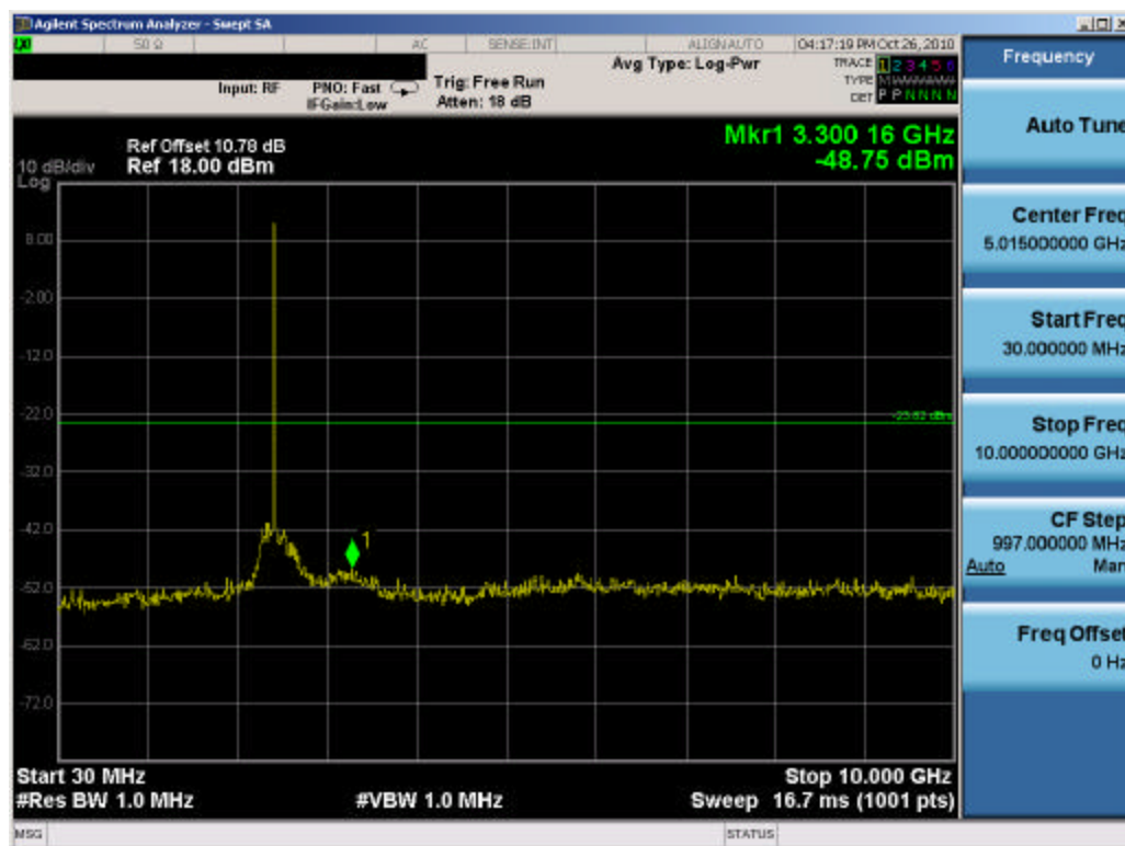
Plot 6-19. Conducted Spurious Plot (802.11b – Ch. 6)
