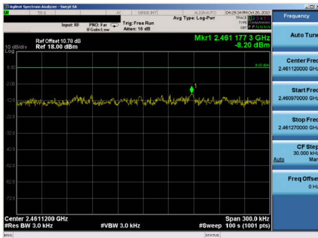
Plot 6-9. Power Spectral Density Plot (802.11b – Ch. 11)
