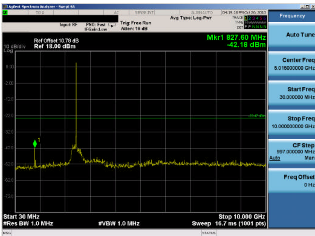
Plot 6-21. Conducted Spurious Plot (802.11b – Ch. 11)
