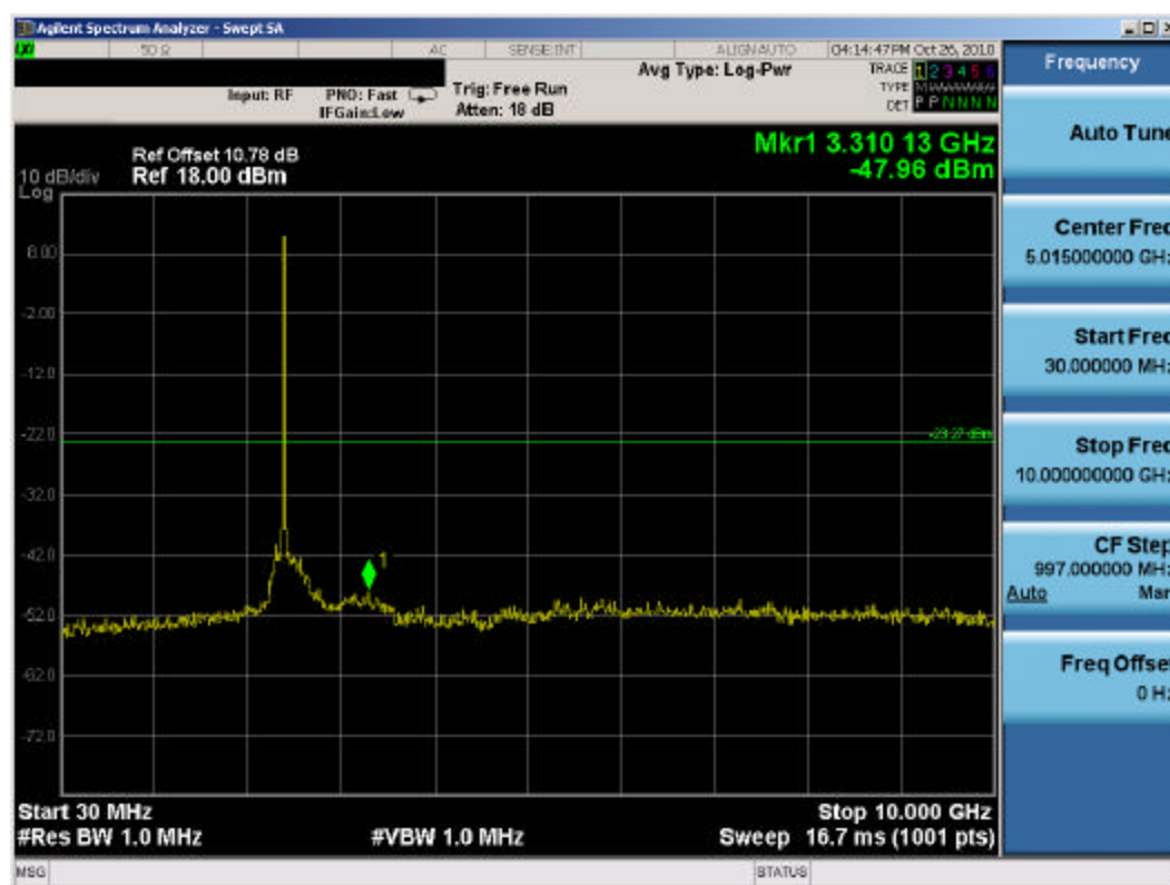
Plot 6-17. Conducted Spurious Plot (802.11b – Ch. 1)
