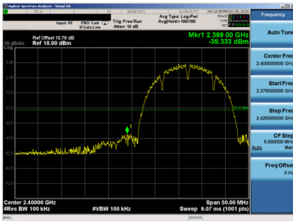
Plot 6-13. Band Edge Plot (802.11b – Ch. 1)
