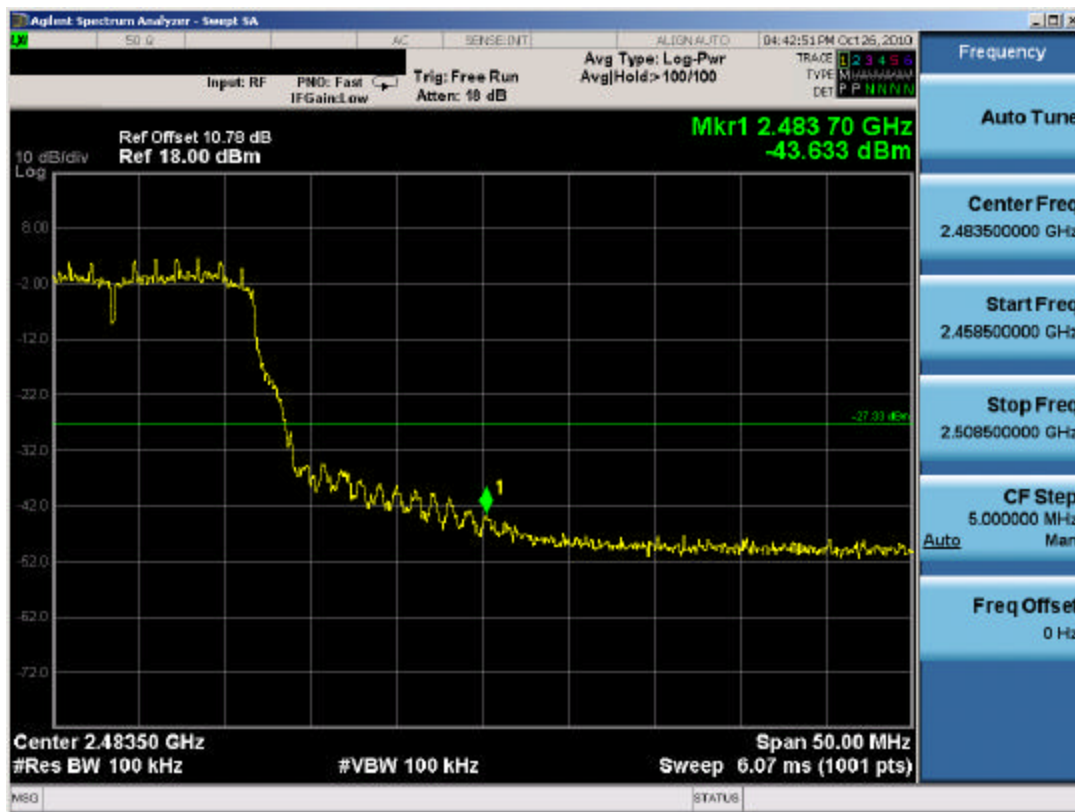
Plot 6-16. Band Edge Plot (802.11g – Ch. 11)
