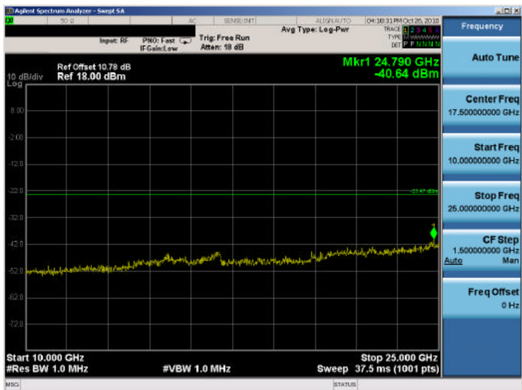
Plot 6-22. Conducted Spurious Plot (802.11b – Ch. 11)
