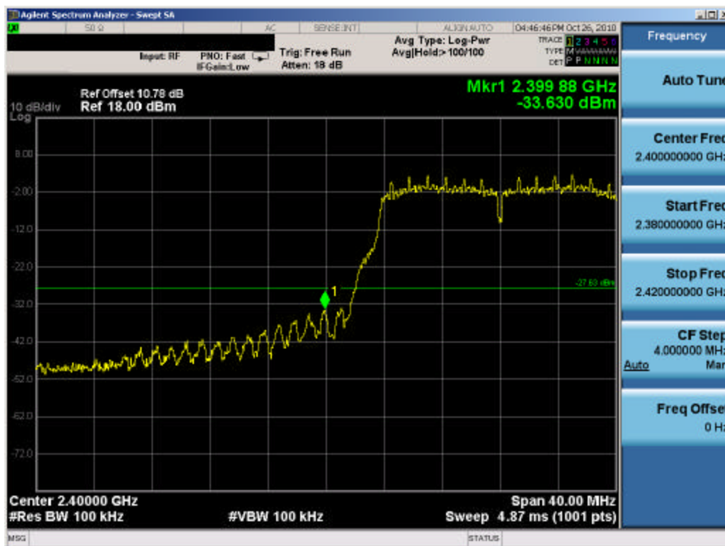
Plot 6-15. Band Edge Plot (802.11g – Ch. 1)
