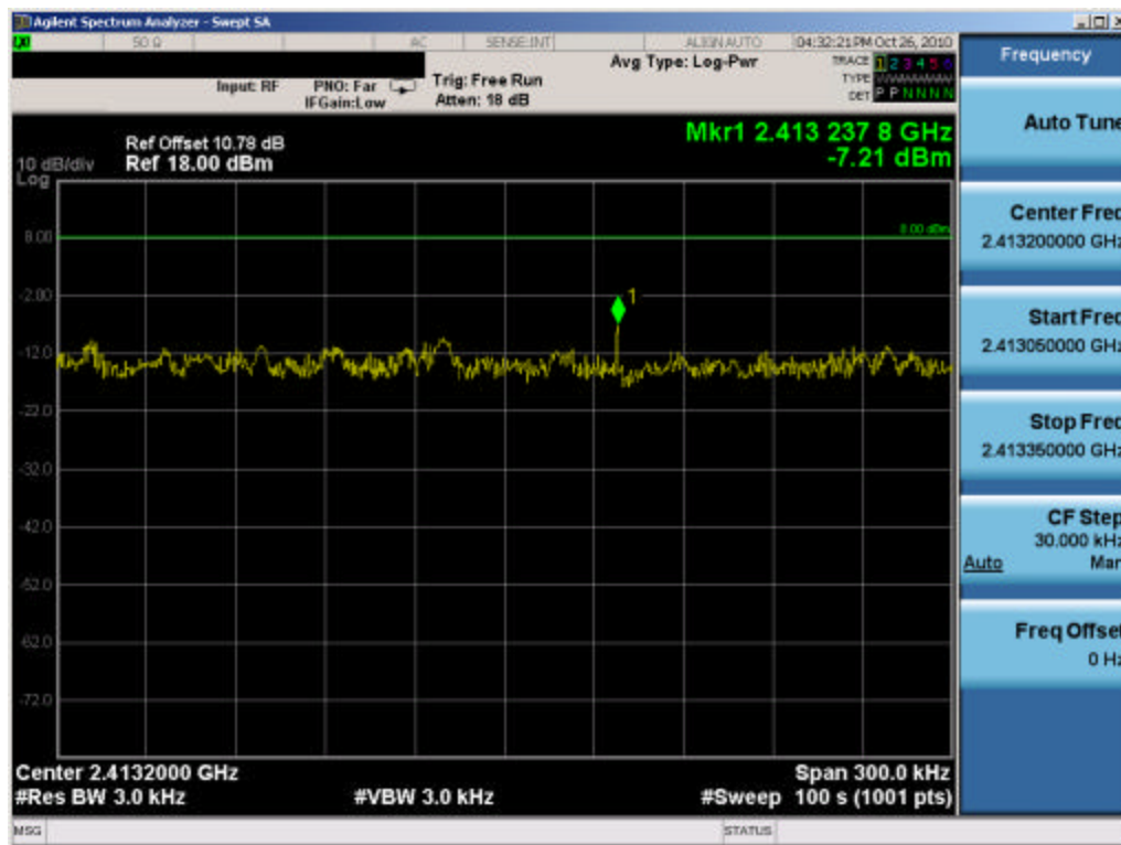
Plot 6-7. Power Spectral Density Plot (802.11b – Ch. 1)
