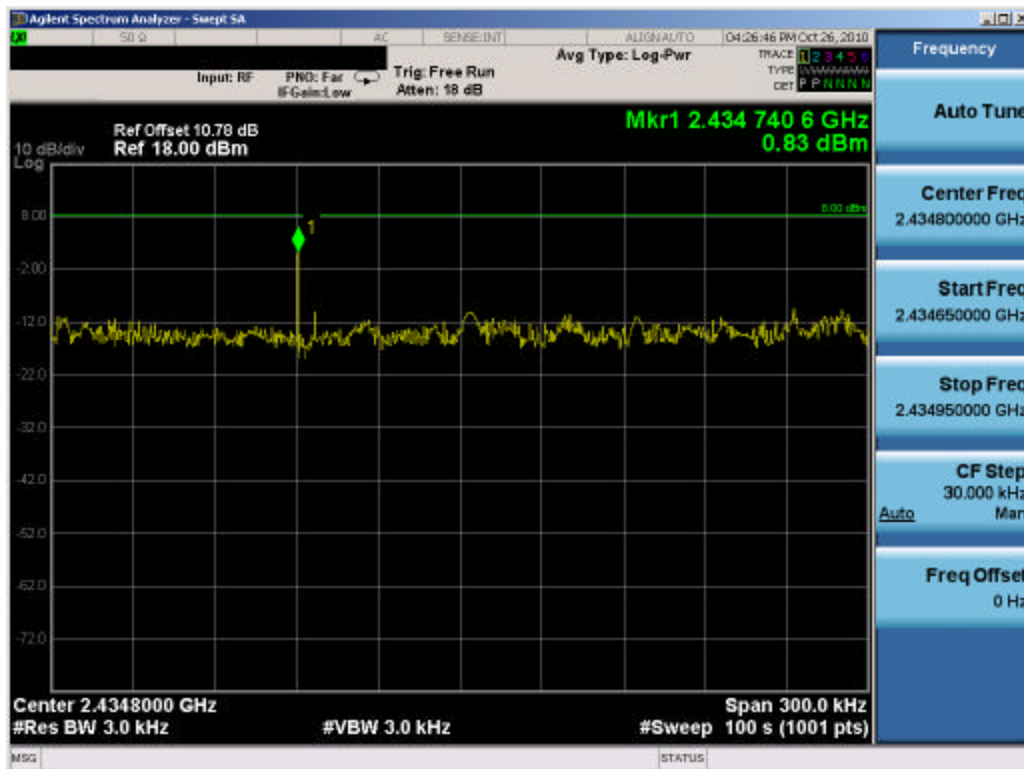
Plot 6-8. Power Spectral Density Plot (802.11b – Ch. 6)
