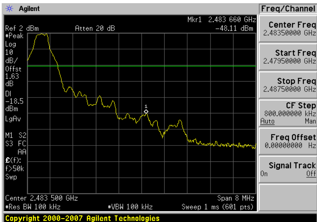
Plot 6-8. Band Edge Plot (Bluetooth, 1Mbps - Ch. 78)
