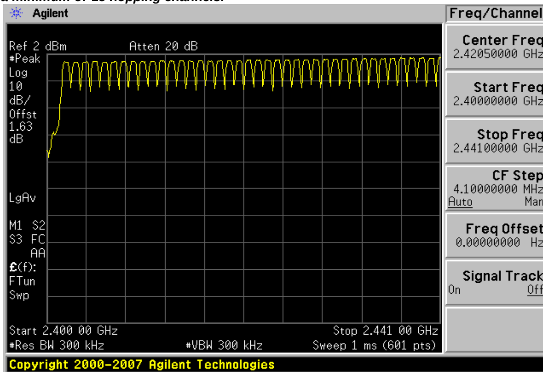
Plot 6-13. Low End Spectrum Channel Hopping Plot (Bluetooth)
