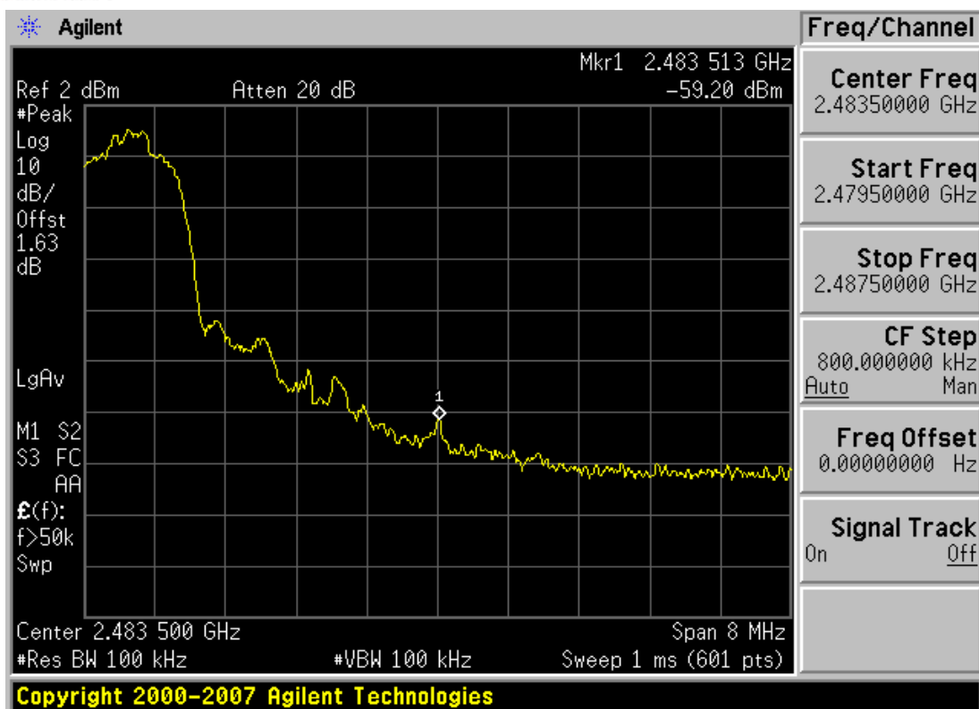
Plot 6-10. Band Edge Plot (Bluetooth, 2Mbps - Ch. 78)
