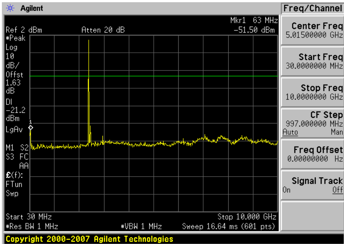
Plot 6-15. Conducted Spurious Plot (Bluetooth, 1Mbps – Ch. 0)
