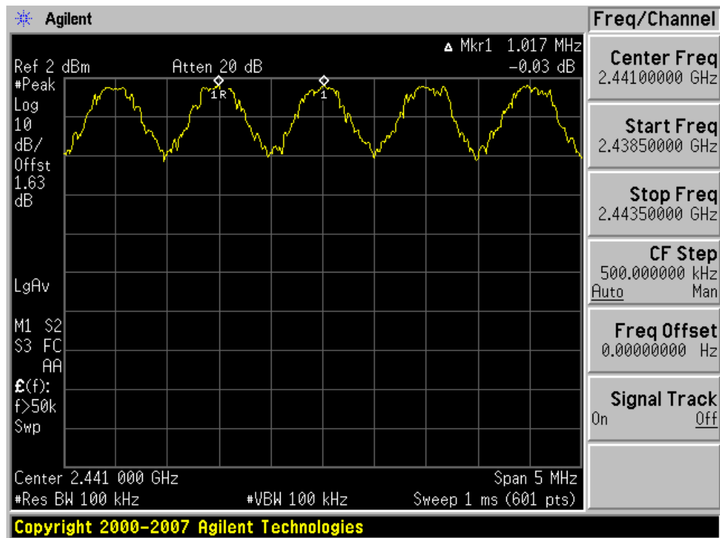
Plot 6-11. Channel Spacing Plot (Bluetooth)
