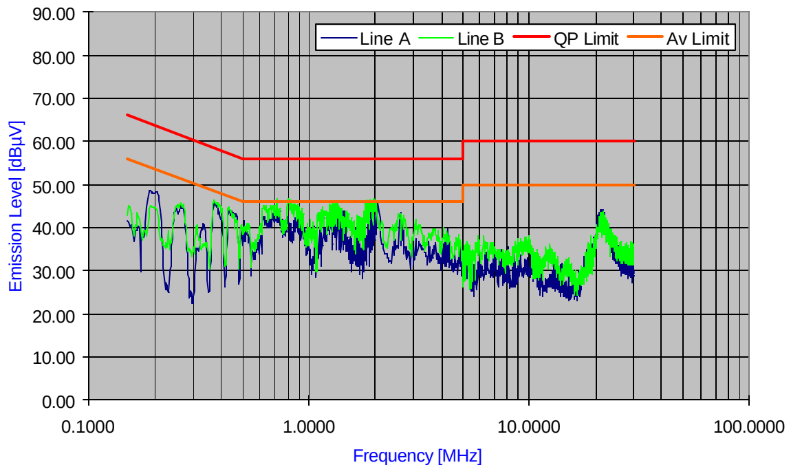
Plot 6-21. Line Conducted Plot with Bluetooth
