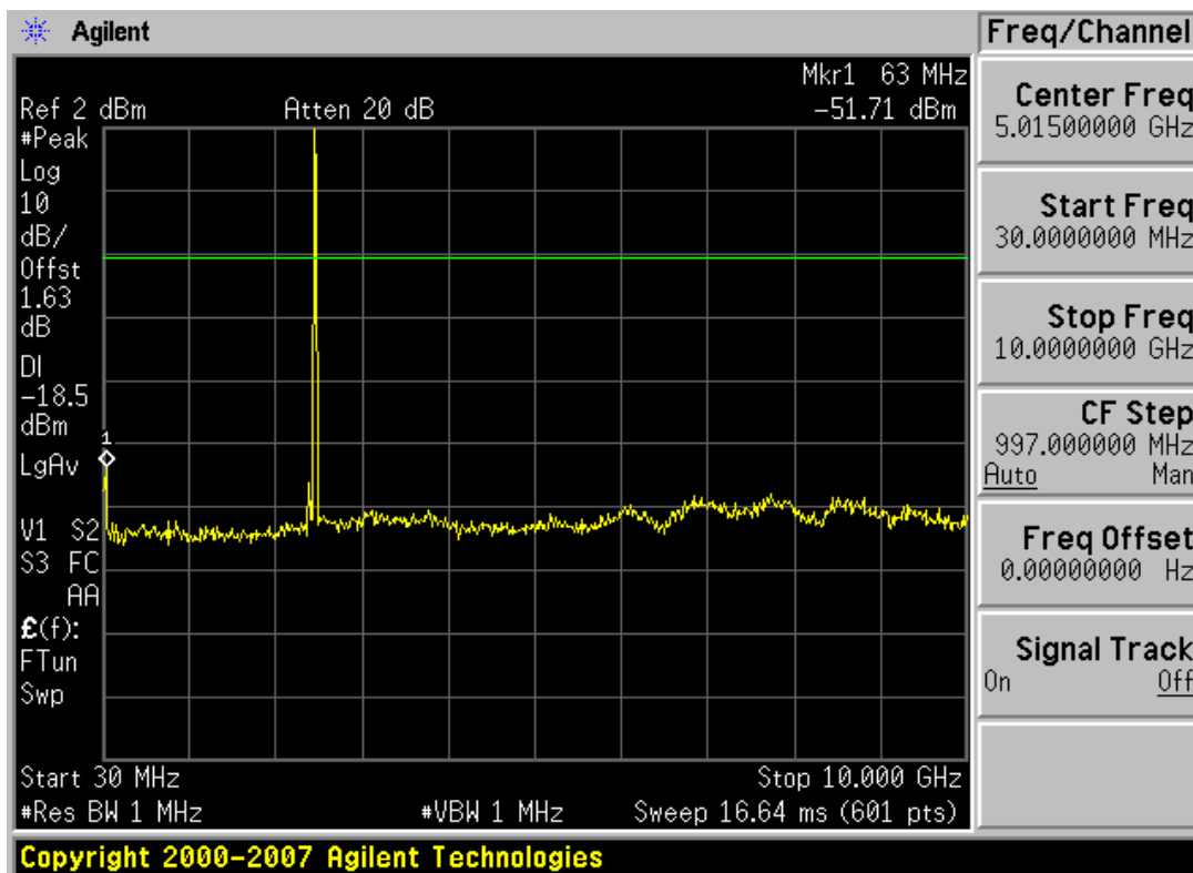
Plot 6-19. Conducted Spurious Plot (Bluetooth, 1Mbps – Ch. 78)
