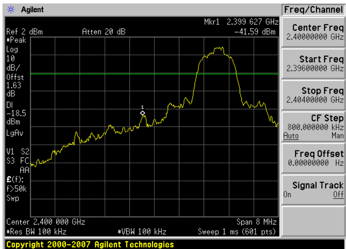
Plot 6-9. Band Edge Plot (Bluetooth, 2Mbps - Ch. 0)
