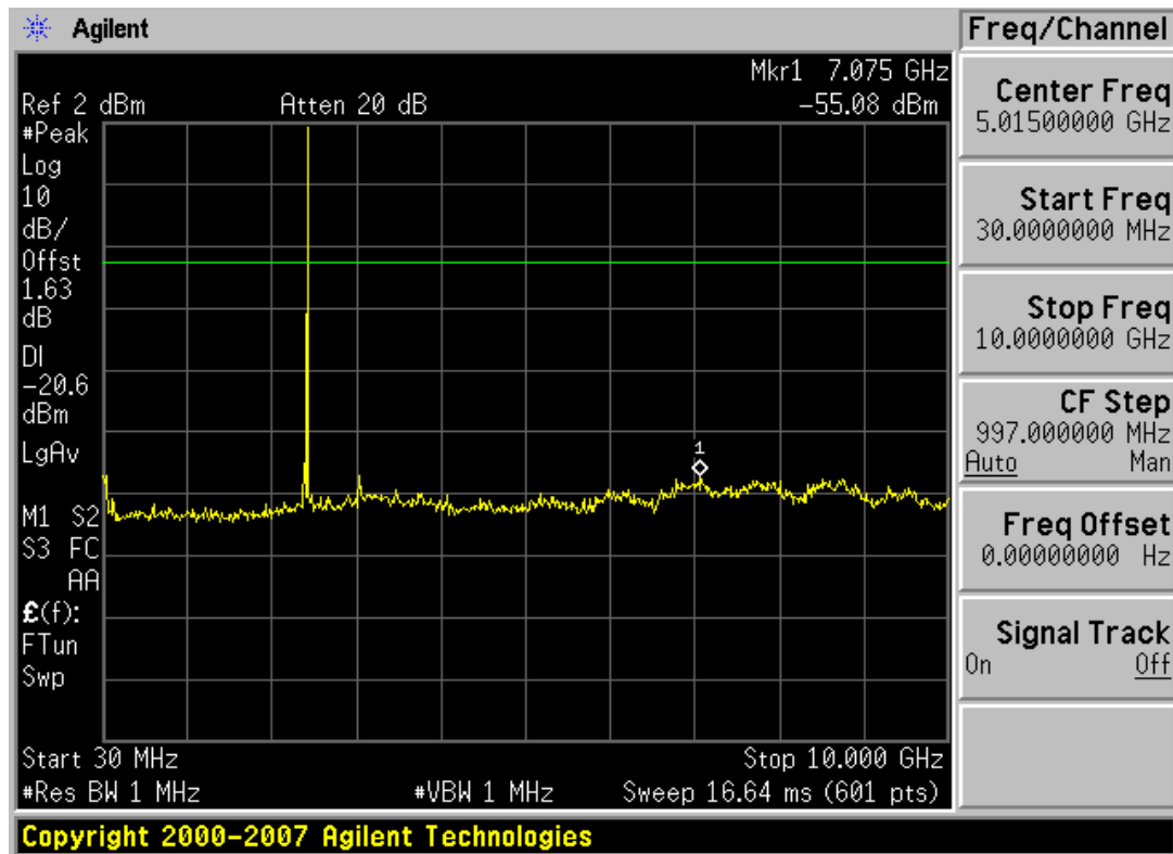
Plot 6-17. Conducted Spurious Plot (Bluetooth, 1Mbps – Ch. 39)
