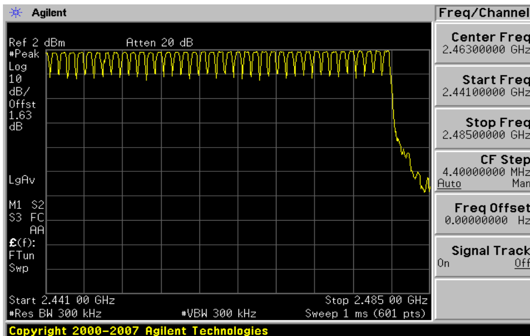
Plot 6-14. High End Spectrum Channel Hopping Plot (Bluetooth)
