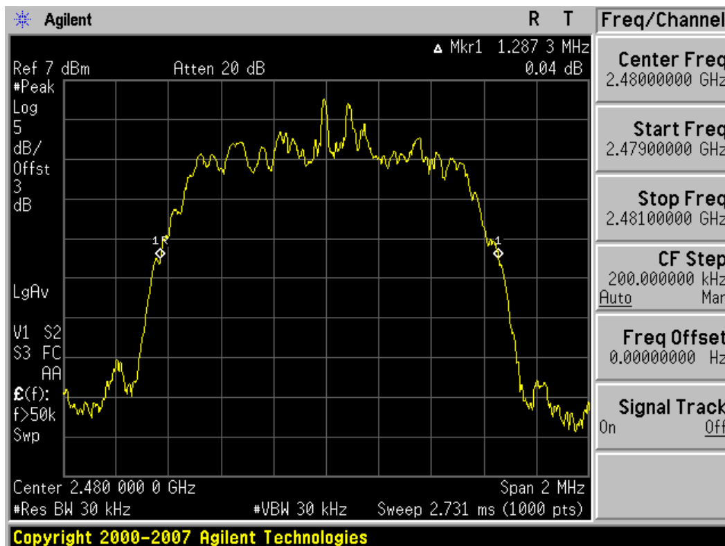
Plot 6-3. 20dB Bandwidth Plot (Bluetooth with EDR – Ch. 78)
