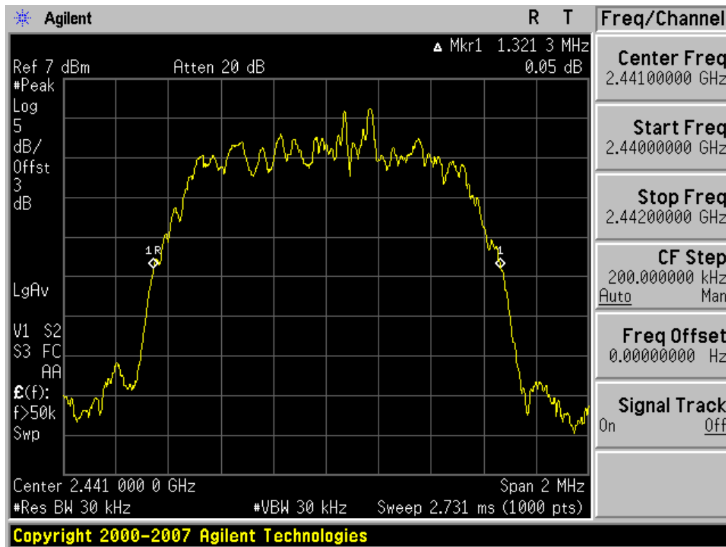
Plot 6-2. 20dB Bandwidth Plot (Bluetooth with EDR – Ch. 39)
