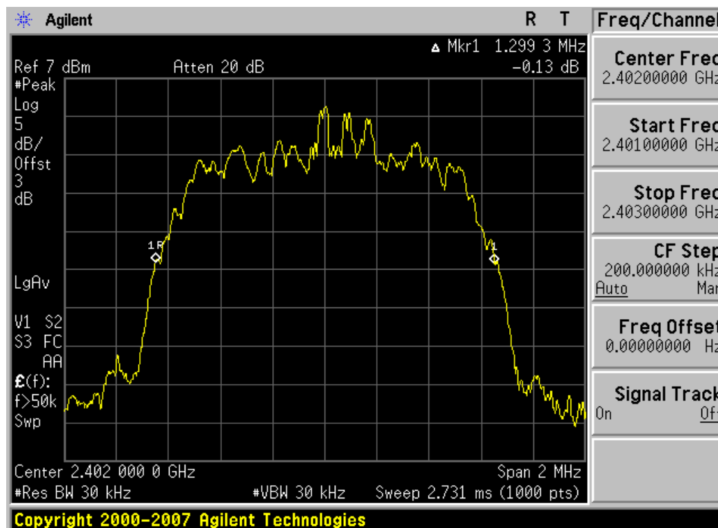
Plot 6-1. 20dB Bandwidth Plot (Bluetooth with EDR – Ch. 0)
