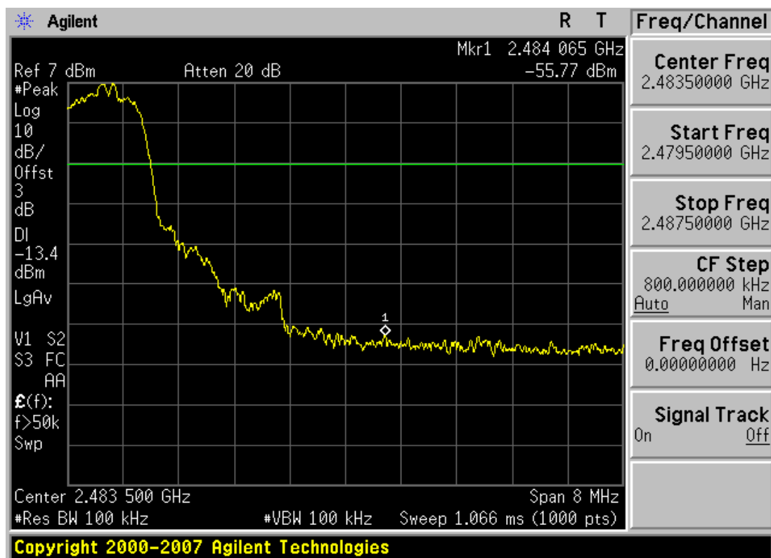
Plot 6-7. Band Edge Plot (Bluetooth with EDR – Ch. 78)
