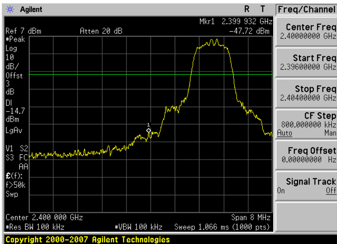
Plot 6-6. Band Edge Plot (Bluetooth with EDR – Ch. 0)
