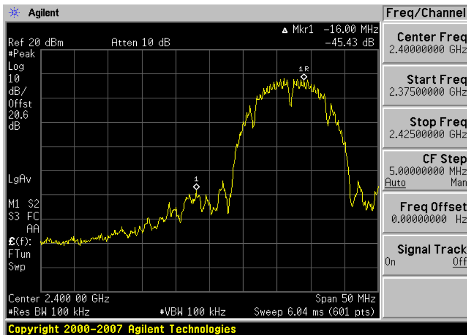
Plot 6-7. Band Edge Plot (802.11b – Ch. 1)
