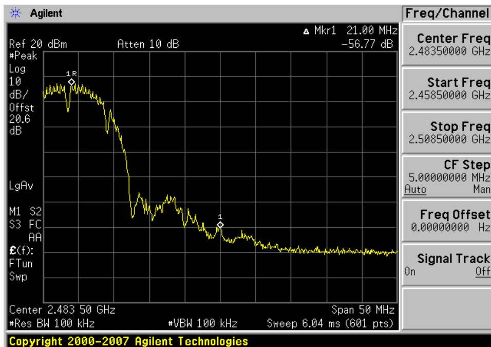
Plot 6-8. Band Edge Plot (802.11b – Ch. 11)
