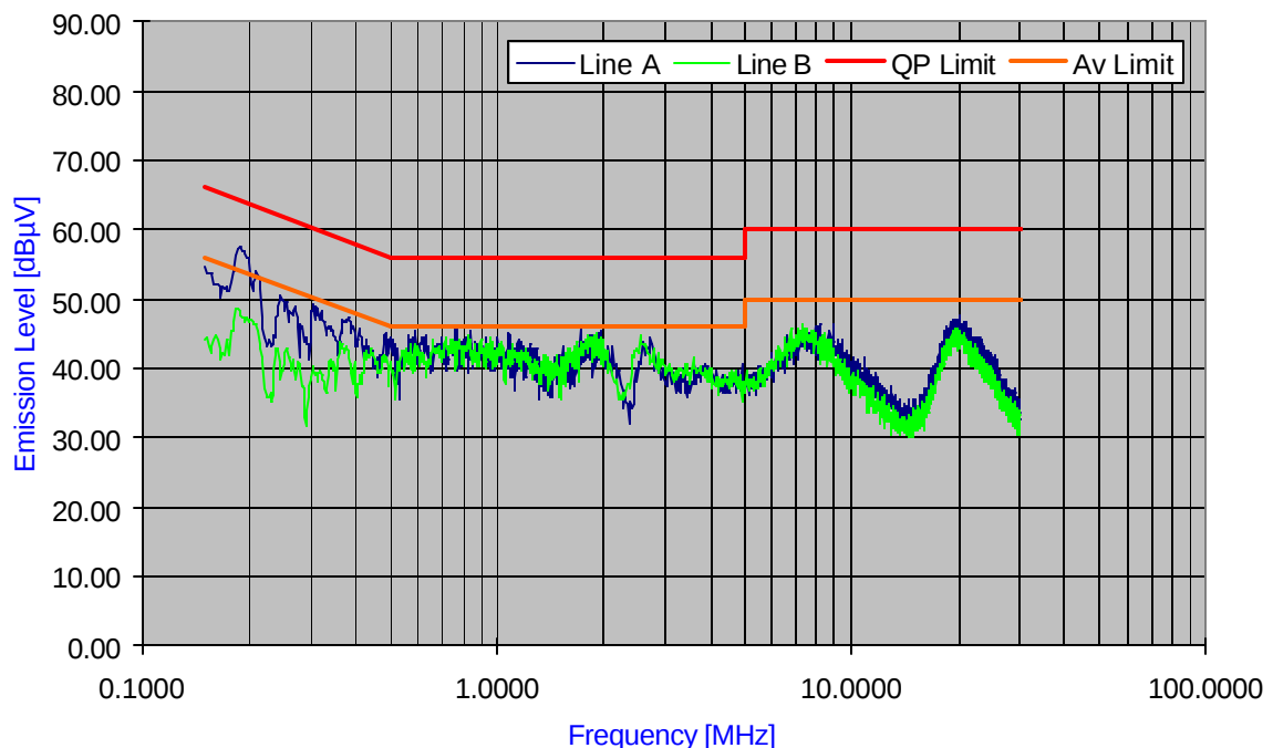
Plot 6-18. Line Conducted Plot with Bluetooth
