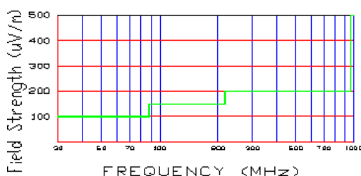
Figure 6-1. 3-Meter Limits
