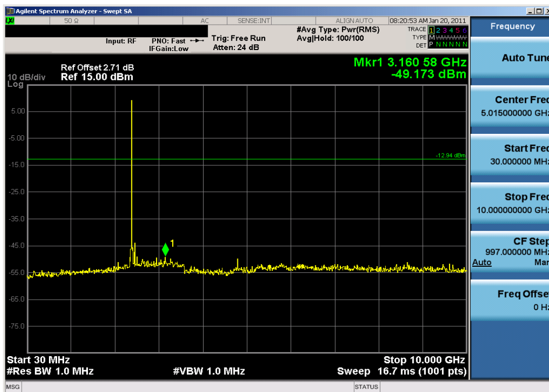
Plot 6-18. Conducted Spurious Plot (Bluetooth, 2Mbps – Ch. 0)
