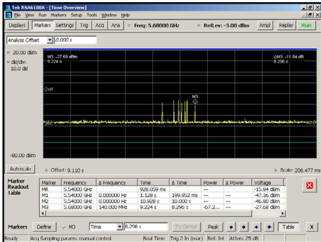
Figure 6-10. Pulse Grouping 5
