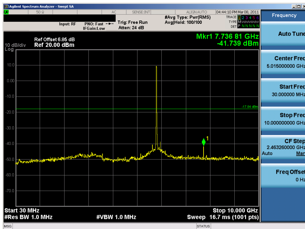
Plot 6-53. Conducted Spurious Plot (802.11a – Ch. 161)
