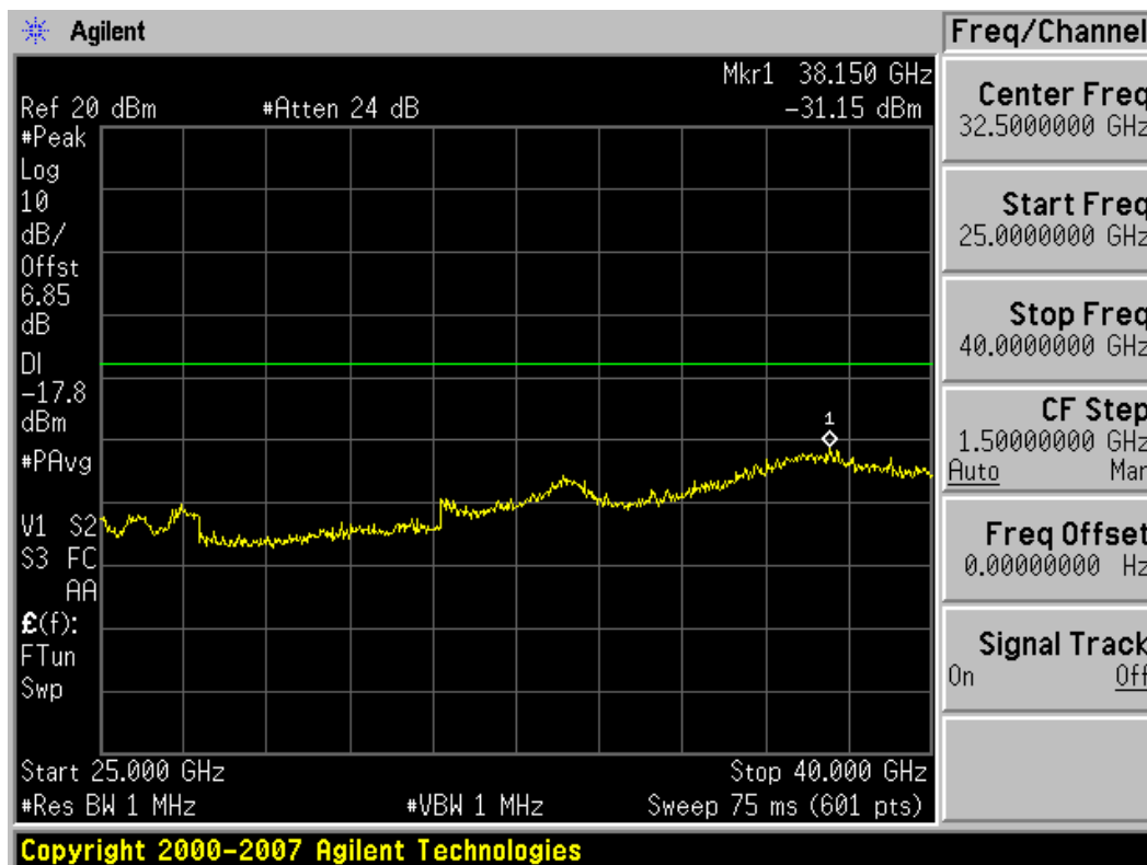
Plot 6-55. Conducted Spurious Plot (802.11a – Ch. 161)
