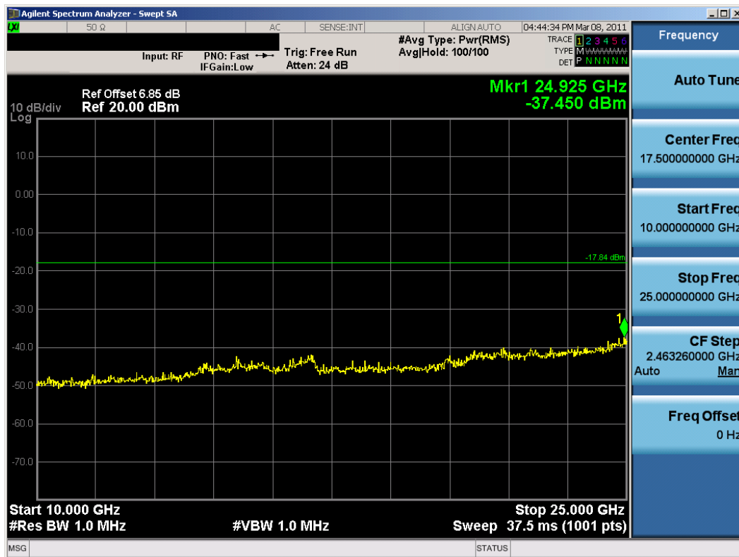
Plot 6-54. Conducted Spurious Plot (802.11a – Ch. 161)
