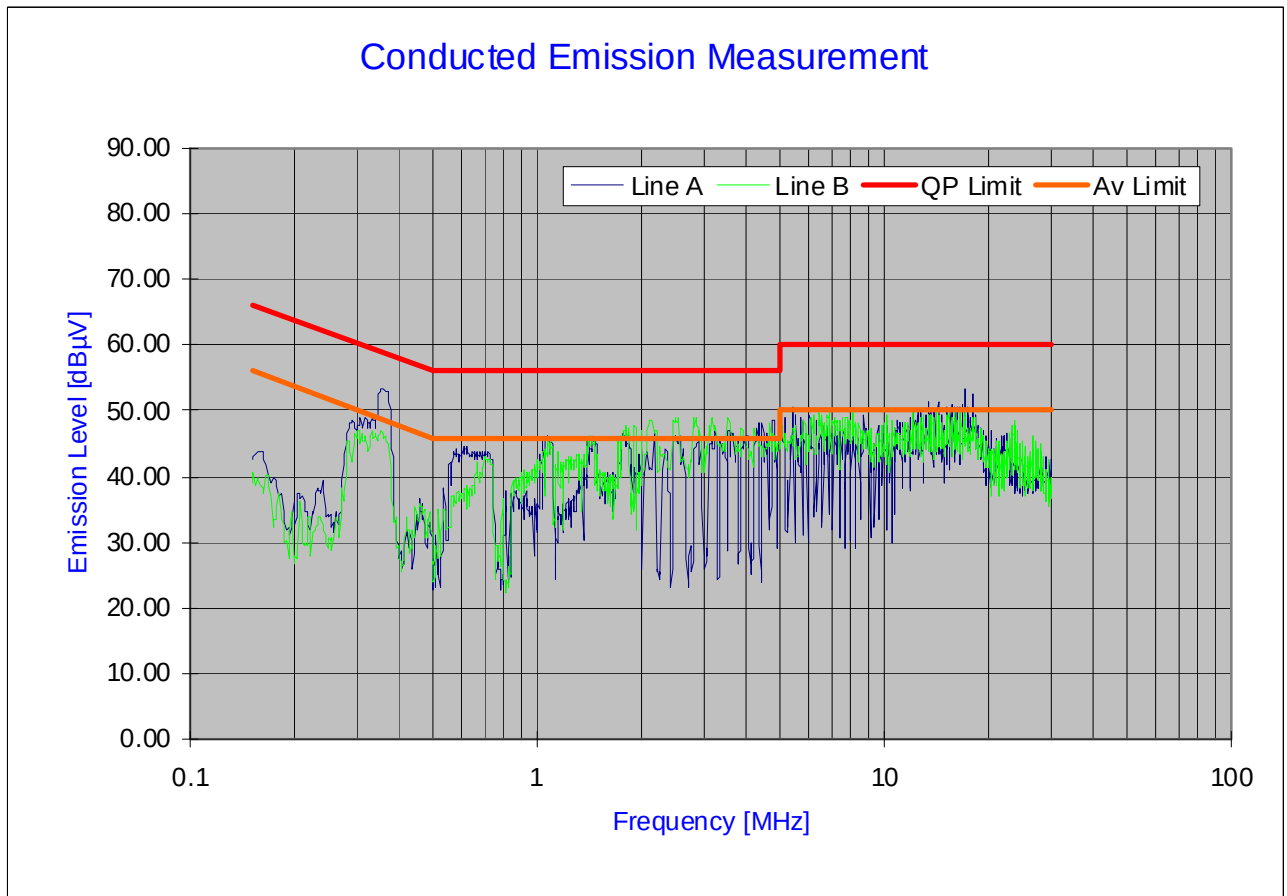
Plot 7-1. Line-Conducted Test Plot
