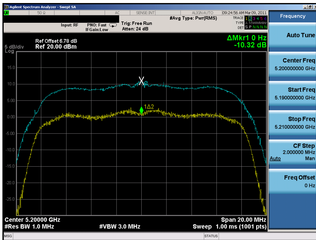
Plot 6-38. Peak Excursion Ratio Plot (802.11a (UNII) – Ch. 40)
