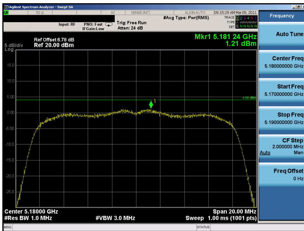
Plot 6-19. Peak Power Spectral Density Plot (802.11a (UNII) – Ch. 36)
