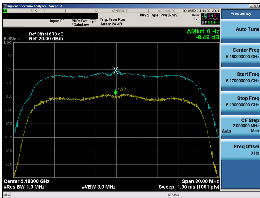
Plot 6-37. Peak Excursion Ratio Plot (802.11a (UNII) – Ch. 36)
