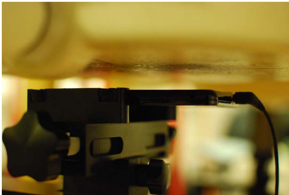
Figure 21-10 SAR Test Setup Photo 10 - Back at 1.5 cm
