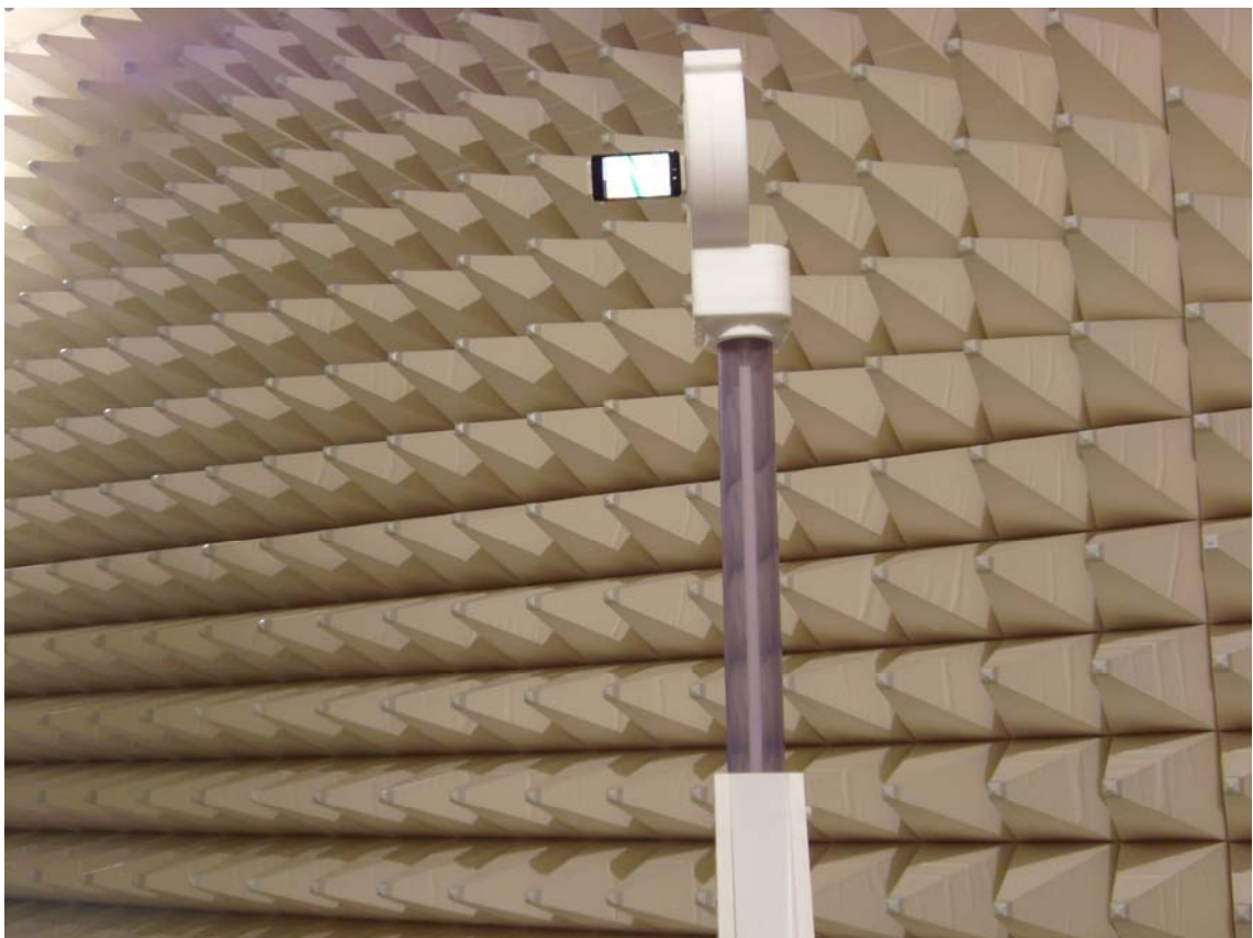
SAMSUNG FCC ID: A3LSHWM250S 1900 GSM/GPRS Phone with Bluetooth and WLAN
