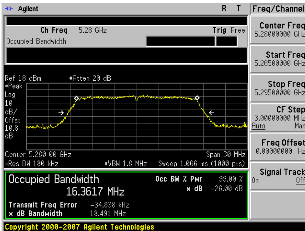
Plot 6-8. 26dB Bandwidth Plot (802.11a (UNII Band 2) – Ch. 56)
