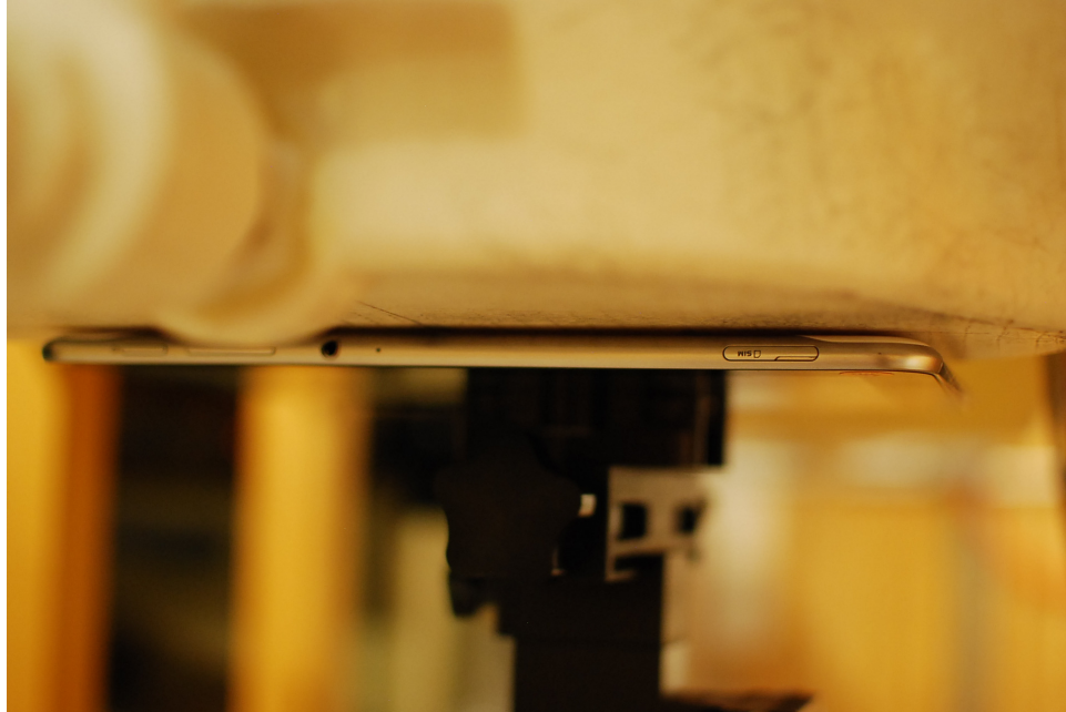
Figure 20-1 SAR Test Setup Photo 1 – Back at 0 cm
