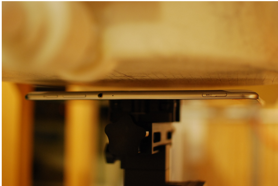
Figure 20-2 SAR Test Setup Photo 2 – Back at 1.0 cm
